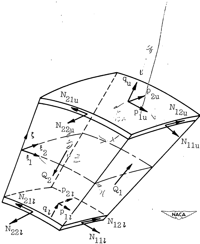
Figure 2.- Element of composite shell, showing location and orientation of stress resultants in face layers and core layer and orientation of external loads.
