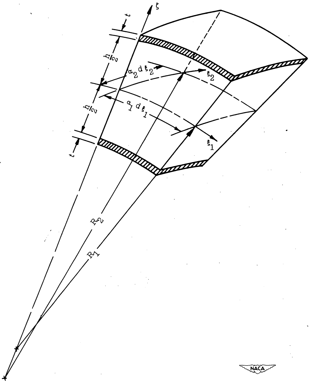
Figure 1.- Element of composite shell, showing coordinates and dimensions.
