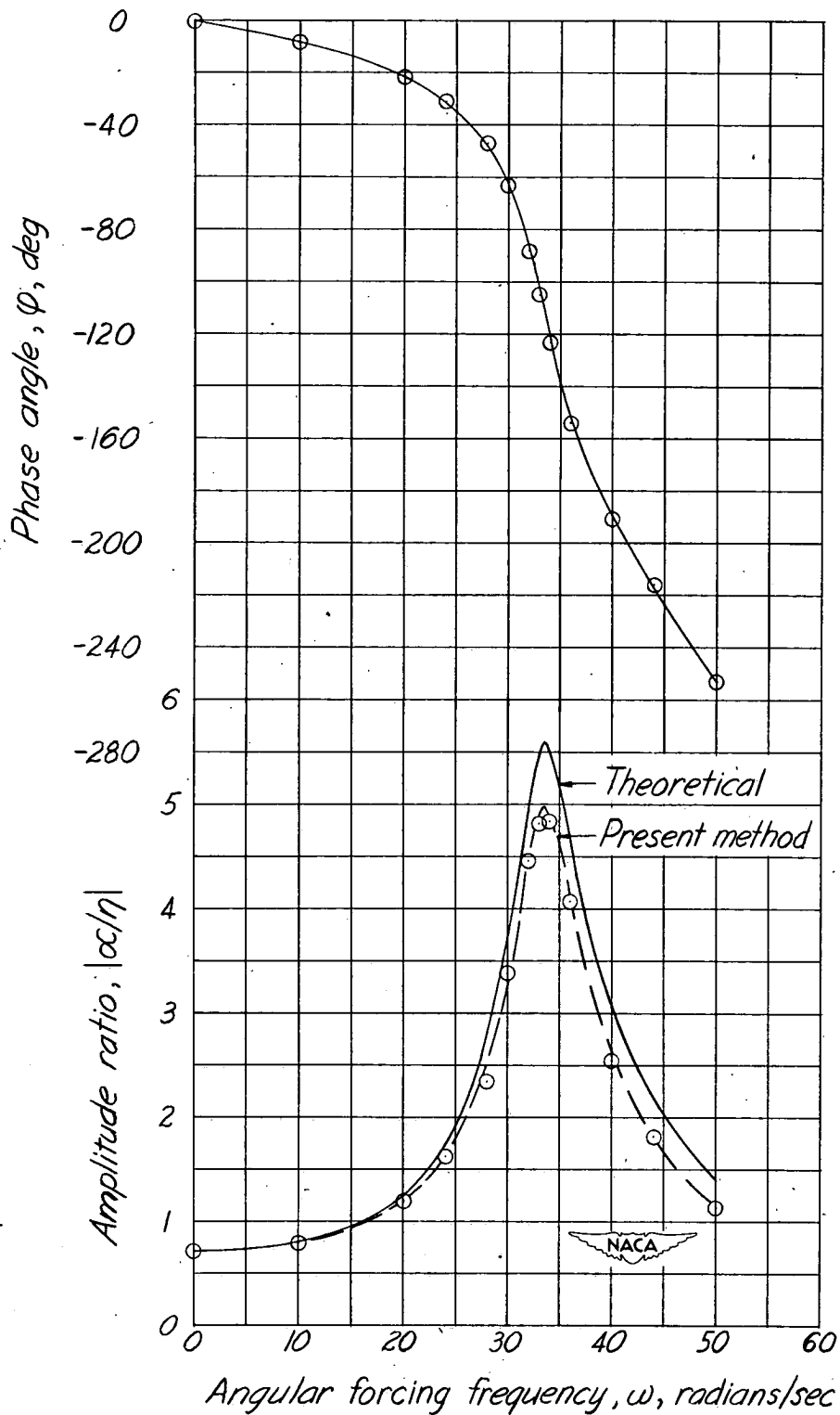
(b) Over-all frequency response, \alpha/\eta .
