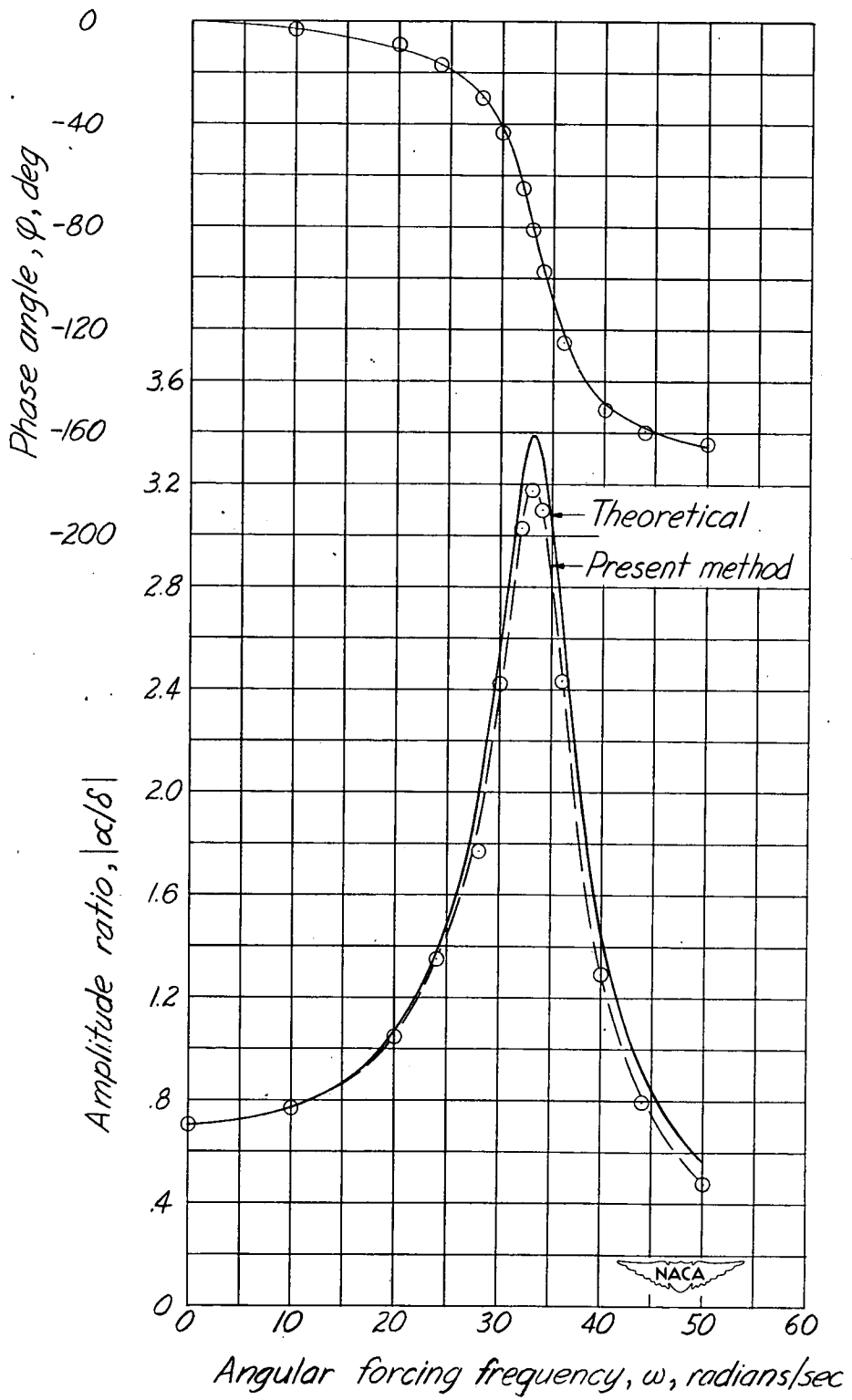
Figure 5.- Comparison of the theoretical response and the computed response determined from the computed frequency responses of figure 4.
