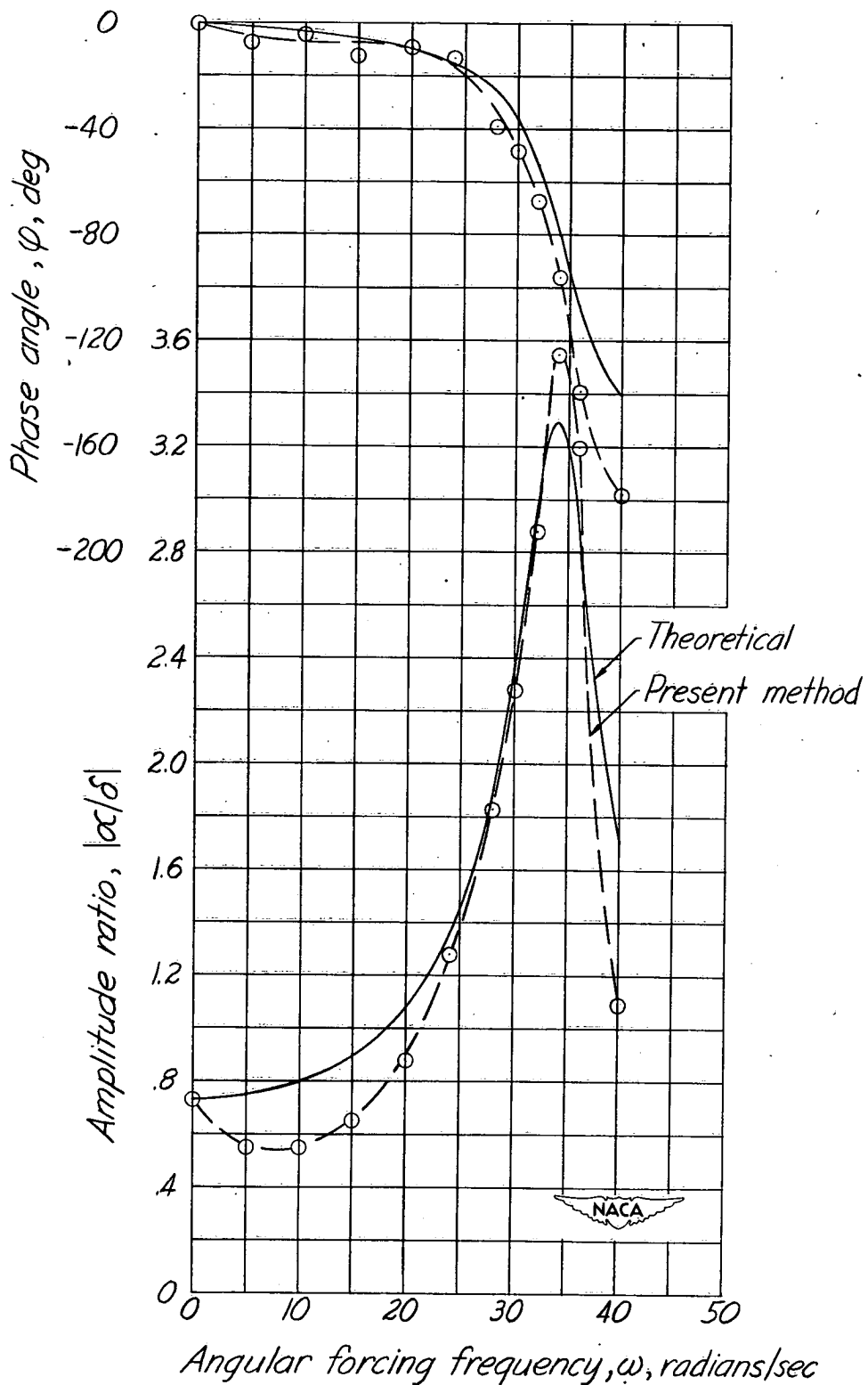
Figure 9.- Comparison of theoretical and computed aircraft angle-of-attack frequency responses as determined from flight-test data.
