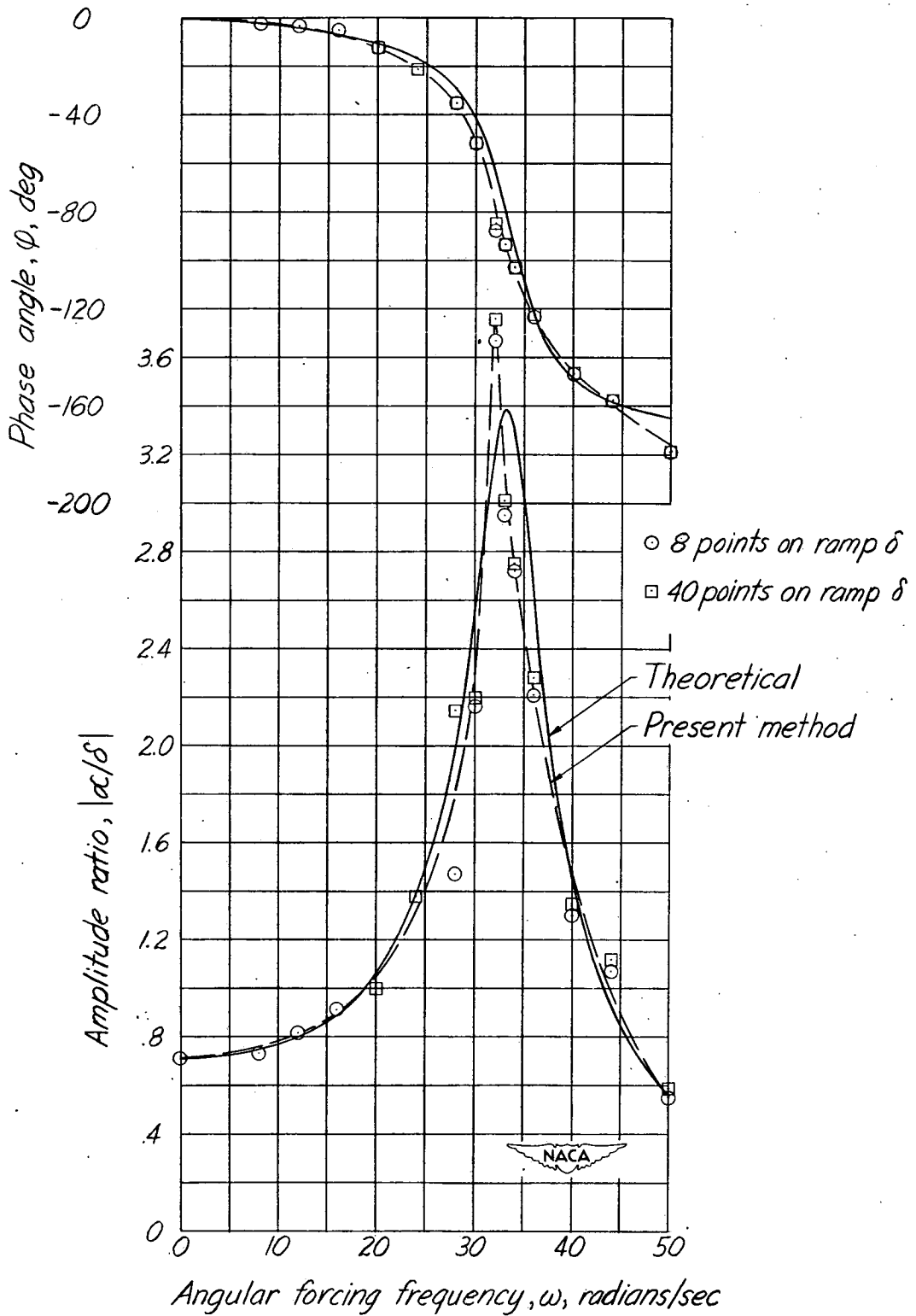
Figure 7.- Comparison of theoretical and computed frequency responses for the ramp-function-input example.
