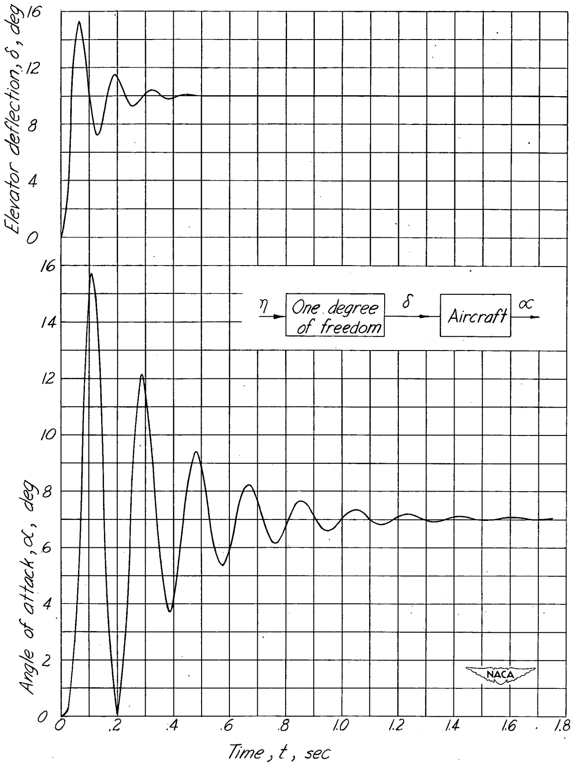
Figure 3.- Calculated input ( \delta ) and output ( \alpha ) transients.
