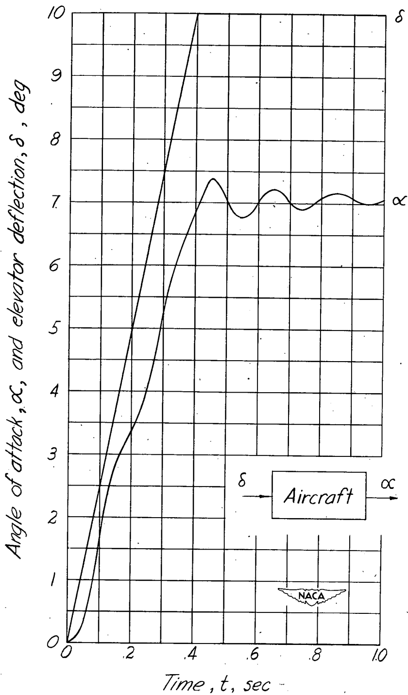
Figure 6.— The input ( \delta ) and output ( \alpha ) transients for the ramp-function-input example.
