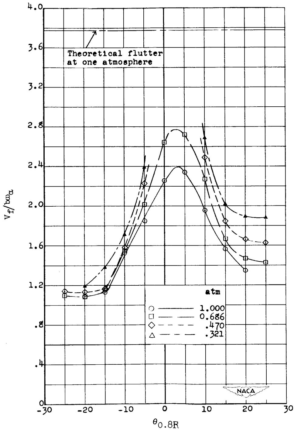
Figure 4.- Variation of reduced frequency V_F/bw_\alpha with \theta_{0.8R} .
