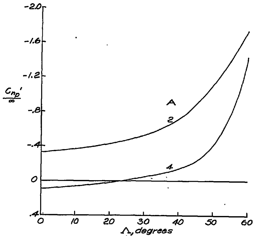
(c) Variation with angle of sweep. M = 2; λ = 0.5.
