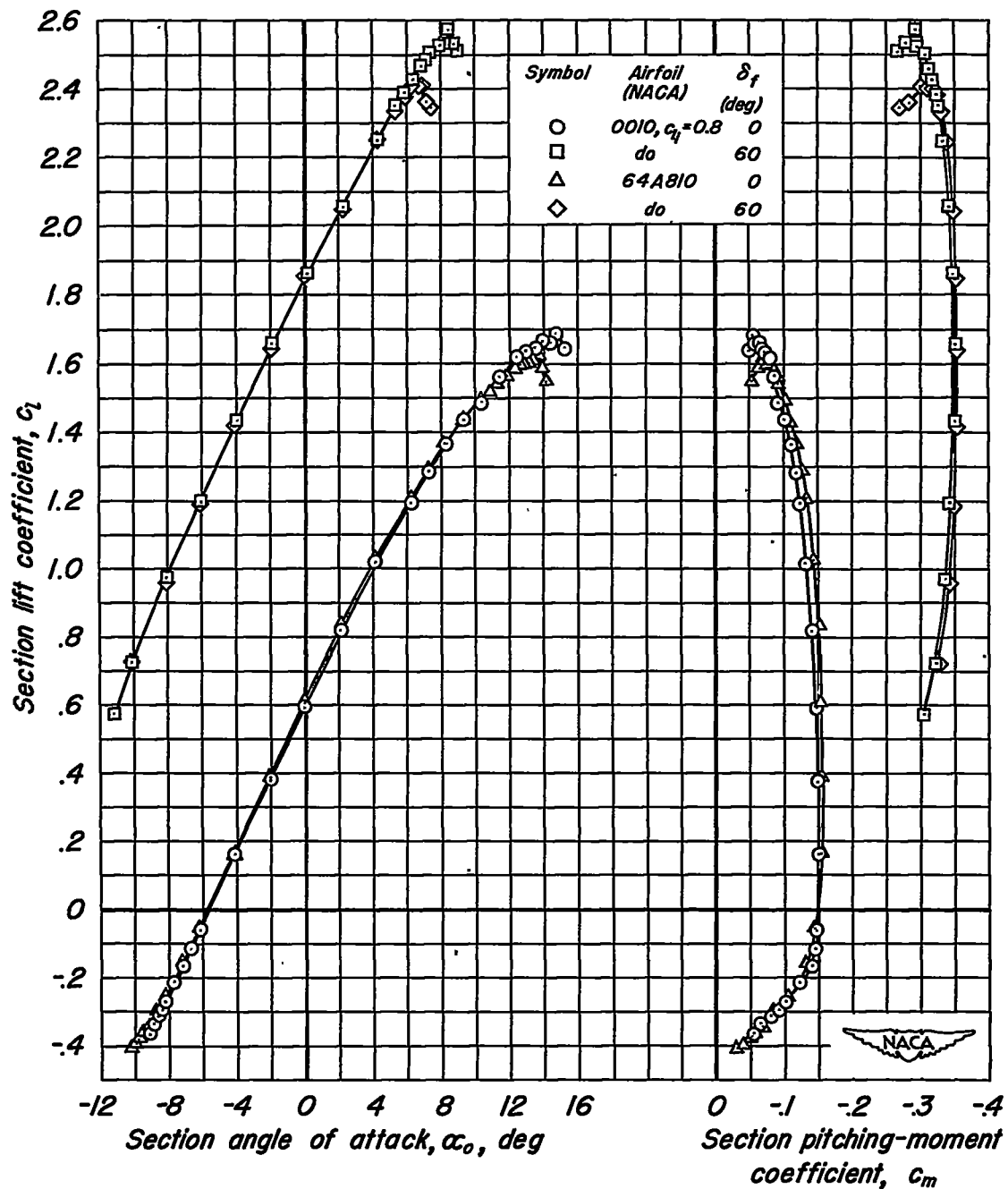
(c) Airfoils with leading-edge roughness; Reynolds number, 5.2 \times 10^6 .
