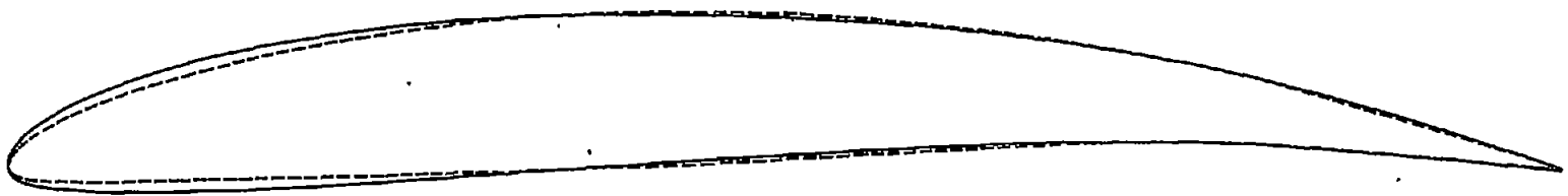
c_{l_i} = 0.8 , NACA a = 0.8 (modified) mean line
