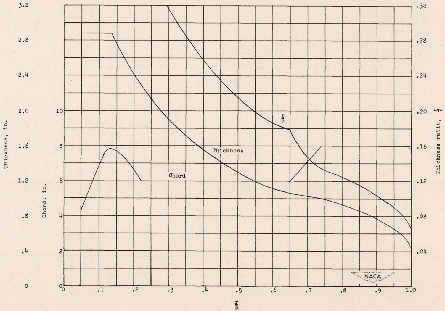
Figure 4.- Rotor-blade dimensions.
