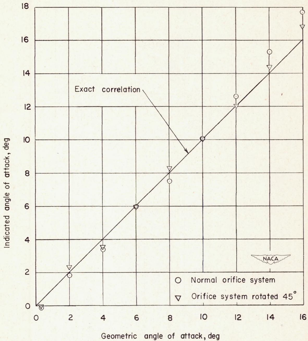
Figure 8.- Comparison of indicated and geometric angles of attack for normal orifice system and orifice system rotated 45^\circ . \psi = 0^\circ .
