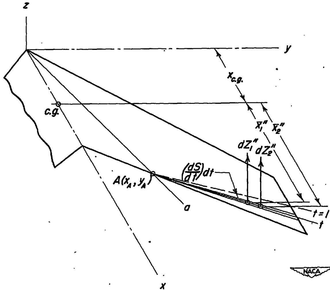
Figure 10.—Forces on an element of wing area due to the conical and quasi-conical components of an oblique pressure canceling sector in the wake.
