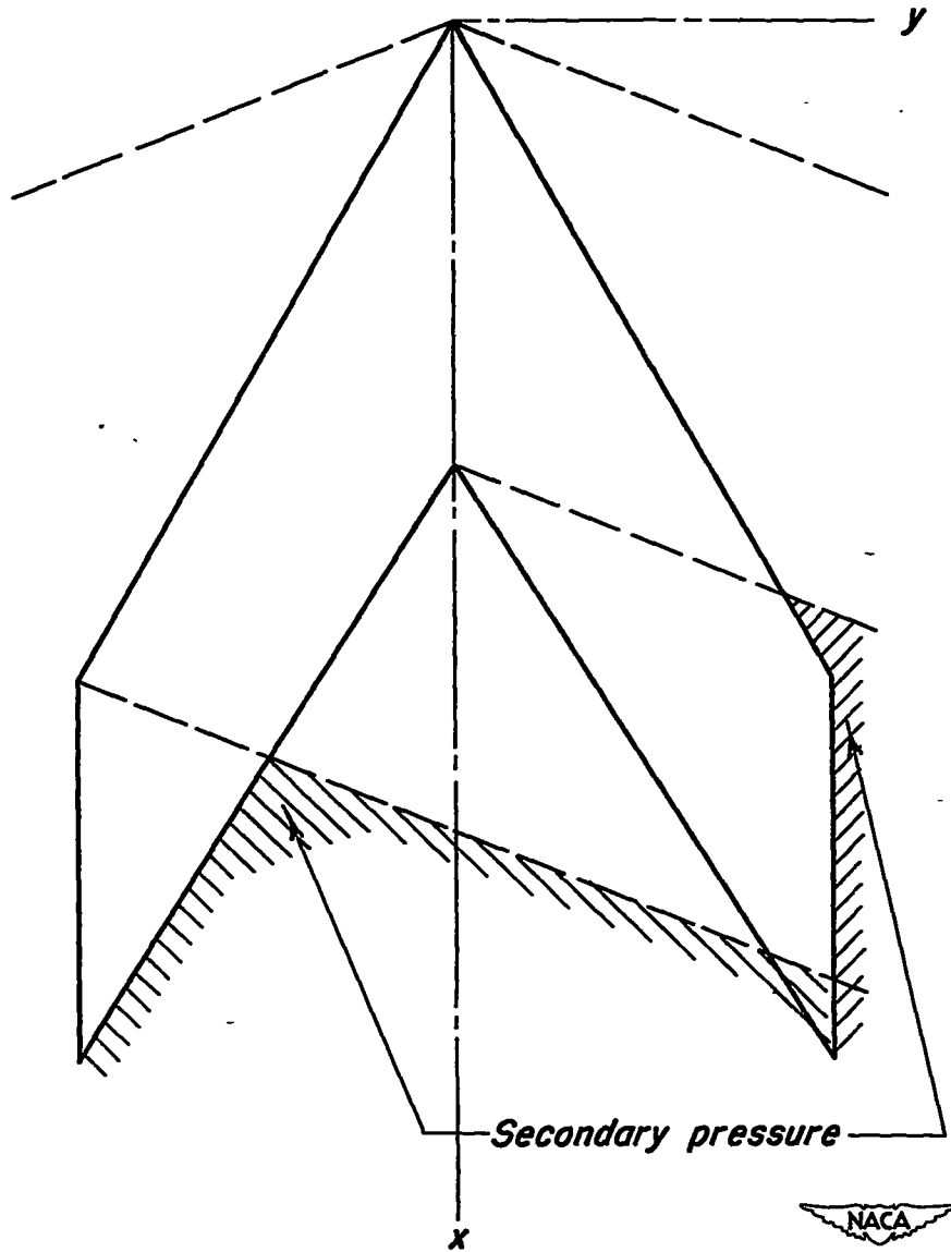
Figure 6. - Regions of secondary pressure in the wake and outboard of the tips and the leading edges.
