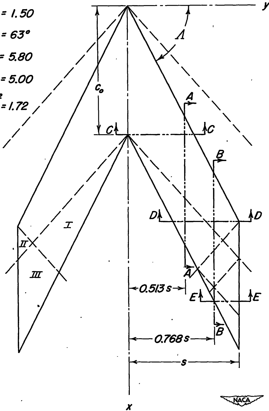
(a) Illustrative wing plan form.
