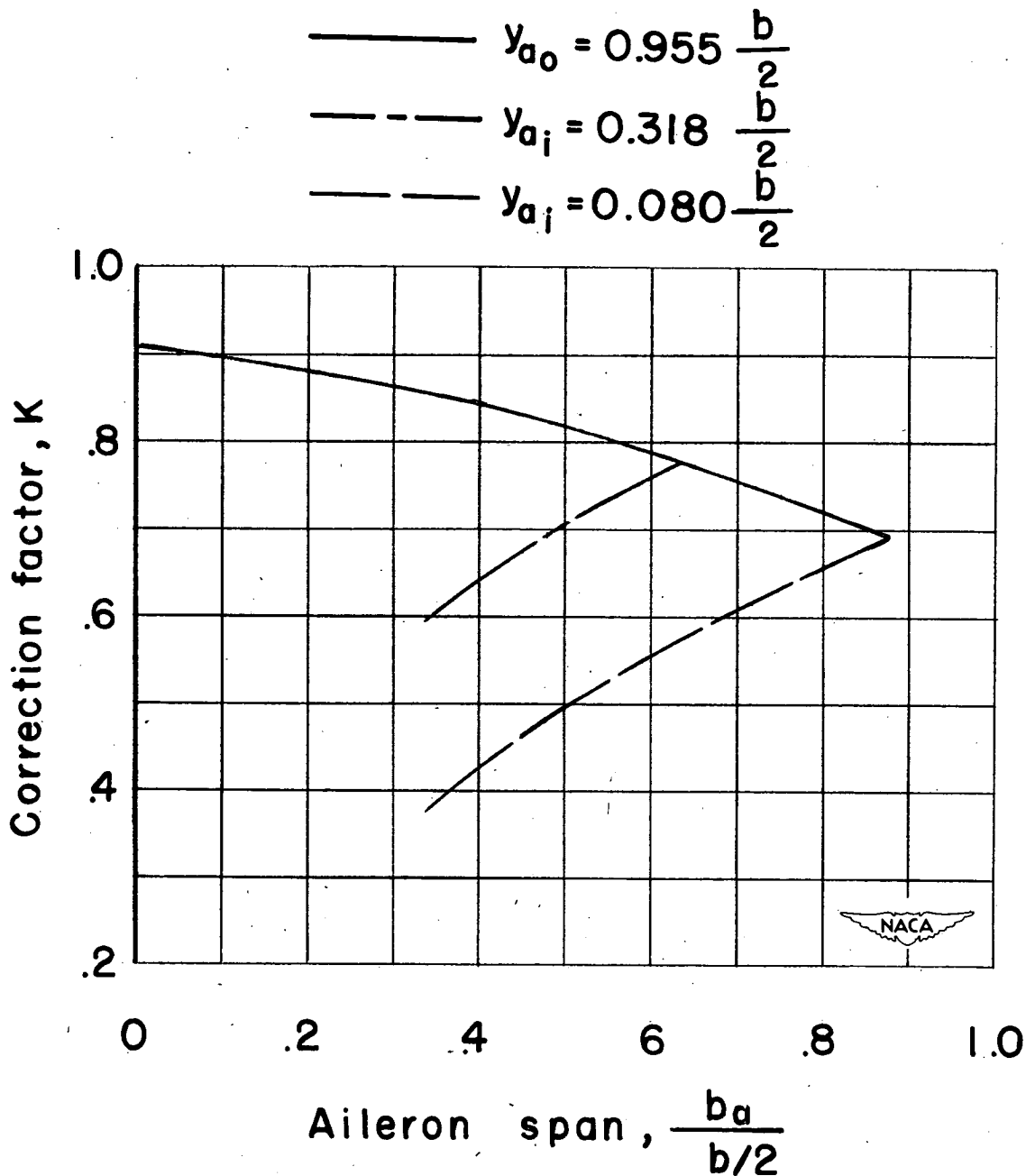
Figure 2.- Reflection-plane correction factor for rolling-moment coefficients ( C_l = KC_{l_{measured}} ).
