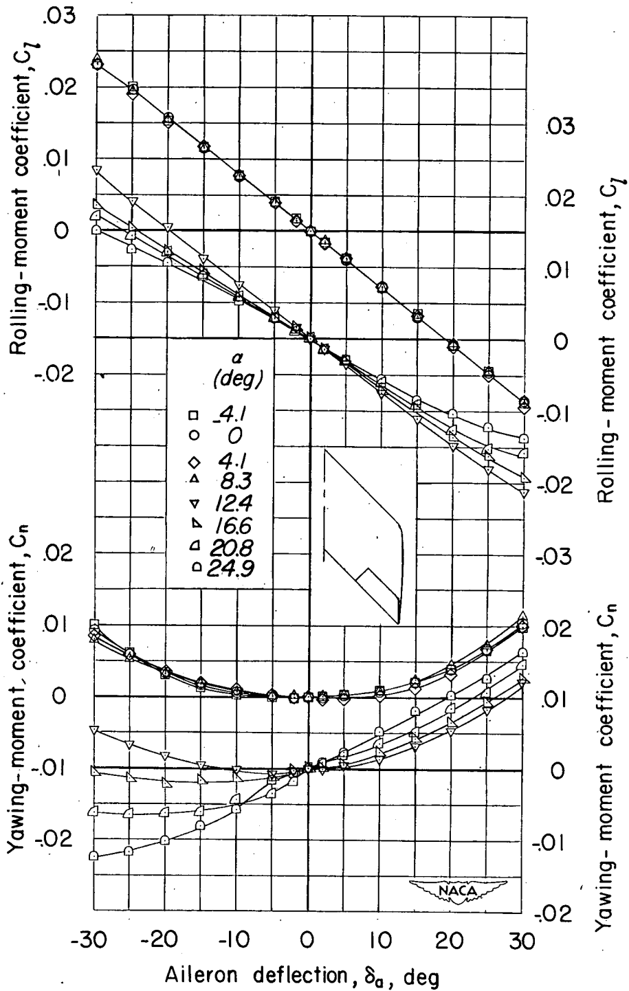
Figure 6.- Variation of lateral control characteristics with aileron deflection on the 45^\circ sweptback semispan wing having an aspect ratio of 1.59. b_a = 0.398\frac{b}{2} ; y_{a_i} = 0.557\frac{b}{2} ; y_{a_o} = 0.955\frac{b}{2} .
