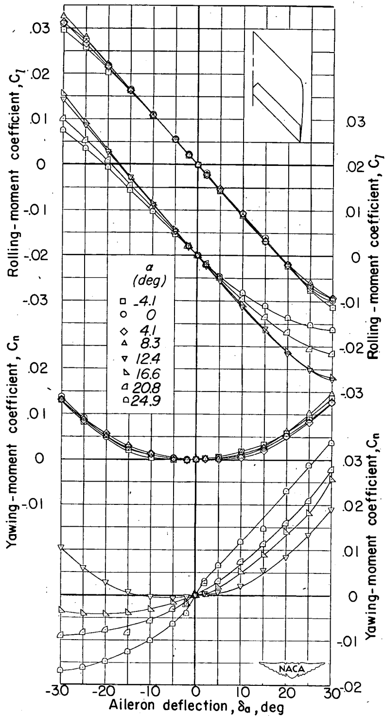
Figure 8.- Variation of lateral control characteristics with aileron deflection on the 45^\circ sweptback semispan wing having an aspect ratio of 1.59. b_a = 0.875\frac{b}{2} ; y_{a_1} = 0.080\frac{b}{2} ; y_{a_0} = 0.955\frac{b}{2} .
