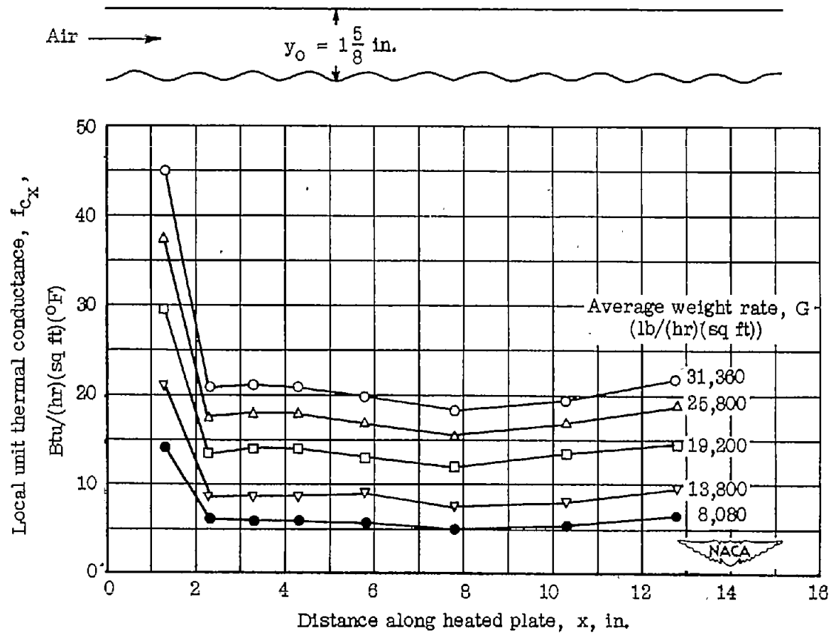
(c) Small wave plate at y_0 = 1\frac{5}{8} inches.
