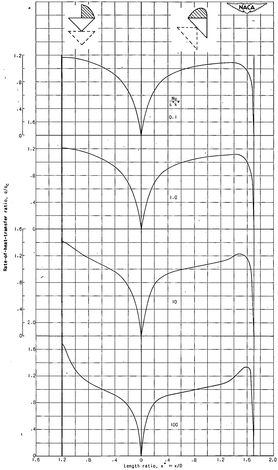
Figure 14. - Local rate of heat transfer from passage of thin-walled heat exchanger (fig. 1).
