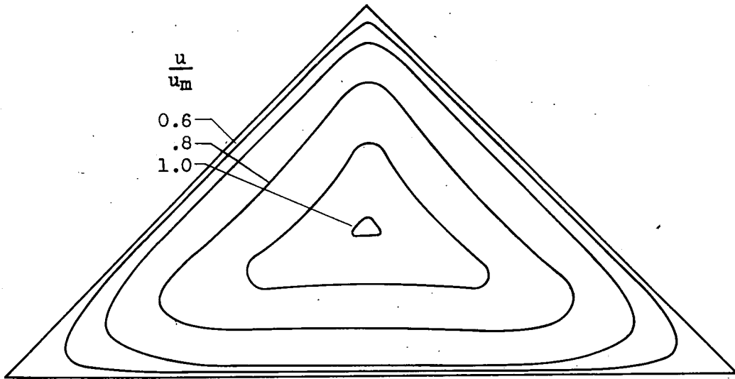
Figure 3. - Velocity contours in triangular passage as measured in reference 3. Reynolds number, 40,500.
