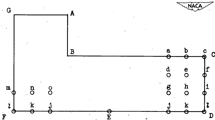
Figure 12. - Relaxation net for rectangular thick-walled heat exchanger.
