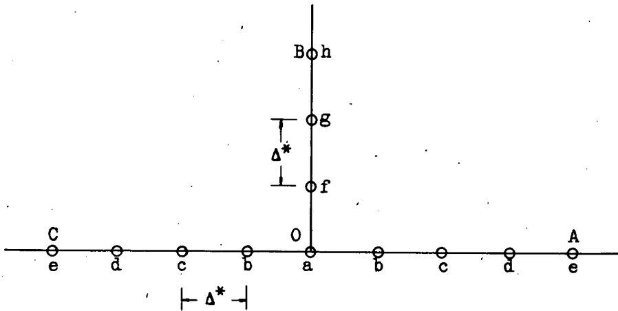
Figure 11. - Relaxation net for rectangular thin-walled heat exchanger.
