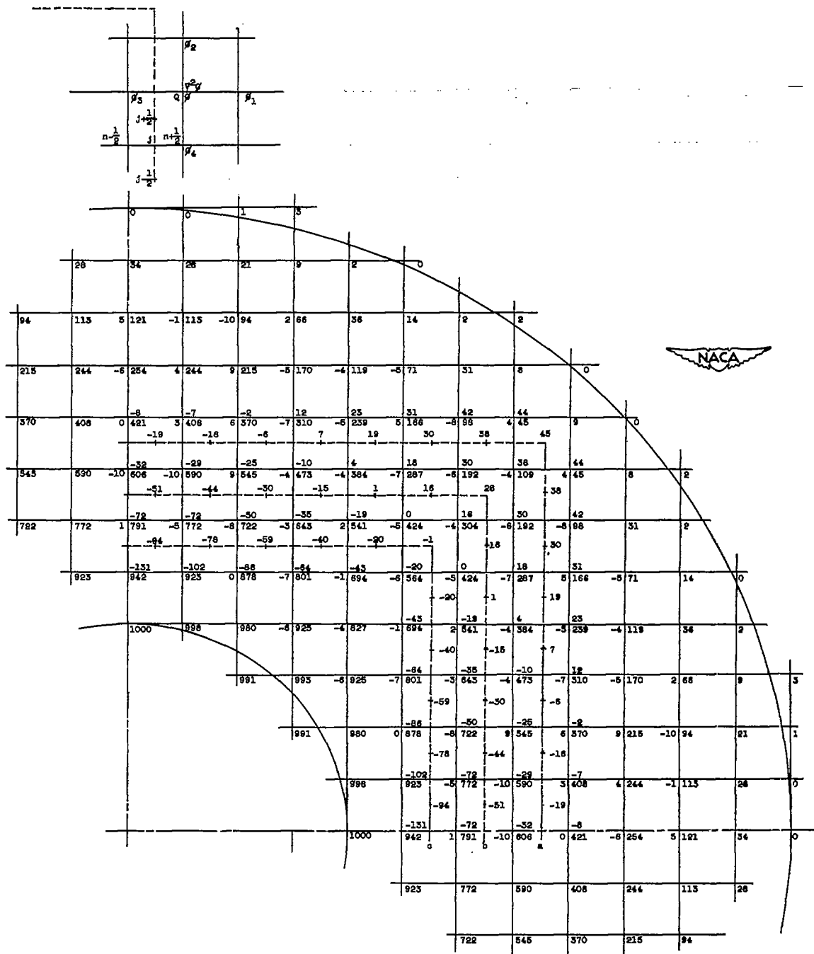
Figure 4. - Results of relaxation calculation for \phi_{13} . Values of \nabla^2\phi on integration paths are obtained by averaging \nabla^2\phi values at four nearest nodal points. \nabla^2\phi = \phi_1 + \phi_2 + \phi_3 + \phi_4 - 4\phi.
