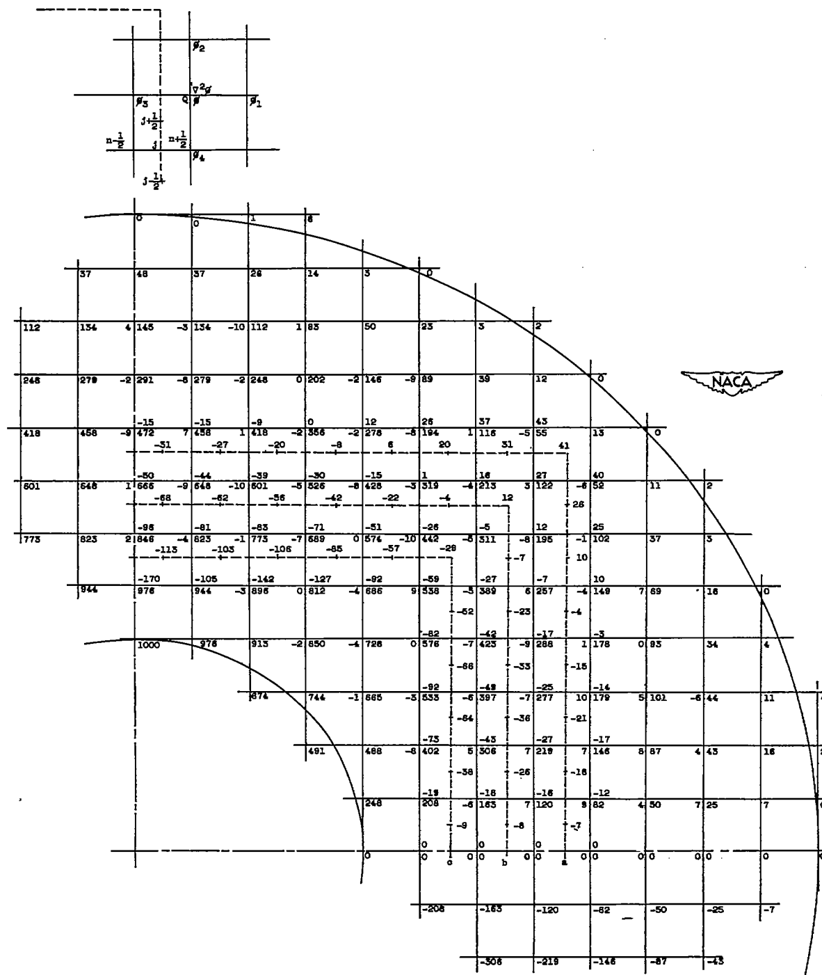
Figure 3. - Results of relaxation calculation of \phi_{12} . Values of \nabla^2\phi on integration paths are obtained by averaging \nabla^2\phi values at four nearest nodal points. \nabla^2\phi = \phi_1 + \phi_2 + \phi_3 + \phi_4 - 4\phi.
