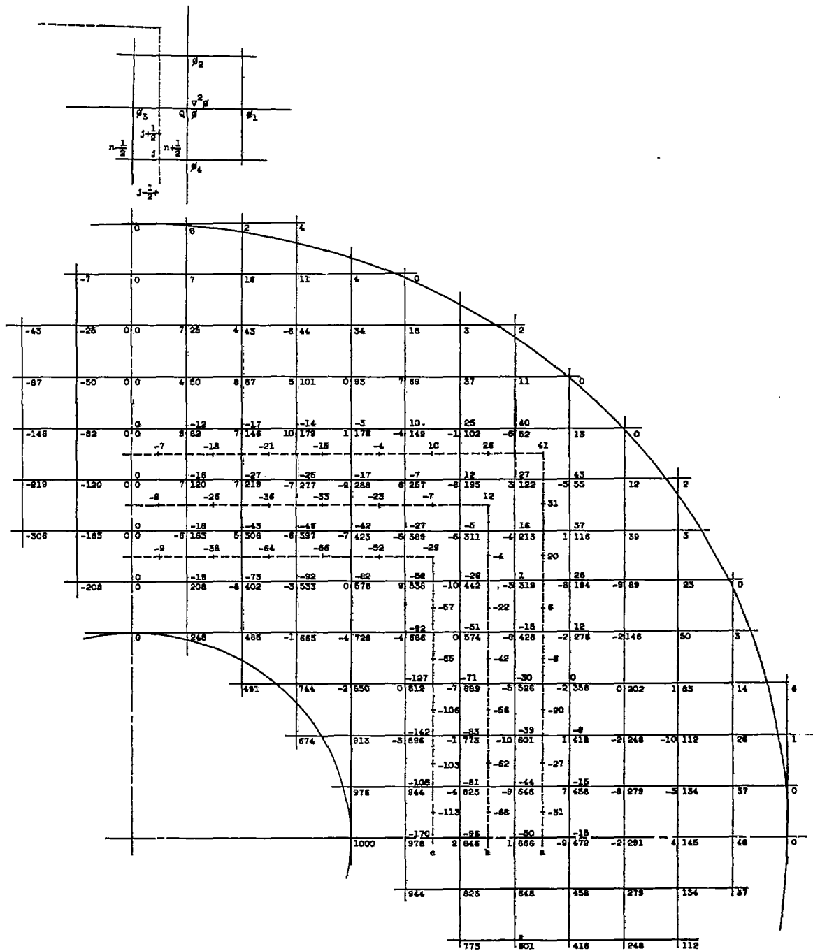
Figure 2. - Results of relaxation calculation of \phi_{11} . Values of \nabla^2 \phi on integration paths are obtained by averaging \nabla^2 \phi values at four nearest nodal points. \nabla^2 \phi = \phi_1 + \phi_2 + \phi_3 + \phi_4 - 4\phi.
