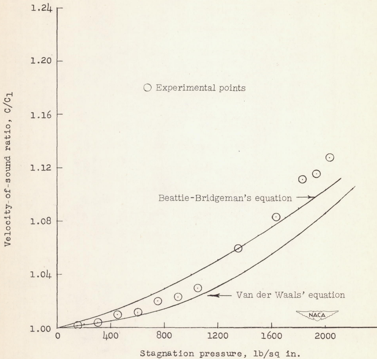
Figure 5.- Velocity-of-sound ratio for stagnation temperature of 545^{\circ} F absolute.
