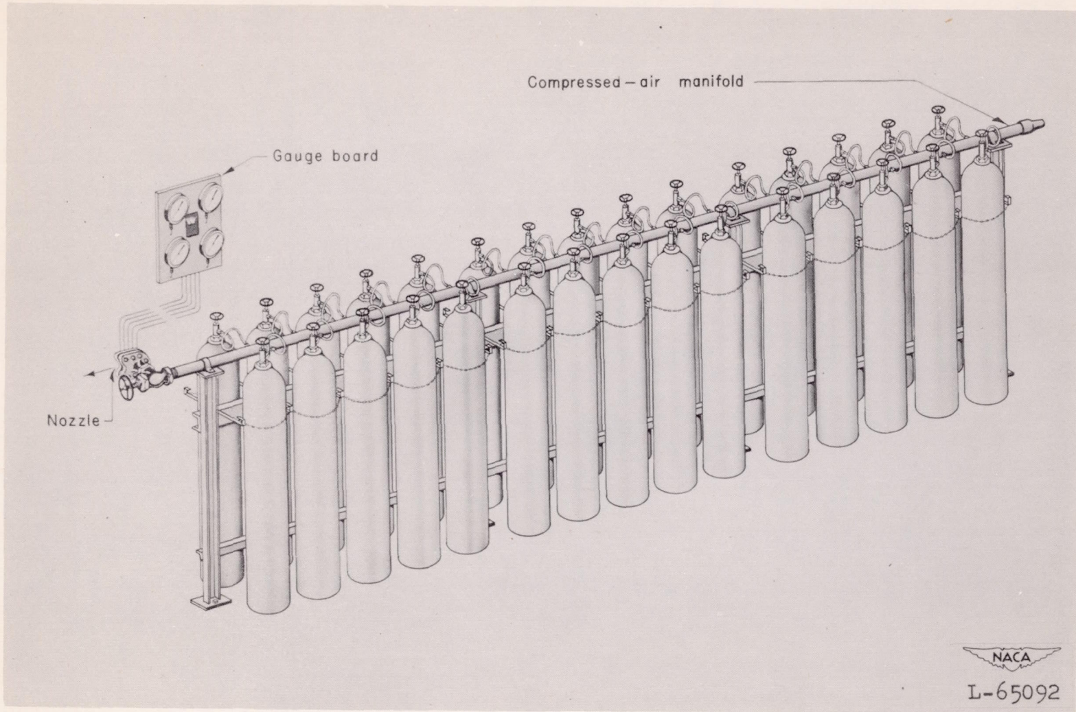
Figure 4.- Apparatus for measuring the critical pressure ratio.
