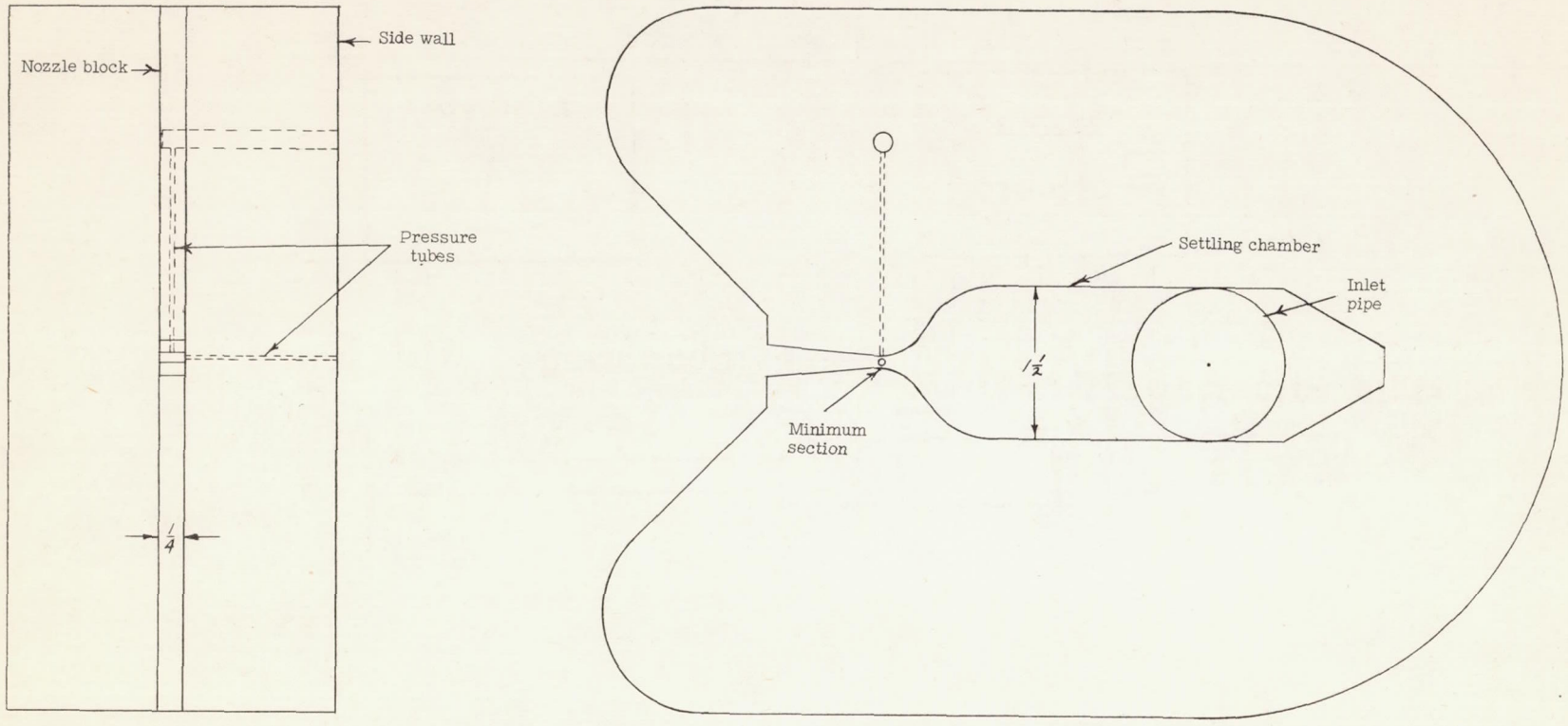
Figure 3.- Sketch of nozzle used for measuring critical pressure ratio.
