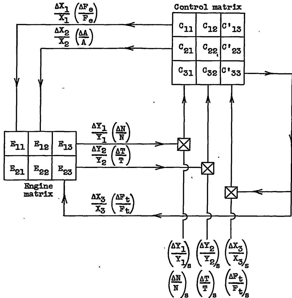
Figure 2. - Controlled-engine-system configuration.
