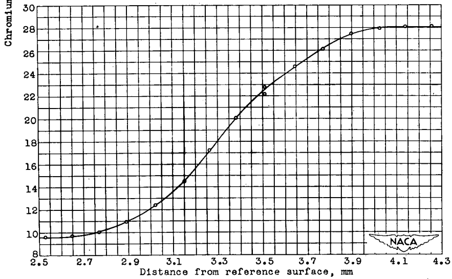
(b) Specimen 2; annealed at 1360° C for 3.384 \times 10^5 seconds (3.92 days).
