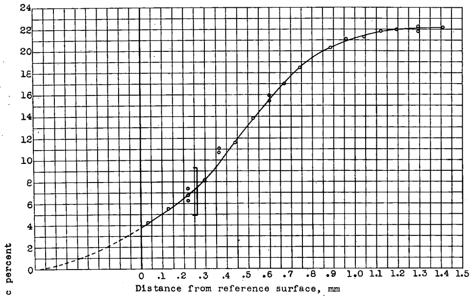
(a) Specimen 1; annealed at 1360° C for 3.384 \times 10^5 seconds (3.92 days). Data to left of bracket are inaccurate because of quench crack, which formed after diffusion had taken place.
