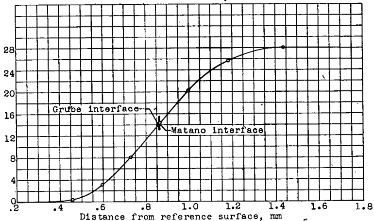
(d) Specimen 3; annealed at 1303° C for 3.522 \times 10^5 seconds (4.08 days).
