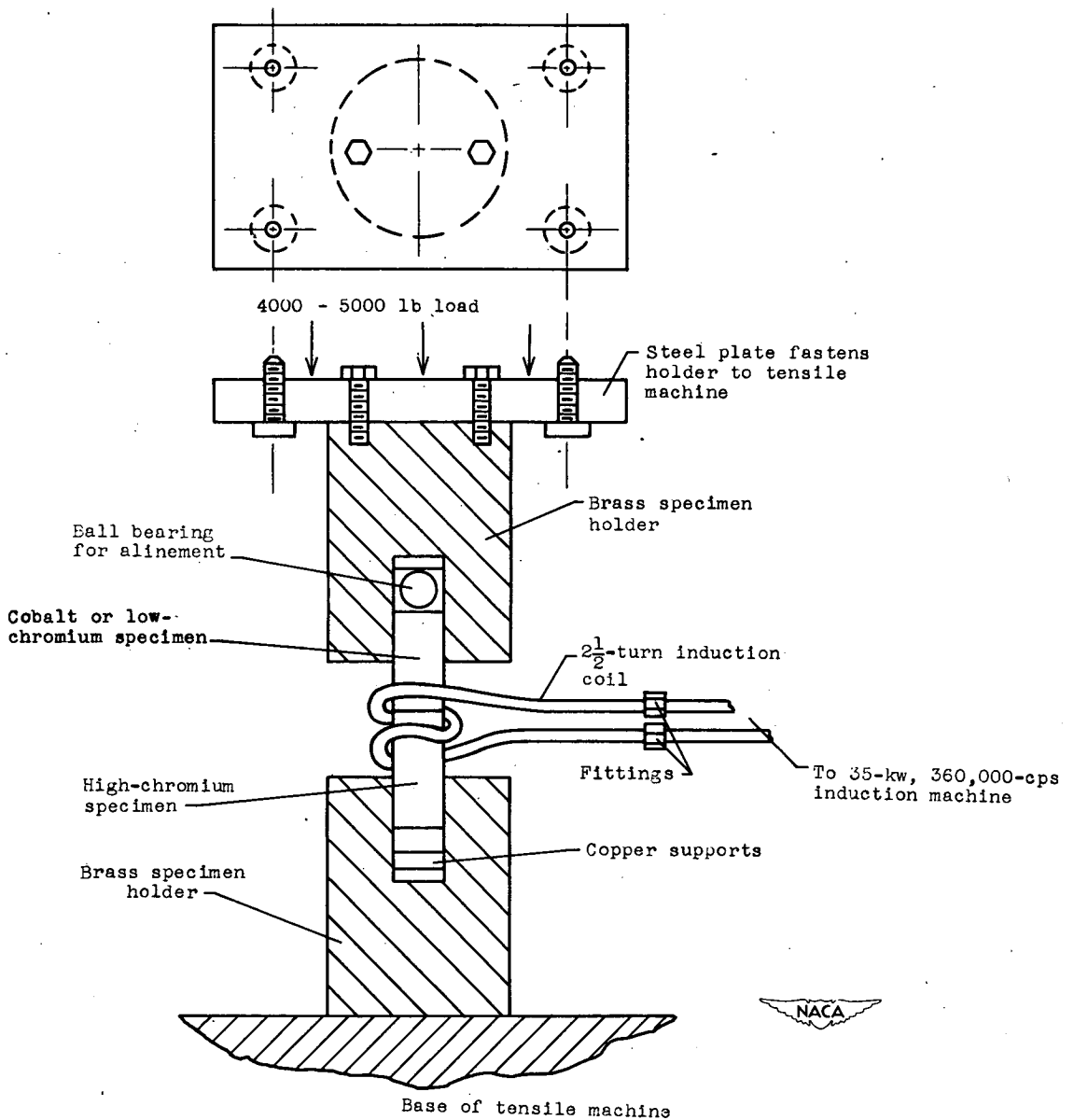
Figure 2. - Pressure-welding apparatus.
