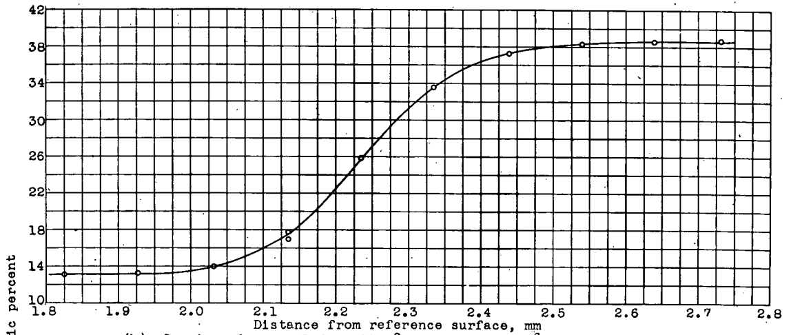
(h) Specimen 6; annealed at 1150° C for 1.0446x10 6 seconds (12.09 days).
