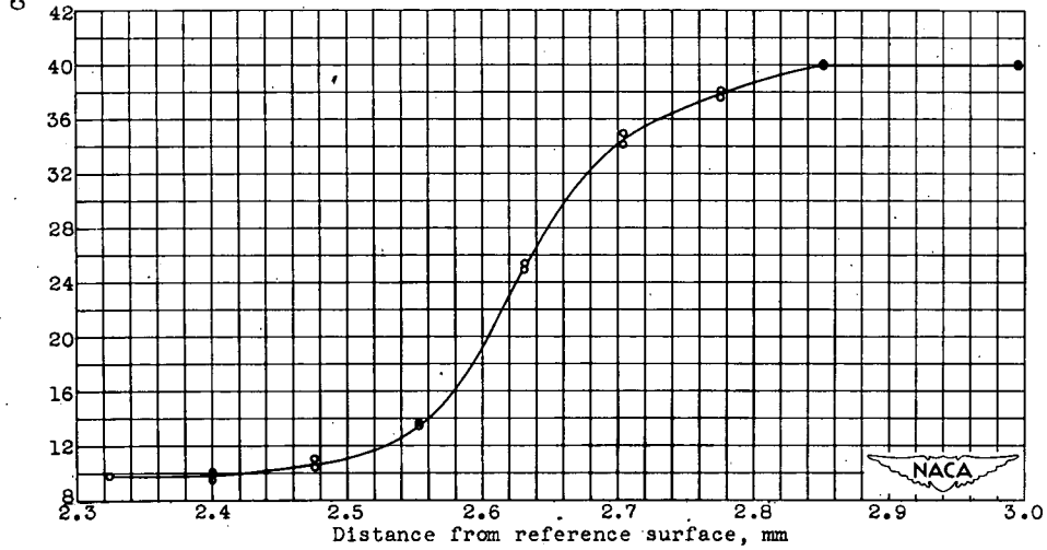
(k) Specimen 9; annealed at 1000° C for 7.664 \times 10^6 seconds (87.70 days).
