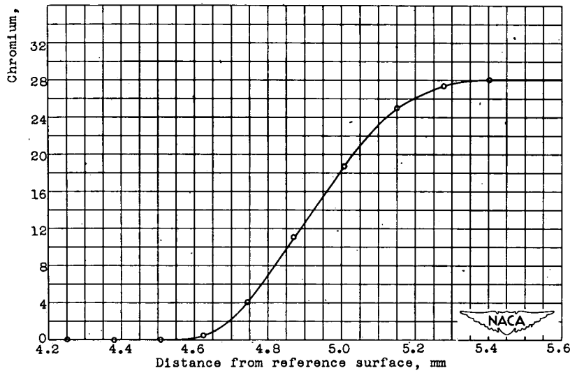
(i) Specimen 7; annealed at 1151° C for 2.152x10 6 seconds (24.91 days).
