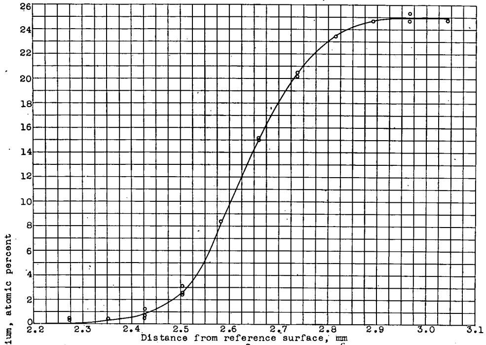
(j) Specimen 8; annealed at 1000° C for 7.664 \times 10^6 seconds (87.70 days).
