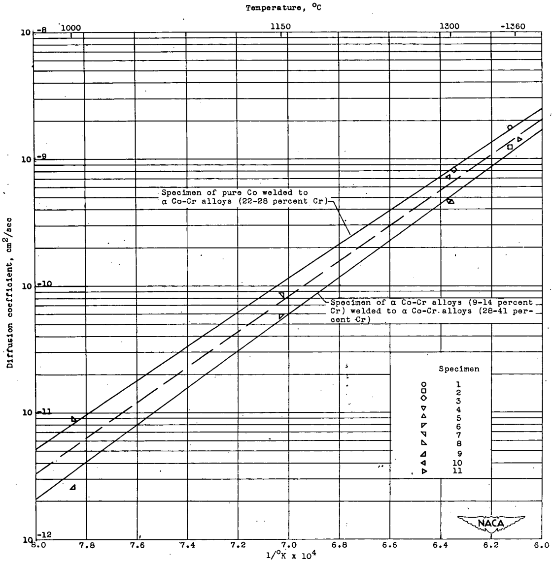
Figure 14. - Diffusion coefficients against 1/°K. Diffusion coefficients were plotted from data for 16-atomic-percent chromium.
