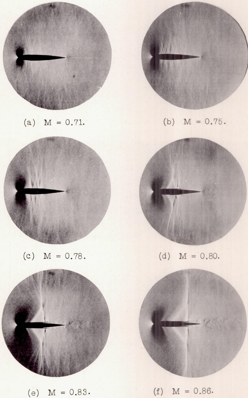
Figure 3.- Schlieren photographs of the flow on the NACA 0012 wing of infinite aspect ratio at 0^\circ angle of attack.
