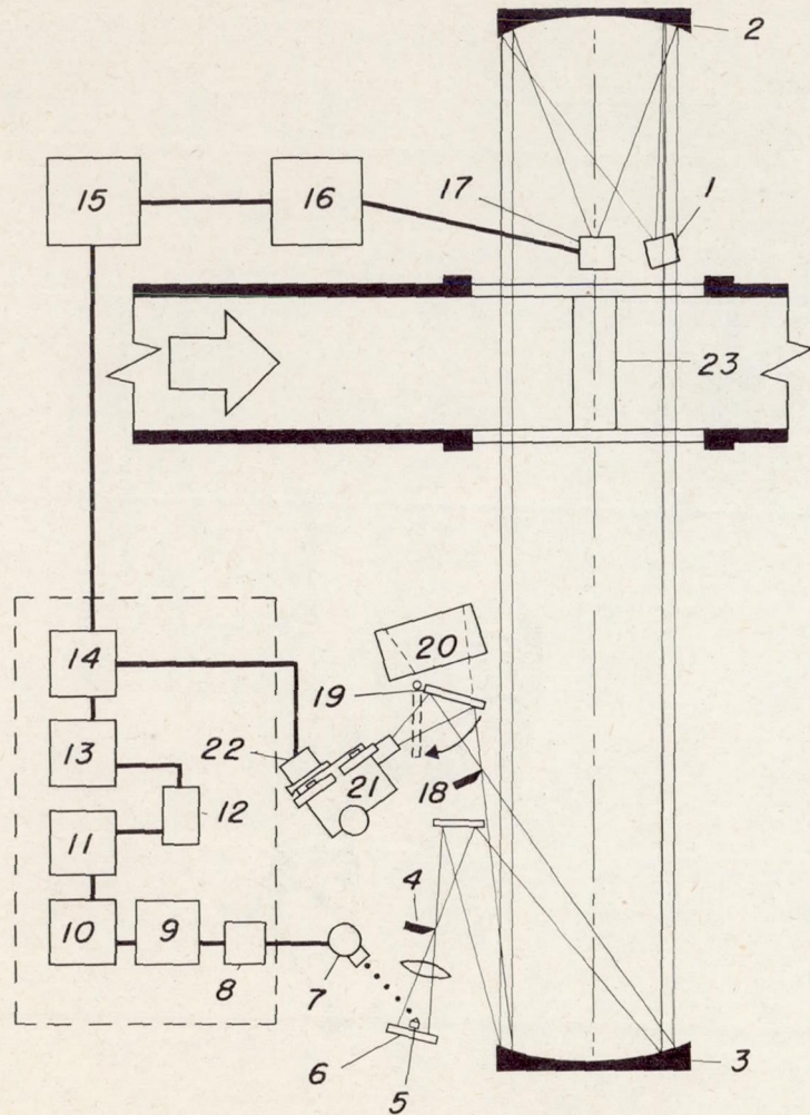
Figure 2.- Block diagram of the self-synchronizing stroboscope apparatus.
