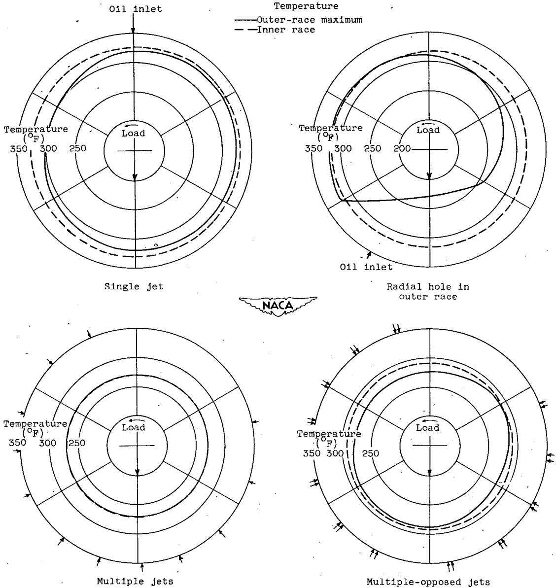
Figure 6. - Effect of oil distribution on circumferential temperature distribution of bearing 5 for four methods of lubrication. Methods of lubrication, single jet, radial hole in outer race, multiple jets, and multiple-opposed jets; DN, 1.2 \times 10^6 ; oil inlet temperature, 100^\circ F; oil flow, 2.8 pounds per minute; load, 368 pounds.
