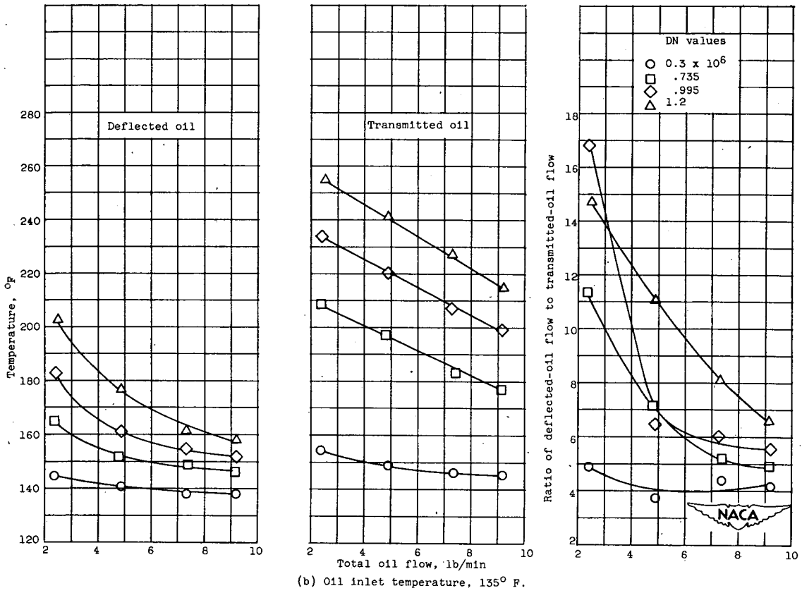
Figure 8. - Continued. Effect of oil flow on deflected- and transmitted-oil temperatures of bearing 10 for various DN values and oil inlet temperatures. Oil flow, 2.2 to 9.3 pounds per minute; DN, 0.3 \times 10^6 to 1.2 \times 10^6 ; oil-jet diameter, 0.050 inch; load, 368 pounds.
