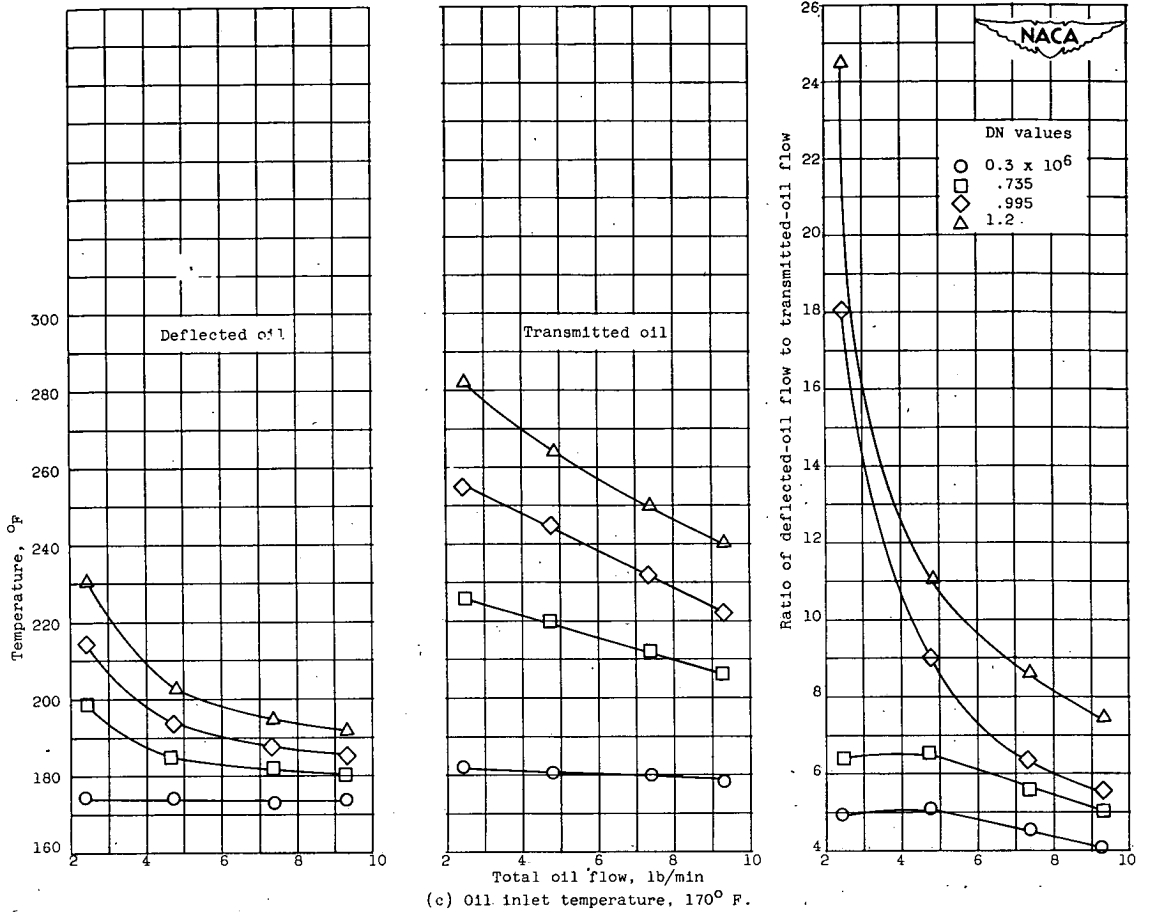
Figure 8. - Continued. Effect of oil flow on deflected- and transmitted-oil temperatures of bearing 10 for various DN values and oil inlet temperatures. Oil flow, 2.2 to 9.3 pounds per minute; DN, 0.3 \times 10^6 to 1.2 \times 10^6 ; oil-jet diameter, 0.050 inch; load, 368 pounds.
