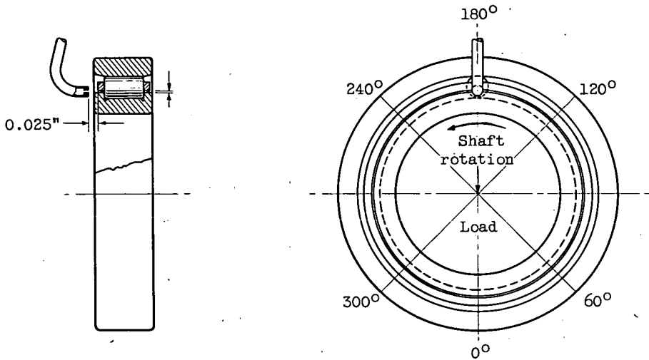
(a) Single jet.
