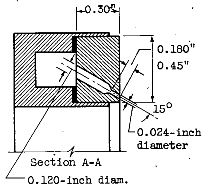
(g) Construction of circular manifold.
