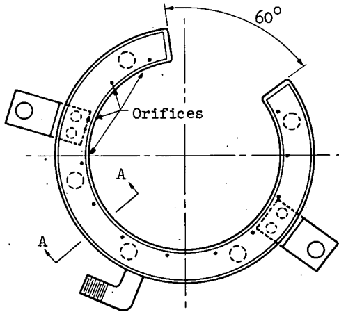
(f) Mounting arrangement of circular manifold for multiple jet arrangements (figs. 2(d) and 2(e)).
