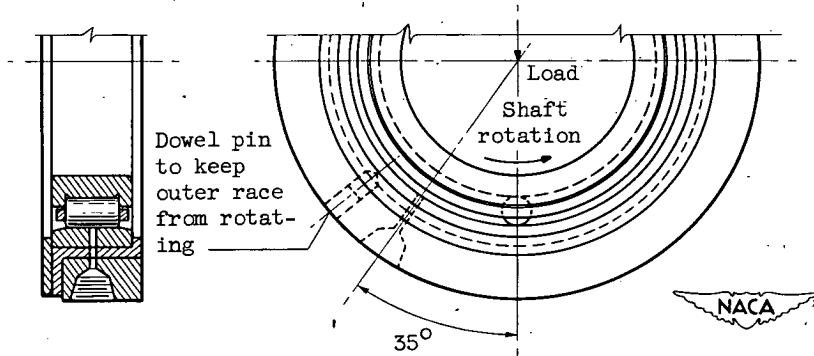
(c) Outer-race radial hole (diam. of orifice, 0.089 in.).
