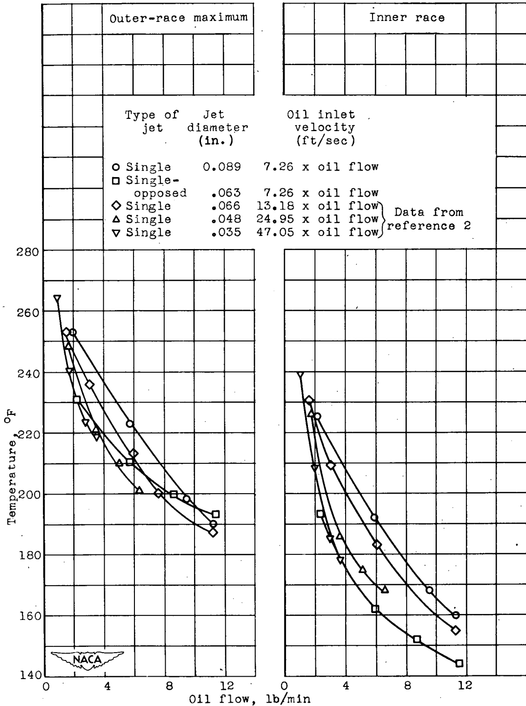
Figure 9. - Effect of oil flow on outer-race-maximum and inner-race temperatures of bearing 6 for single-opposed jets and single jets of various sizes. Oil flow, 1.2 to 11.5 pounds per minute; DN, 1.2 \times 10^6 ; oil inlet temperature, 100^\circ\text{F} ; load, 368 pounds.
