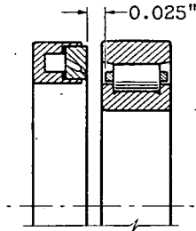
(d) Multiple jets from circular manifold (12 orifices, each 0.024 inch diam.).
