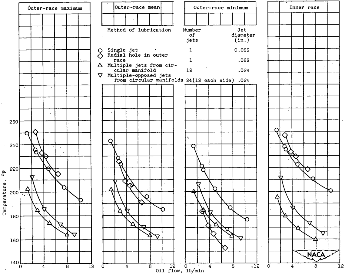
Figure 5. - Effect of oil flow on outer-race maximum, mean, and minimum and inner-race temperatures of bearing 5 for four methods of lubrication at various DN values and loads. Oil flow, 1.5 to 10.3 pounds per minute; methods of lubrication, single jet, radial hole in outer race, multiple jets from circular manifold, and multiple-opposed jets from circular manifolds; oil inlet temperature, 100° F.
