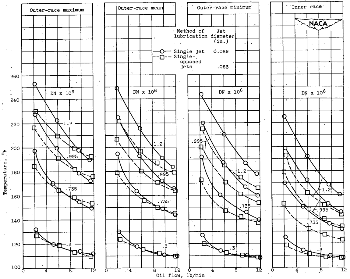
Figure 4. - Effect of oil flow on outer-race maximum, mean, and minimum and inner-race temperatures of bearing 6 for comparison of two methods of lubrication over range of DN values. Oil flow, 2 to 12 pounds per minute; methods of lubrication, single-jet and single-opposed jets; DN, 0.3 \times 10^6 to 1.2 \times 10^6 ; oil inlet temperature, 100° F; load, 368 pounds.
