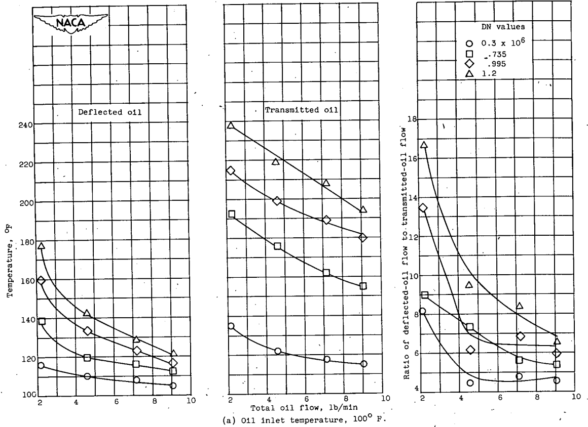
Figure 8. - Effect of oil flow on deflected- and transmitted-oil temperatures of bearing 10 for various DN values and oil inlet temperatures. Oil flow, 2.2 to 9.3 pounds per minute; DN, 0.3 \times 10^6 to 1.2 \times 10^6 ; oil-jet diameter, 0.050 inch; load, 368 pounds.
