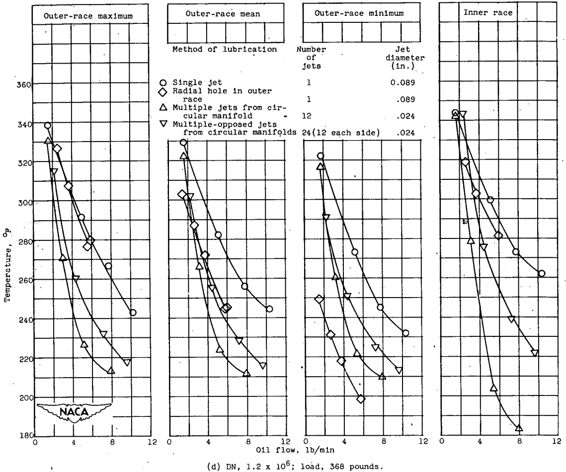
Figure 5. - Concluded. Effect of oil flow on outer-race maximum, mean, and minimum and inner-race temperatures of bearing 5 for four methods of lubrication at various DN values and loads. Oil flow, 1.5 to 10.3 pounds per minute; methods of lubrication, single jet, radial hole in outer race, multiple jets from circular manifold, and multiple-opposed jets from circular manifolds; oil inlet temperature, 100° F.
