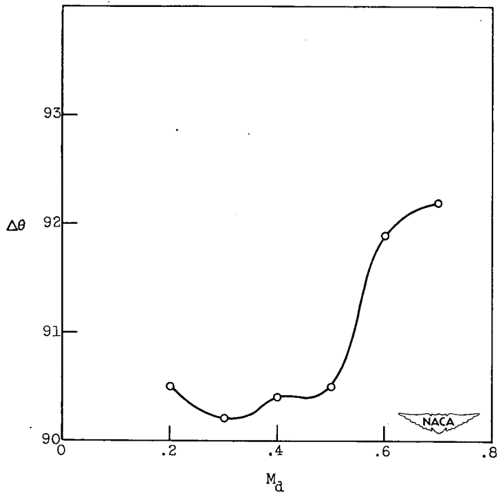
Figure 17. - Variation in air-turning angle with downstream Mach number.
