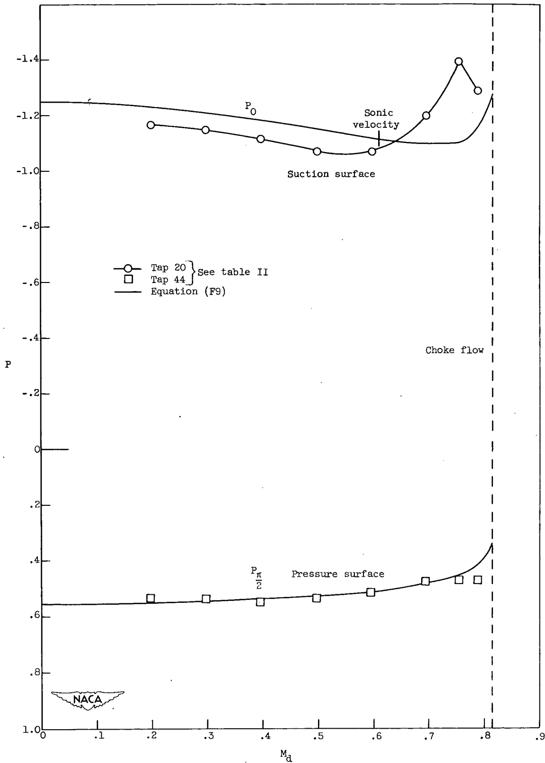
Figure 22. - Variation in pressure coefficient P with downstream Mach number M_d at static taps on pressure and suction surfaces of blade and at equivalent radii of a free compressible vortex.
