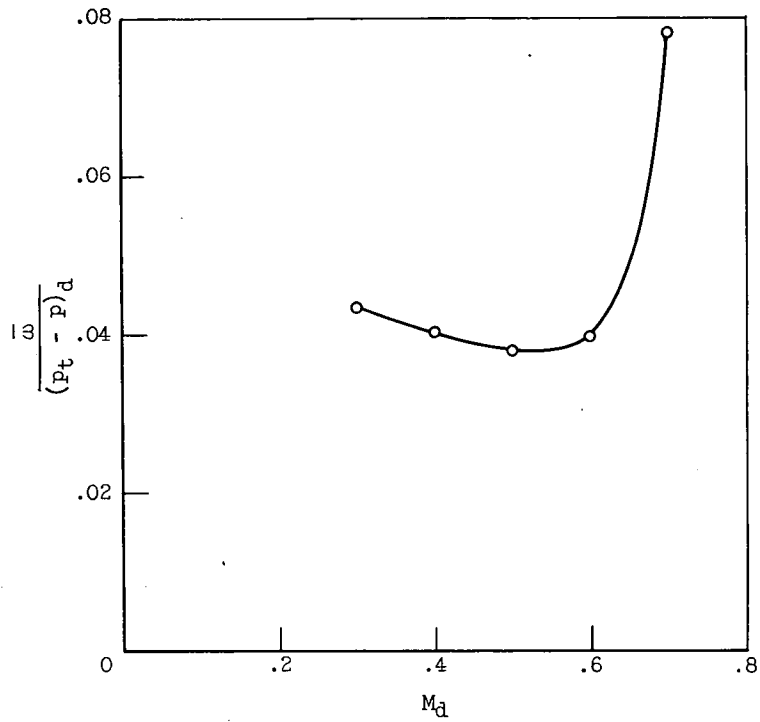
Figure 16. - Variation in pressure-loss coefficient with downstream Mach number.
