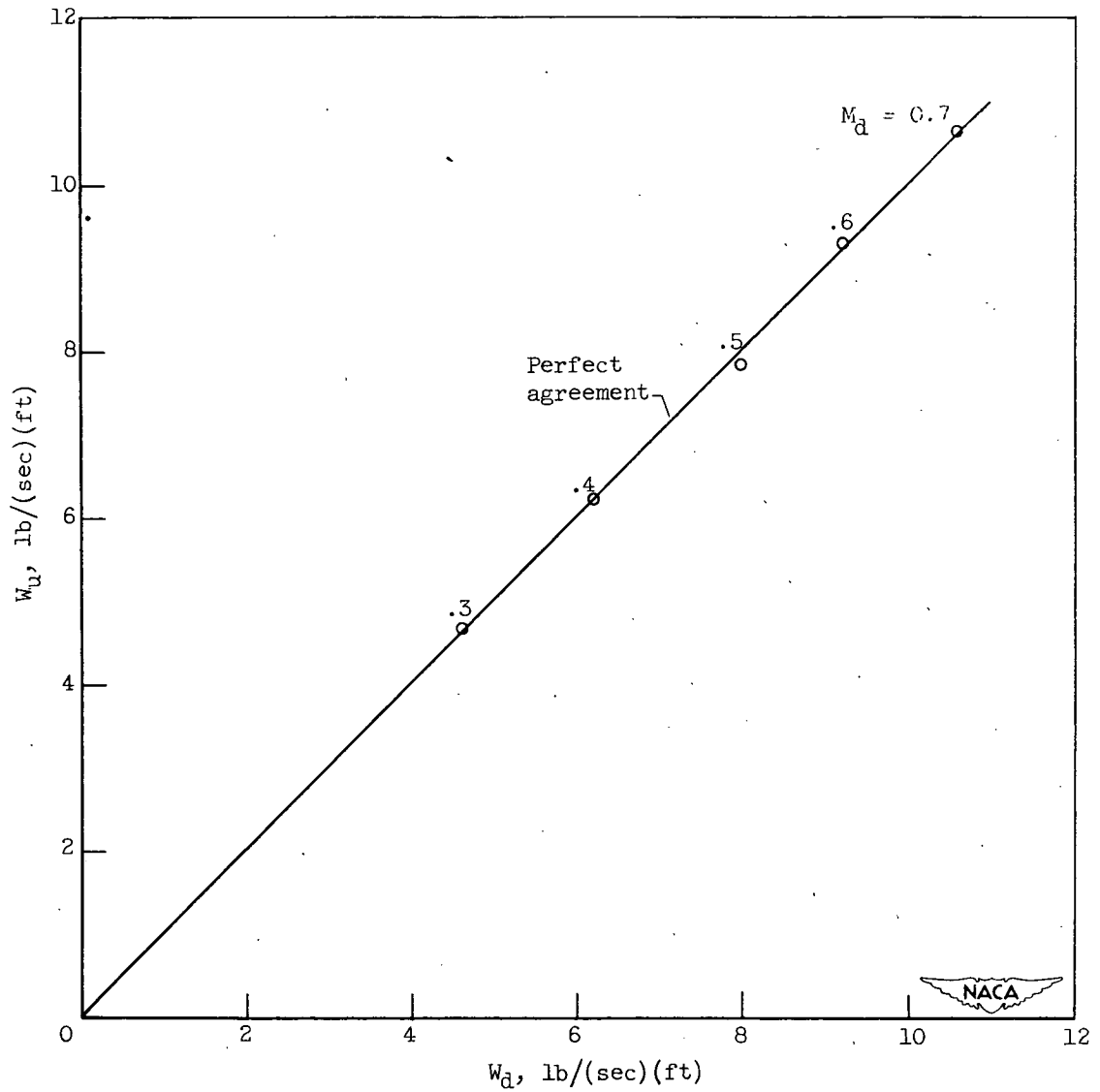
Figure 20. - Comparison of measured flow rates upstream and downstream of cascade for five values of downstream Mach number.
