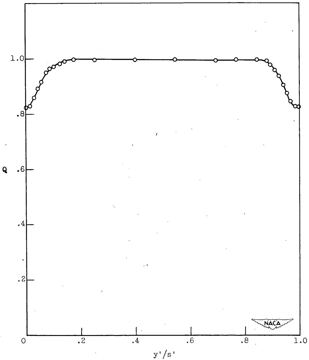
Figure 19. - Variation in Q with y'/s' between wakes downstream of cascade. Downstream Mach number M_d , 0.30.
