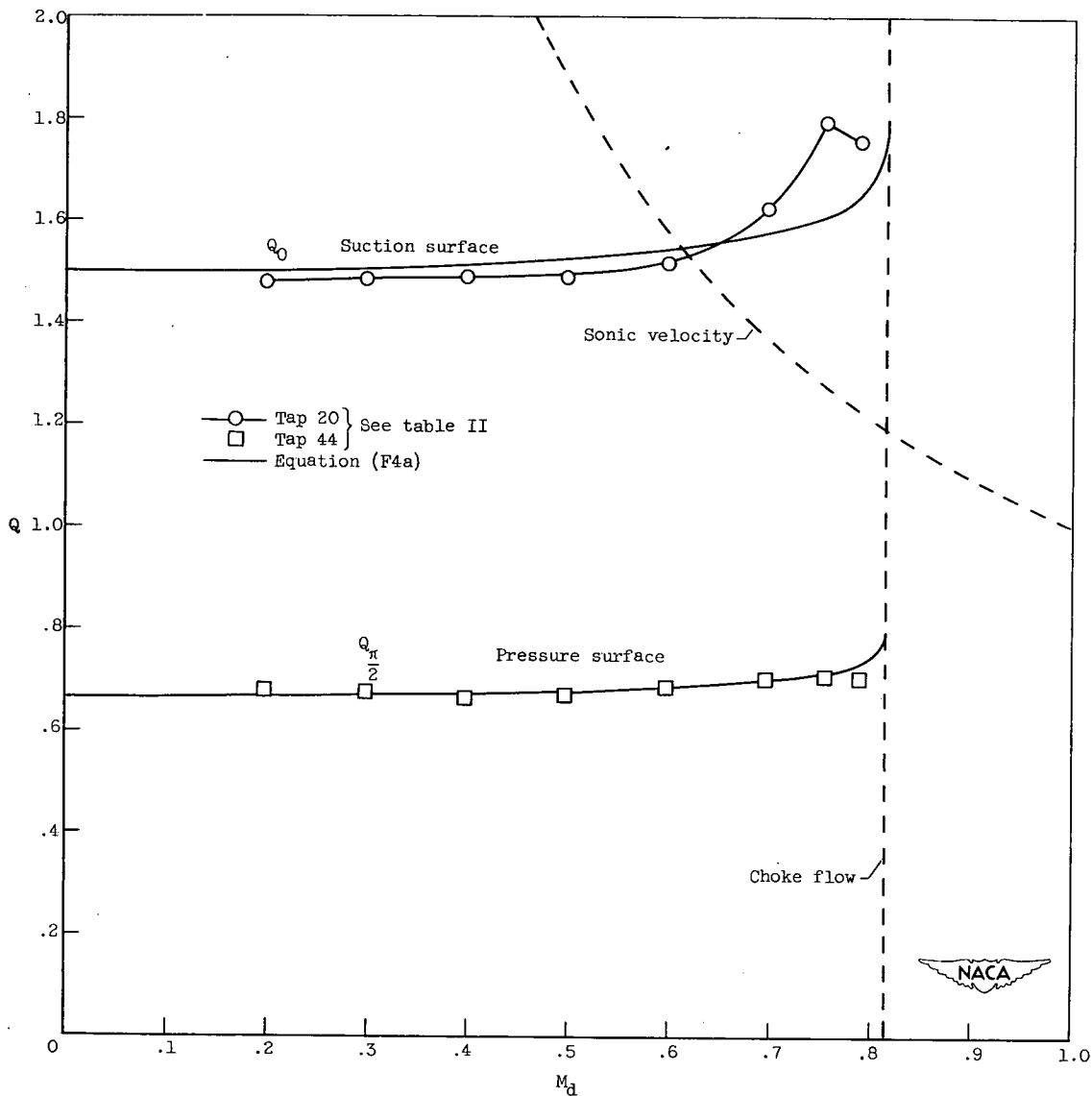
Figure 21. - Variation in velocity Q with downstream Mach number M_d at static taps on pressure and suction surfaces of blade and at equivalent radii of a free compressible vortex.
