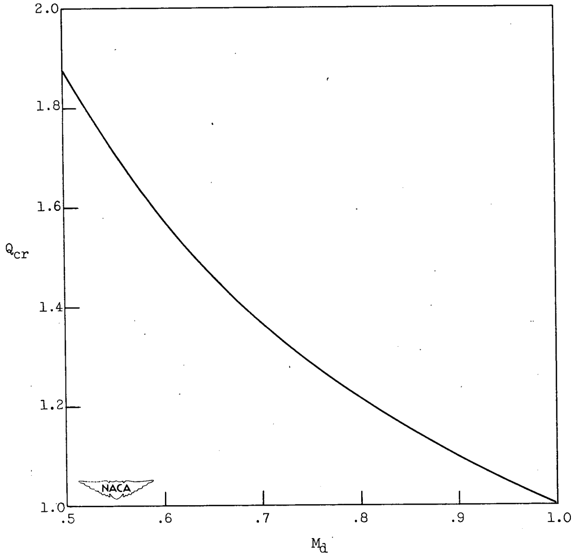
Figure 23. - Variation in Q_{cr} with downstream Mach number. (For a given value of M_d , sonic velocity occurs at Q_{cr} .)
