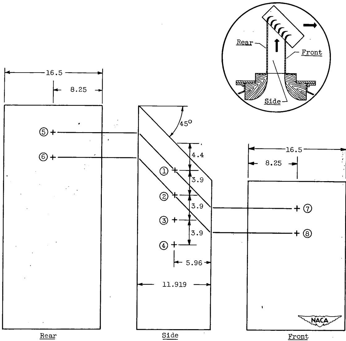
Figure 11. - Static-pressure tap locations on tunnel walls. Circled numbers are tap numbers. All linear dimensions in inches.
