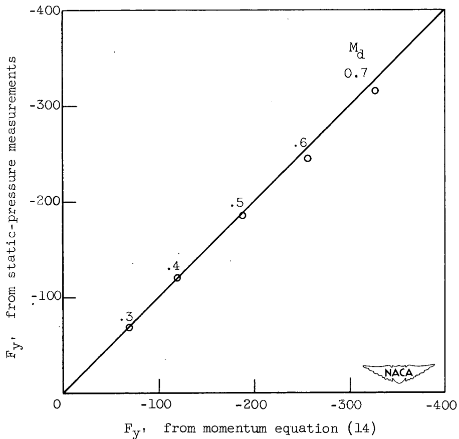
Figure 24. - Comparison of blade force in direction of y' as determined from measured static pressures on blade surface and from momentum equation (14).
