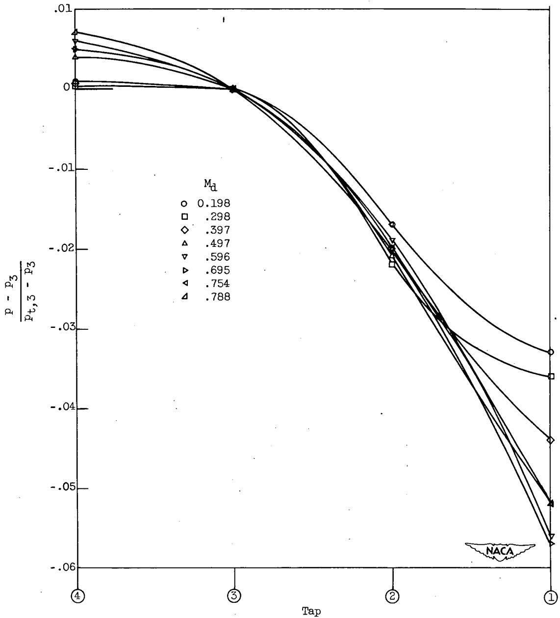
Figure 12. - Variation in static pressure (with downstream Mach number) at four tunnel wall taps indicated by corresponding circled numbers in figure 11.
