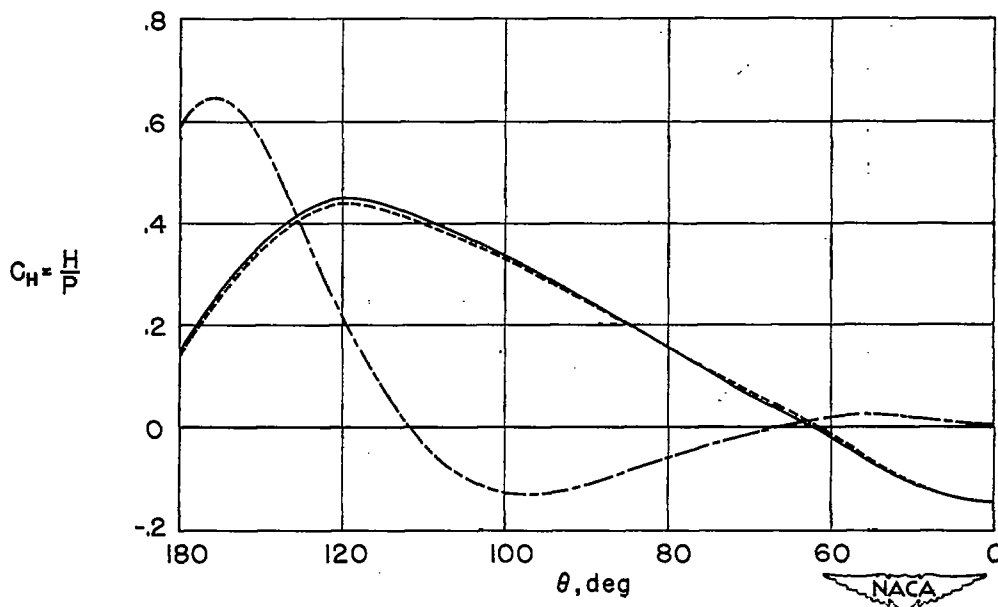
(b) Ring axial force.
