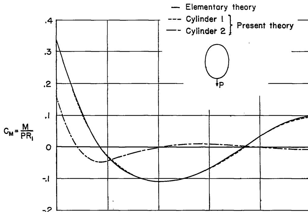
(a) Ring bending moment.
