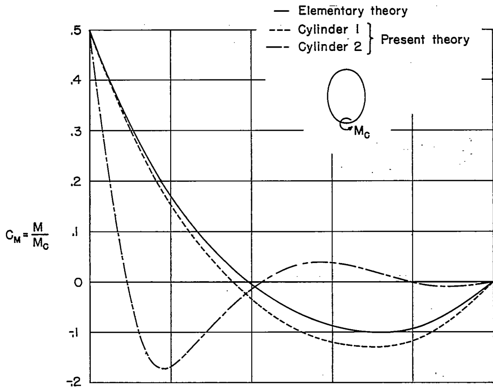
(a) Ring bending moment.
