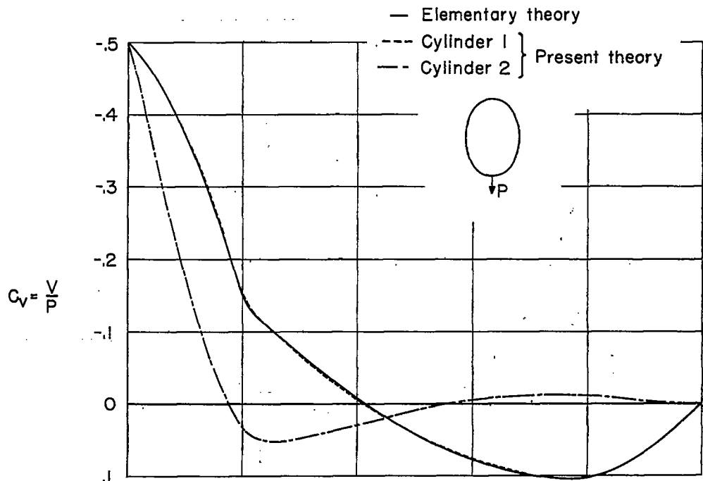
(a) Ring shear force.
