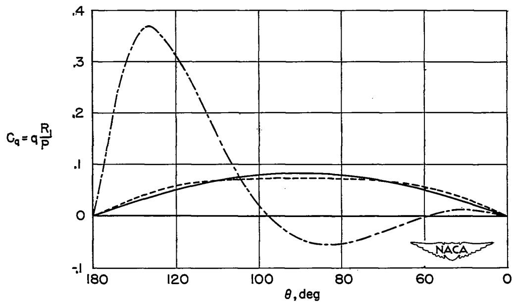
(b) Sheet shear flow.
