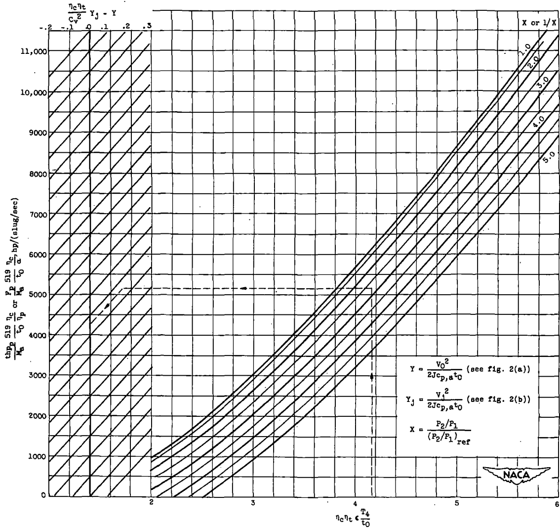
Figure 5. - Chart for determining thrust horsepower or shaft horsepower factors. (A 17- by 21-in. print of this chart (in two sections) is attached.)
