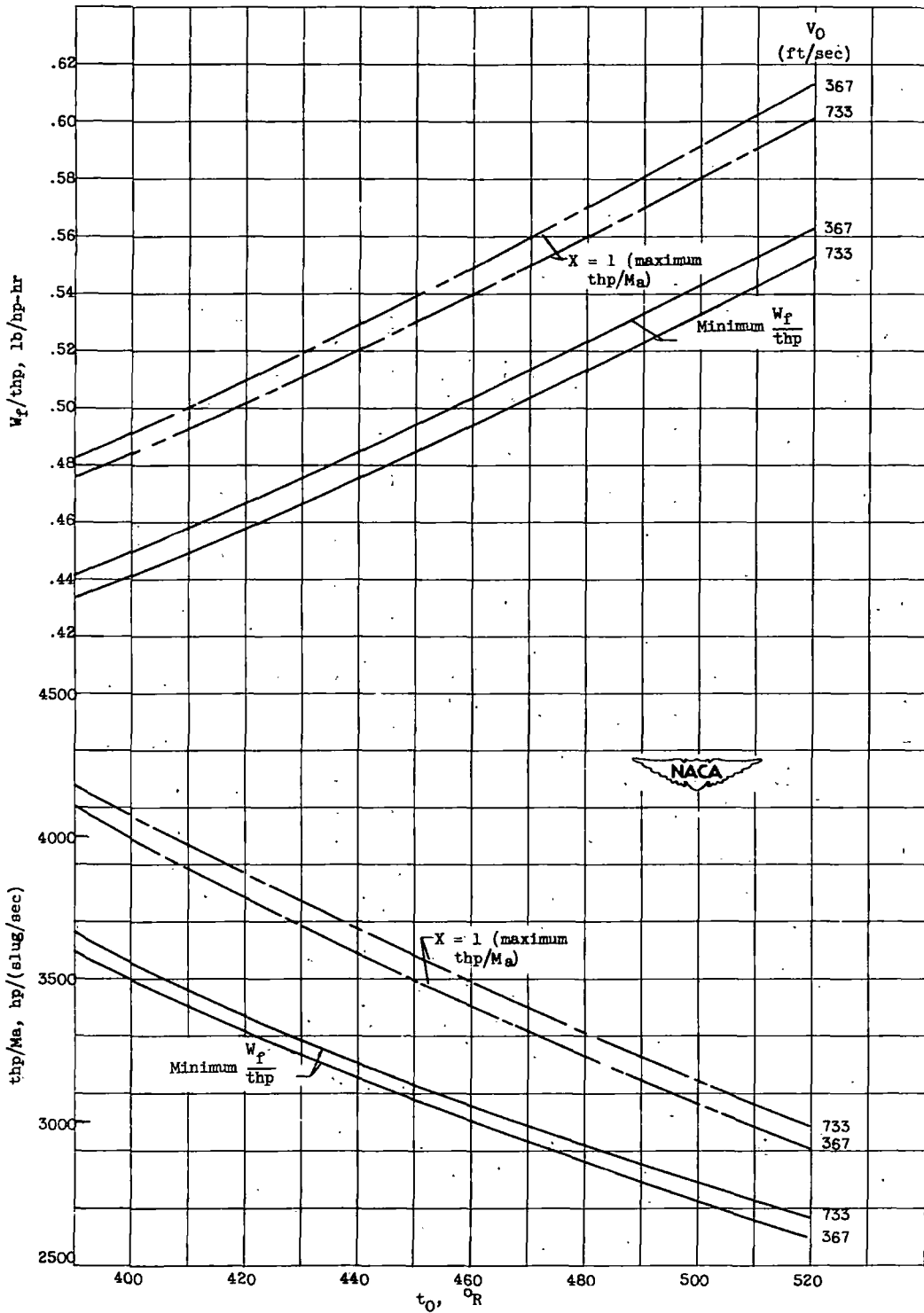
(a) Specific fuel consumption and thrust horsepower per unit mass rate of air flow.
