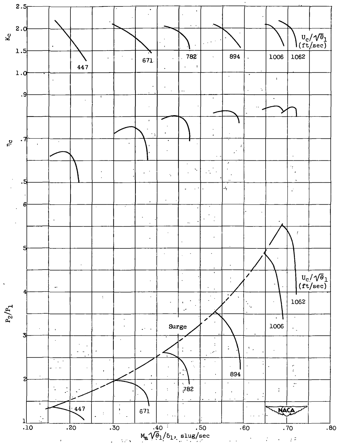
Figure 11. - Characteristics of axial-flow compressor.
