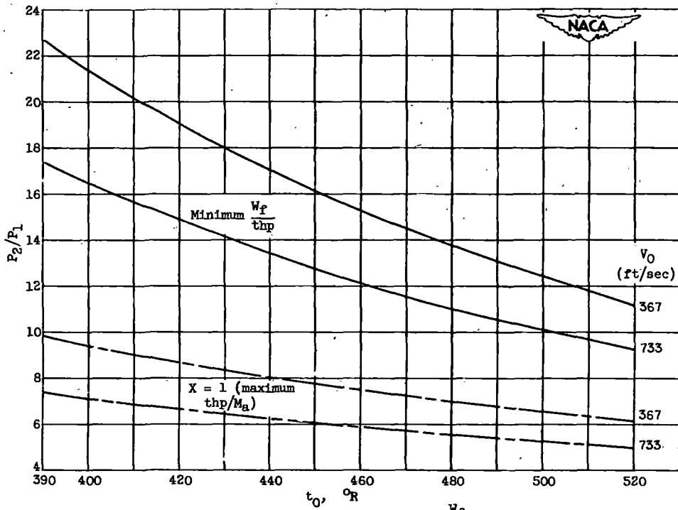
(b) Compressor pressure ratios for minimum \frac{W_f}{thp} and X = 1 .
