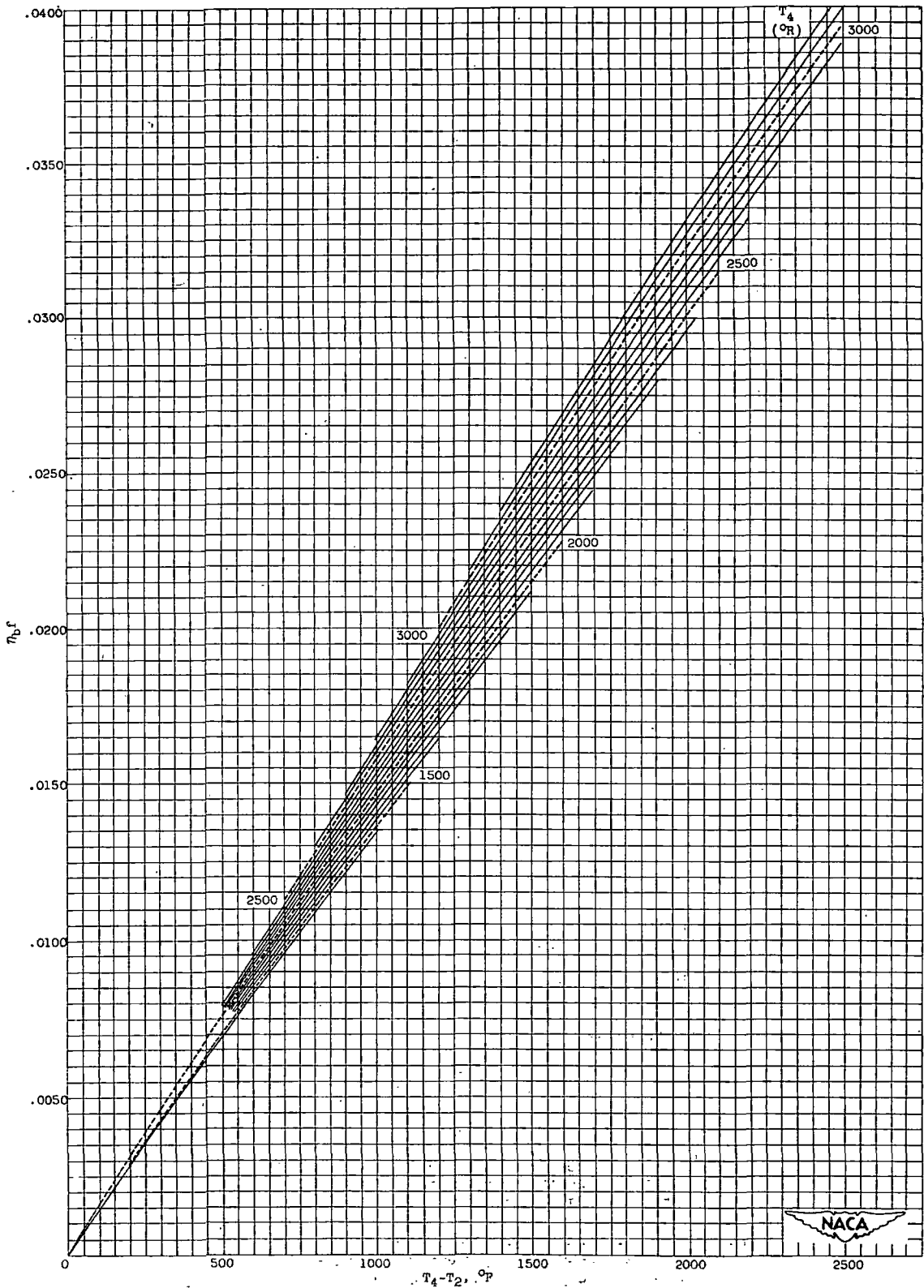
Figure 7. - Chart for determining f for various values of T_4 - T_2 and T_4 ; h , 18,900 Btu per pound; hydrogen-carbon ratio, 0.185. (A 15- by 21-in. print of this chart is attached.)
