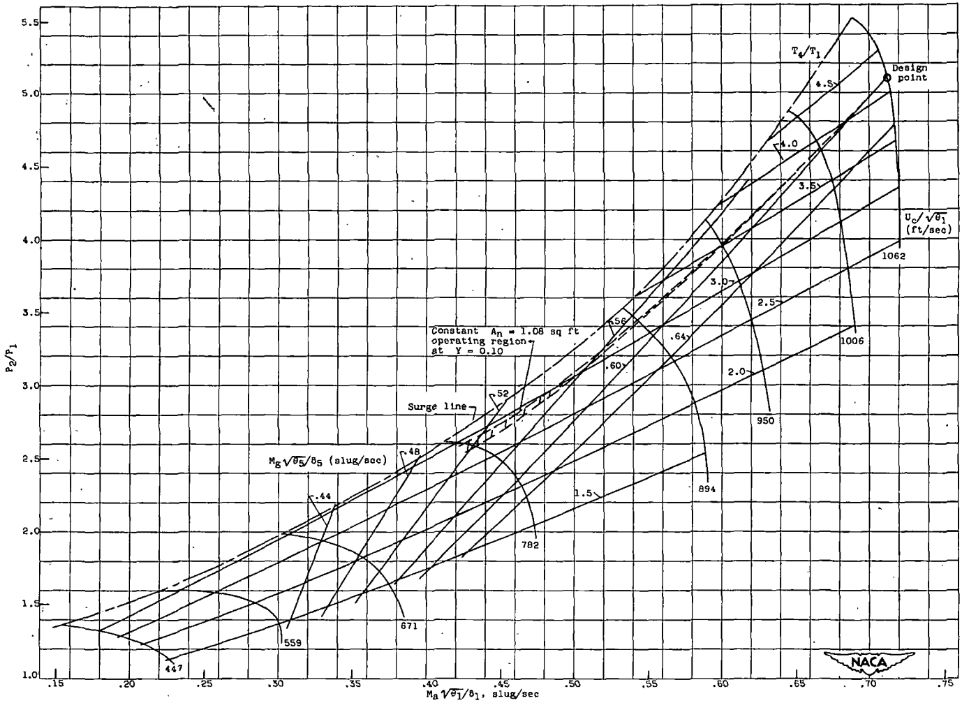
(a) Lines of constant T_4/T_1 and constant M_g \sqrt{\theta_5/\theta_5} .
