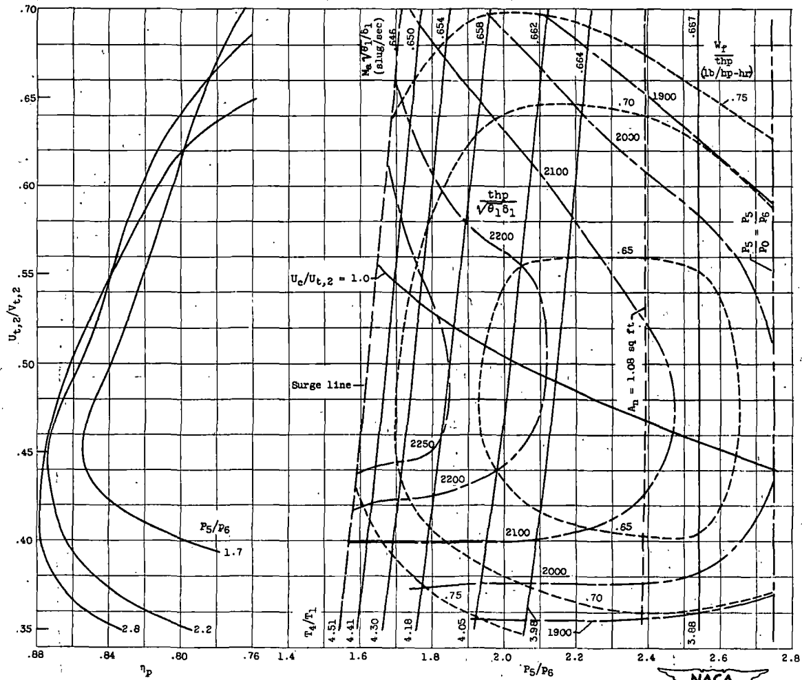
(c) U_c/\sqrt{\theta_1} , 1006 feet per second; Y , 0.1 (flight Mach number, 0.7).
