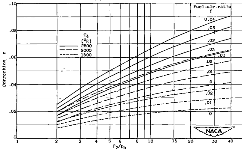
(c) Correction c.
