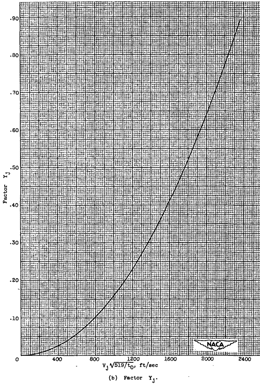
Figure 2. - Concluded. Charts for determining flight Mach number, compressor inlet total pressure, and factors Y and Y_j .
