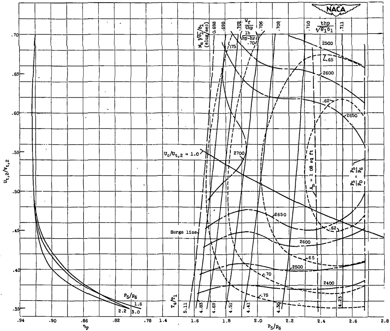
(b) U_c/\sqrt{\theta_1} , 1082 feet per second; Y , 0.06 (flight Mach number, 0.55).
