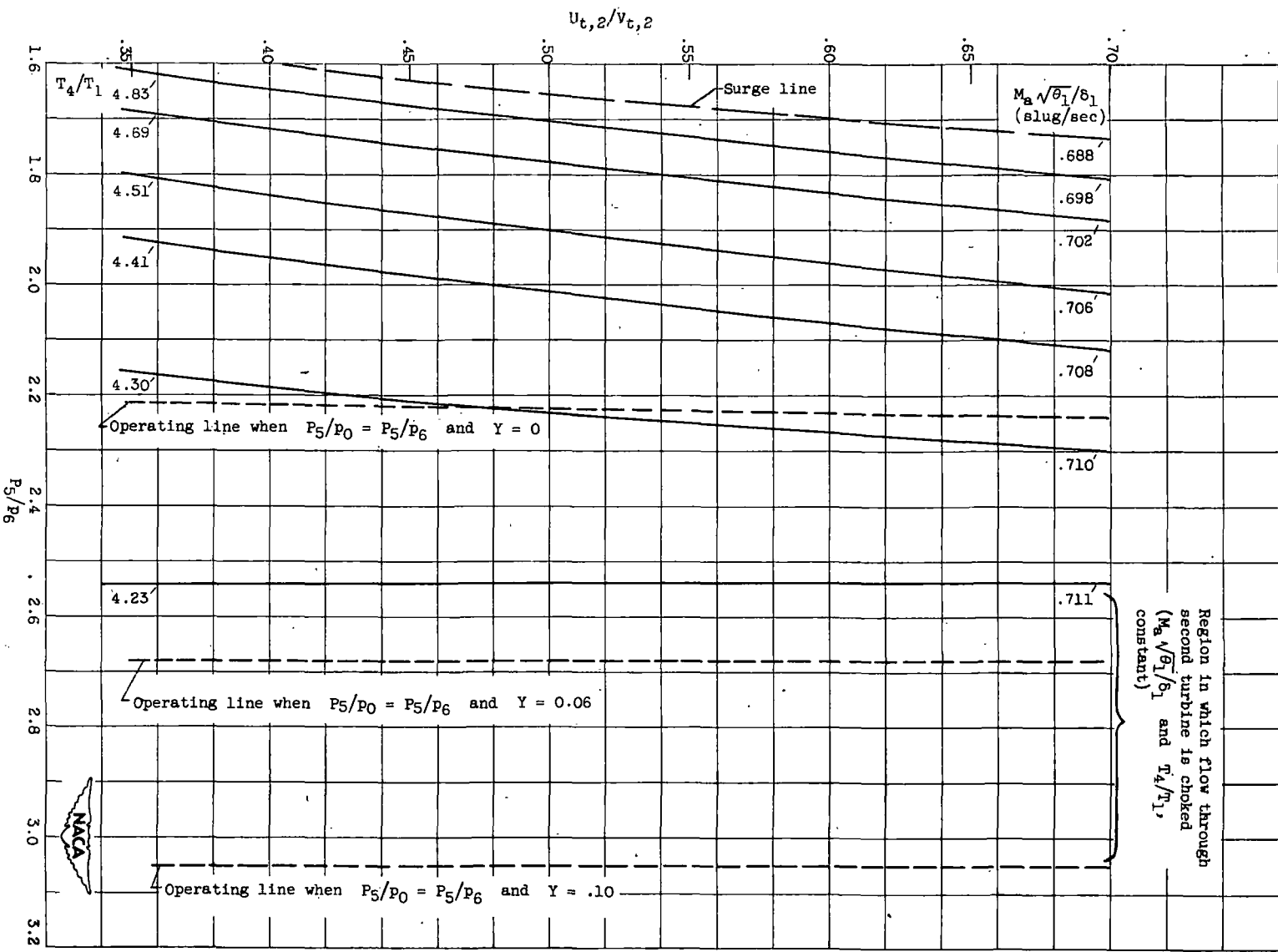
(a) U_c/\sqrt{\beta_1} , 1062 feet per second. Figure 16. - Relation between operating parameters of second turbine and gas generator.
