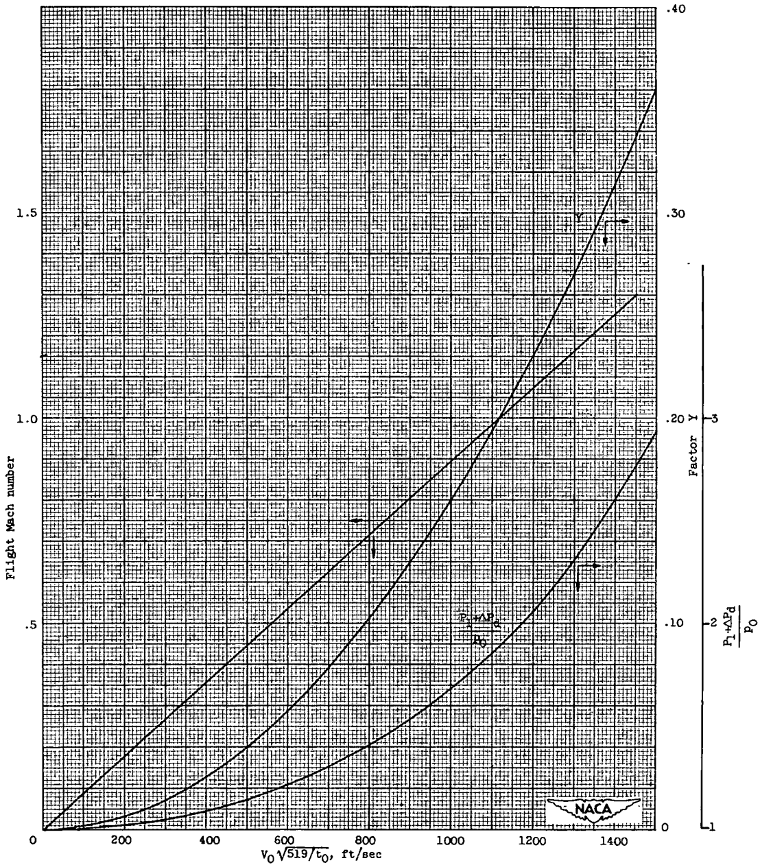
(a) Flight Mach number, factor Y , and \frac{P_1 + \Delta P_d}{P_0} .
