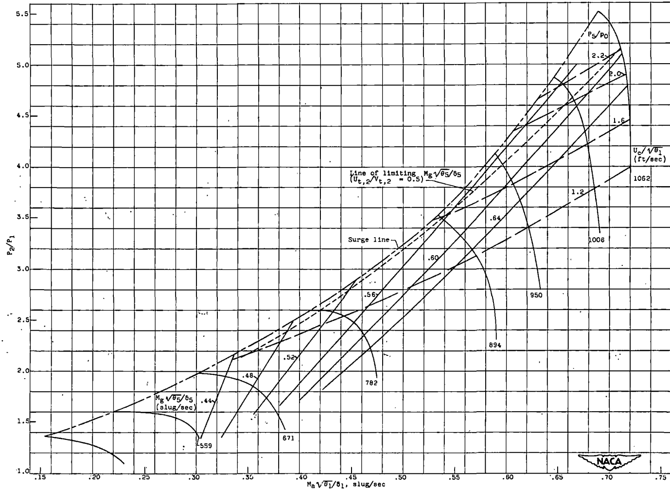
(c) Lines of constant P_5/P_0 and constant M_g \sqrt{\theta_5/\theta_5} ; \gamma, 0 (flight Mach number, 0).
