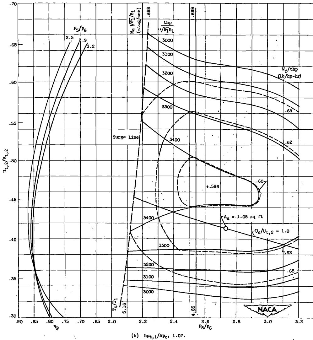
Figure 18. - Continued. Performance plots of matched turbine-propeller engine for various values of power output of first turbine to compressor power; U_c/\sqrt{\theta_1} , 1062 feet per second; Y , 0.1 (flight Mach number, 0.7); \eta_p , 0.86; C_v , 0.97; h , 18,900 Btu per pound; \Delta P_1/P_1 , 0.03; \Delta P_2/P_2 , 0.05.
