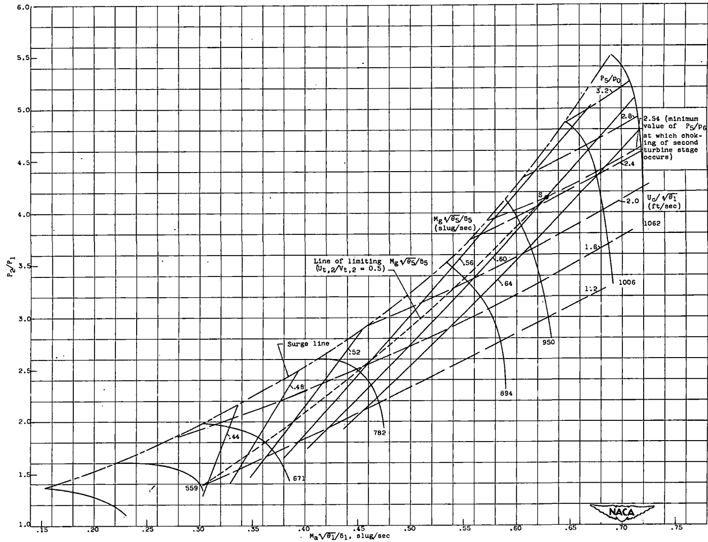
(b) Lines of constant P_5/P_0 and constant M_g \sqrt{\theta_5}/\theta_5 ; \gamma , 0.10 (flight Mach number, 0.7).
