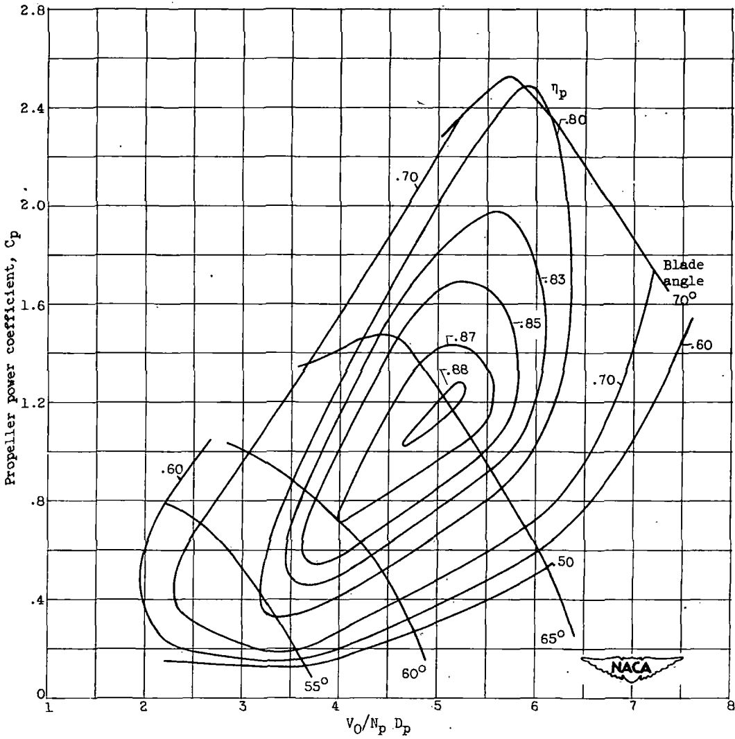
(b) Y, 0.1 (flight Mach number, 0.7).
