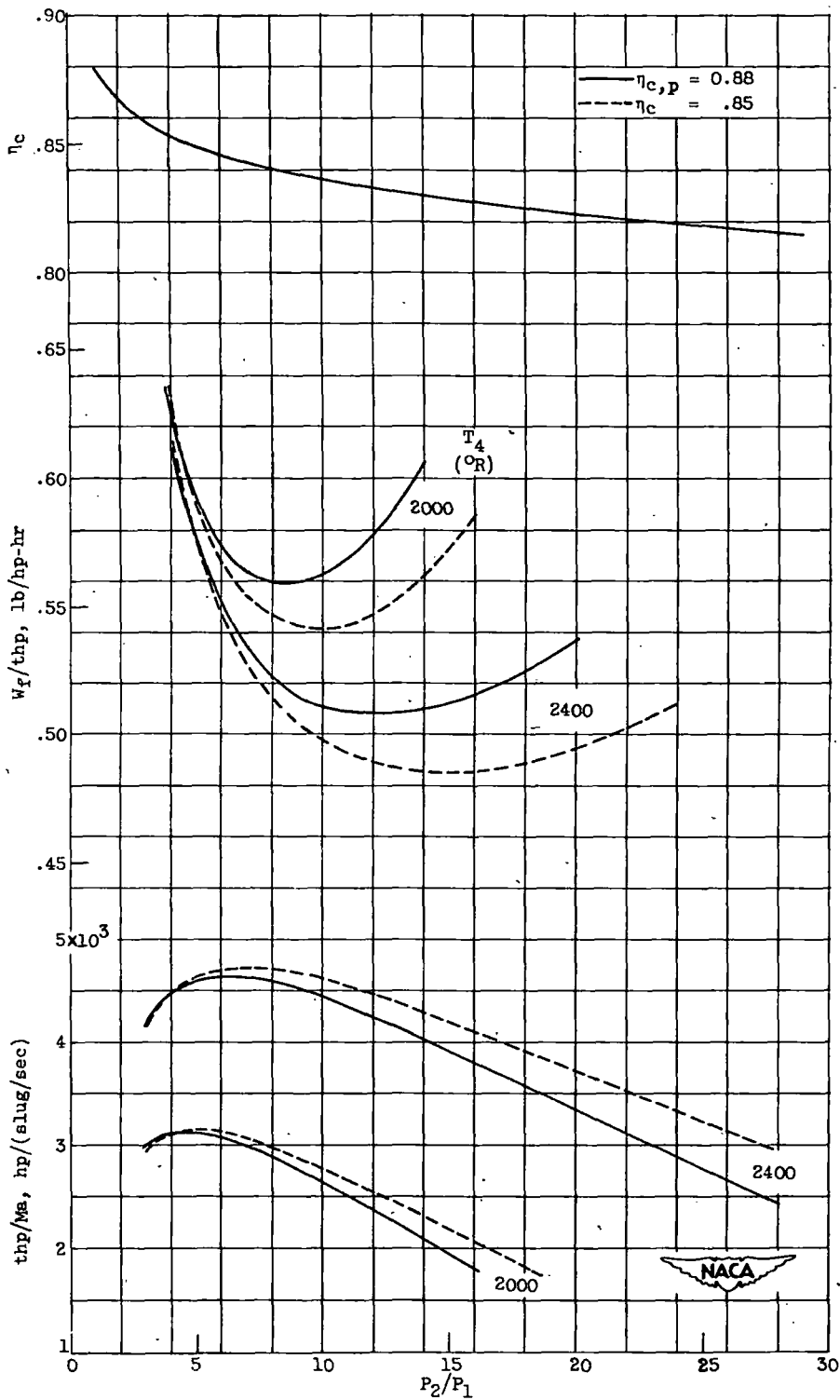
Figure 10. - Comparison of performance with constant \eta_c and with constant \eta_{c,p} at various compressor pressure ratios; V_0 , 733 feet per second; V_j , 902 feet per second; t_0 , 519° R; \eta_p , 0.85; \eta_t , 0.90; \eta_b , 0.96; C_v , 0.97; h , 18,900 Btu per pound; \epsilon , 1.00.
