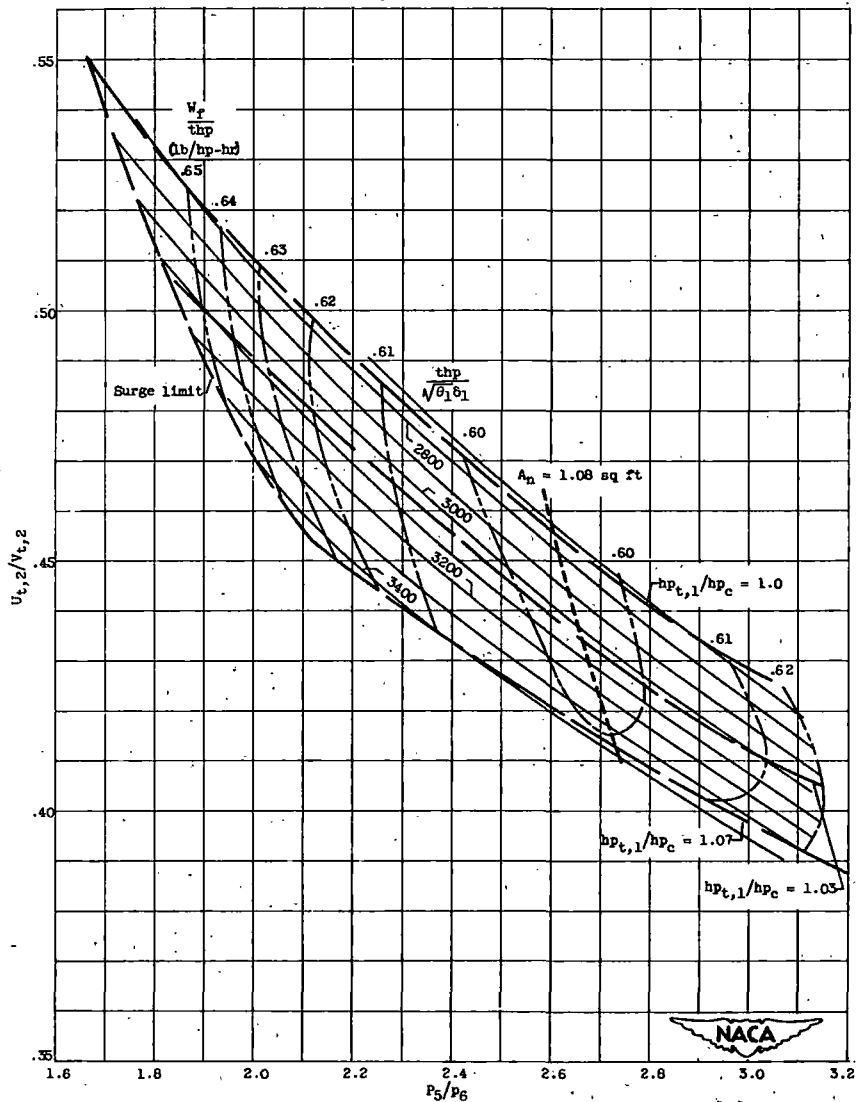
(c) hp_{t,1}/hp_c , 1.00 to 1.07; U_c/U_{t,2} = 1.0 .
