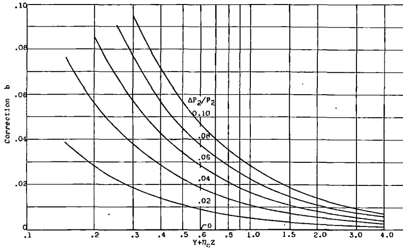
(b) Correction b.
