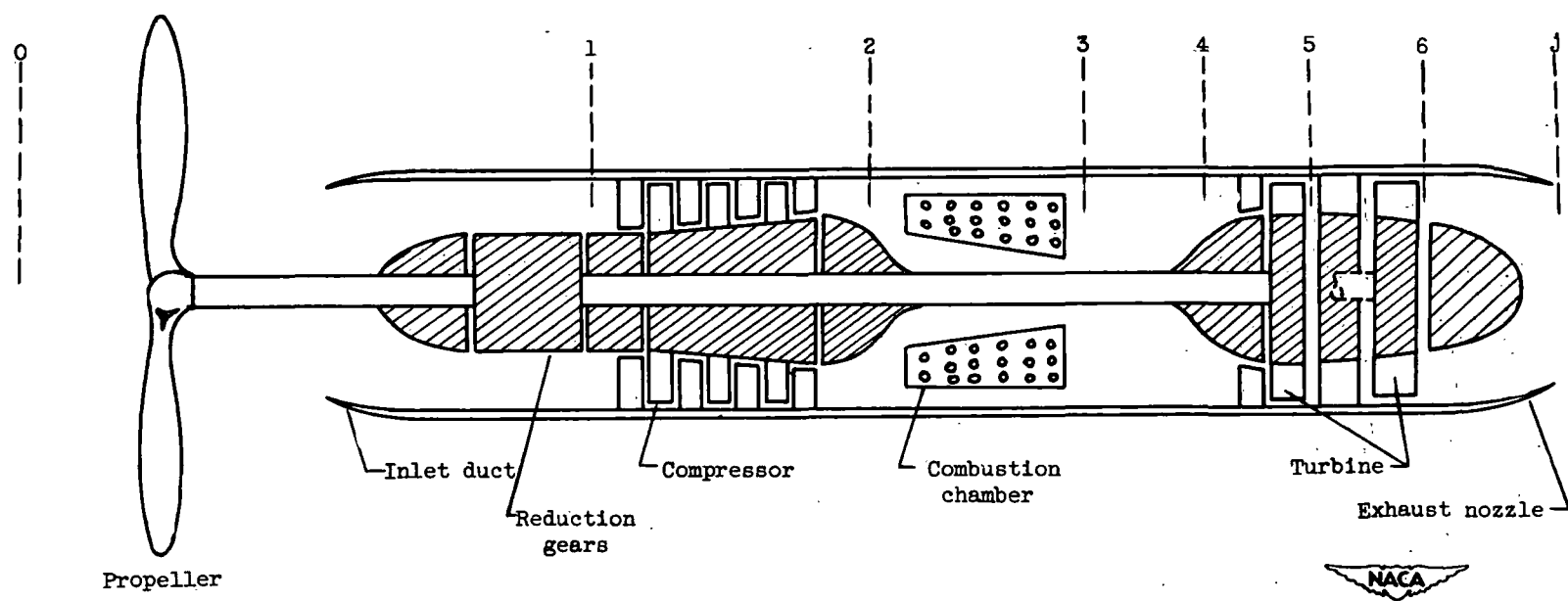
Figure 1. - Schematic diagram of turbine-propeller engine.
