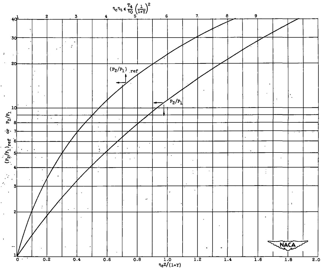
Figure 4. - Chart for determining (P_2/P_1)_{ref} for various values of \eta_c \eta_t \leq \frac{T_4}{T_0} \left(\frac{1}{1+Y}\right)^2 and for determining \frac{\eta_c Z}{1+Y} for various values of P_2/P_1 . (A 17- by 19-in. print of this chart is attached.)
