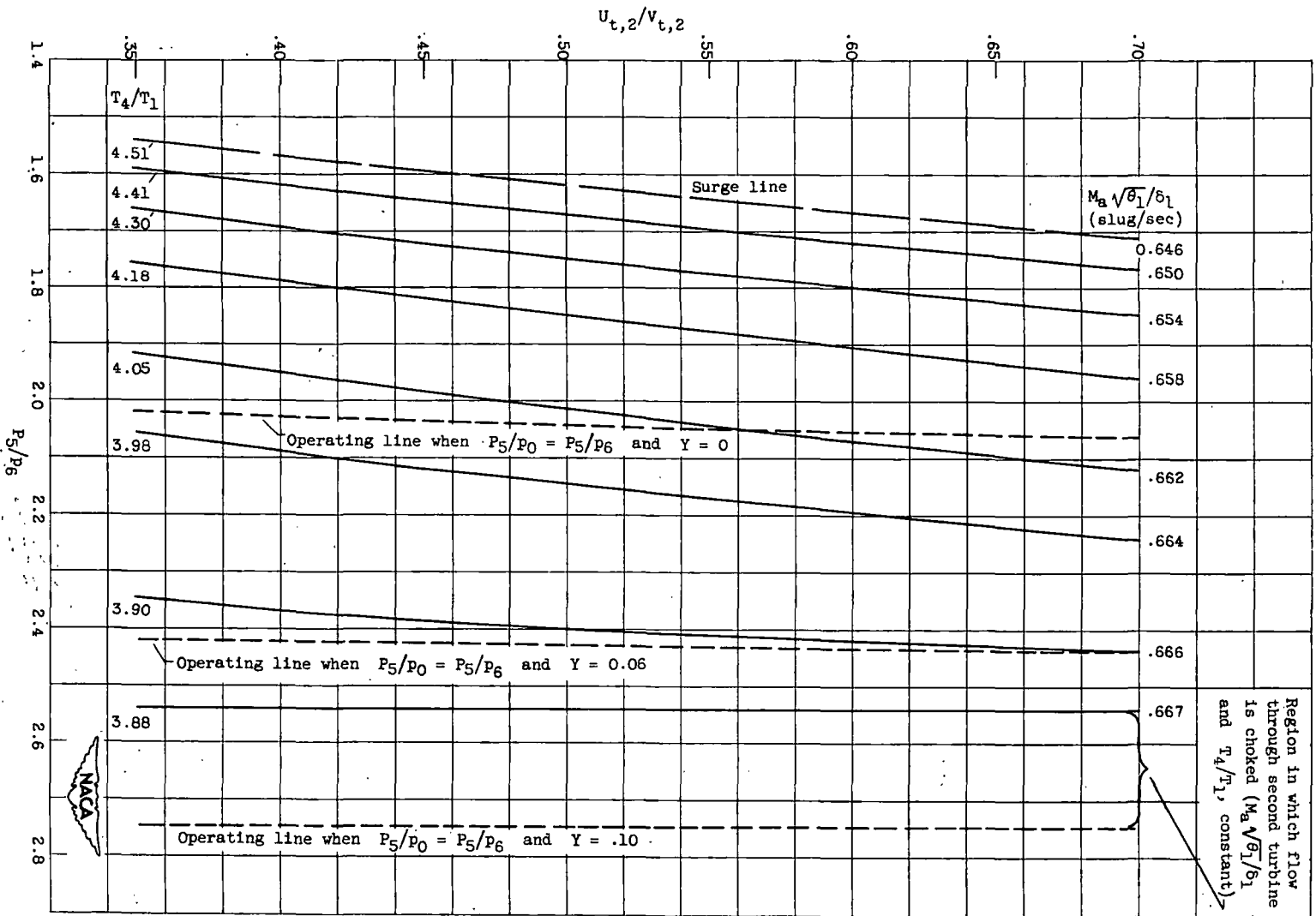
Figure 16. - Concluded. Relation between operating parameters of second turbine and gas generator.
