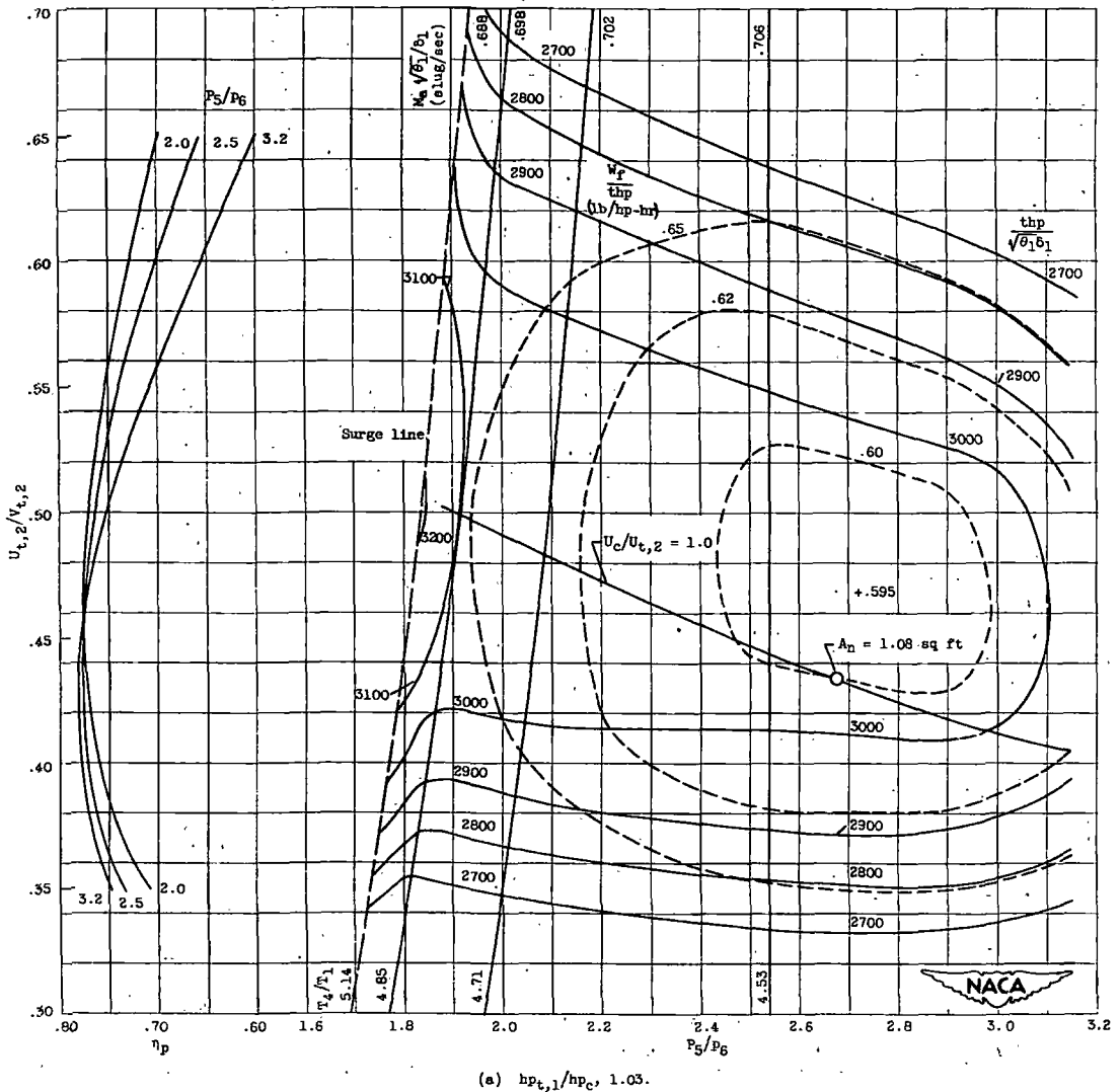
Figure 18. - Performance plots of matched turbine-propeller engine for various values of power output of first turbine to compressor power; U_c/\sqrt{\theta_1} , 1062 feet per second; Y , 0.1 (flight Mach number, 0.7); \eta_p , 0.96; C_v , 0.97; h , 18,900 Btu per pound; \Delta P_d/P_1 , 0.03; \Delta P_2/P_2 , 0.05.
