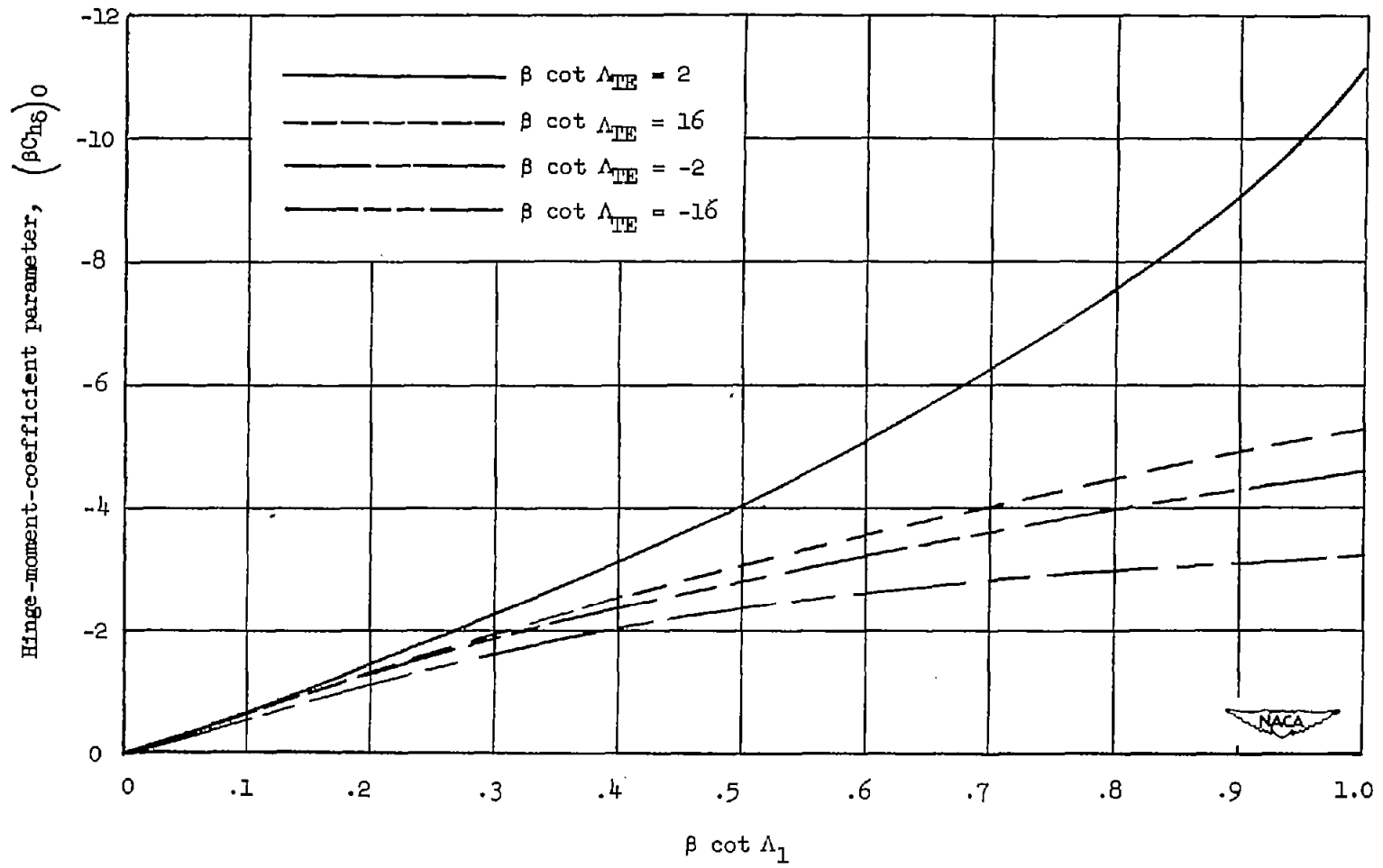
Figure 7.- Variation of (\beta C_{h8})_0 with \beta \cot A_1 and \beta \cot A_{TE} for the basic configuration.
