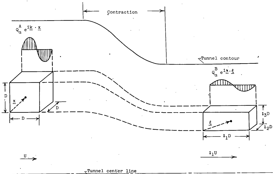
(b) Stream tube geometry.
