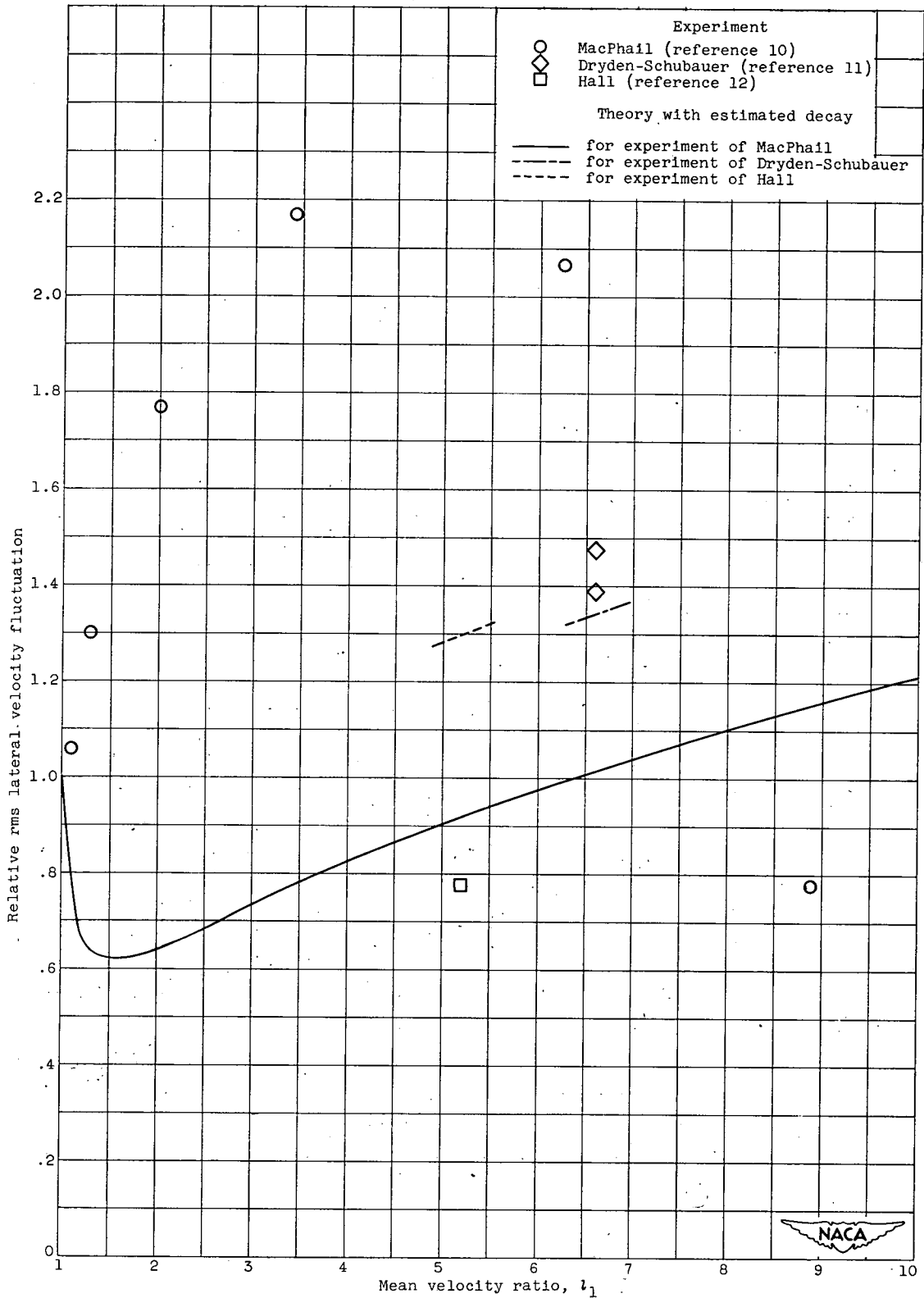
Figure 8. - Comparison of predicted axisymmetric contraction effect with experiment for lateral component of turbulence, with decay allowed for in first approximation. Initial isotropic turbulence assumed.
