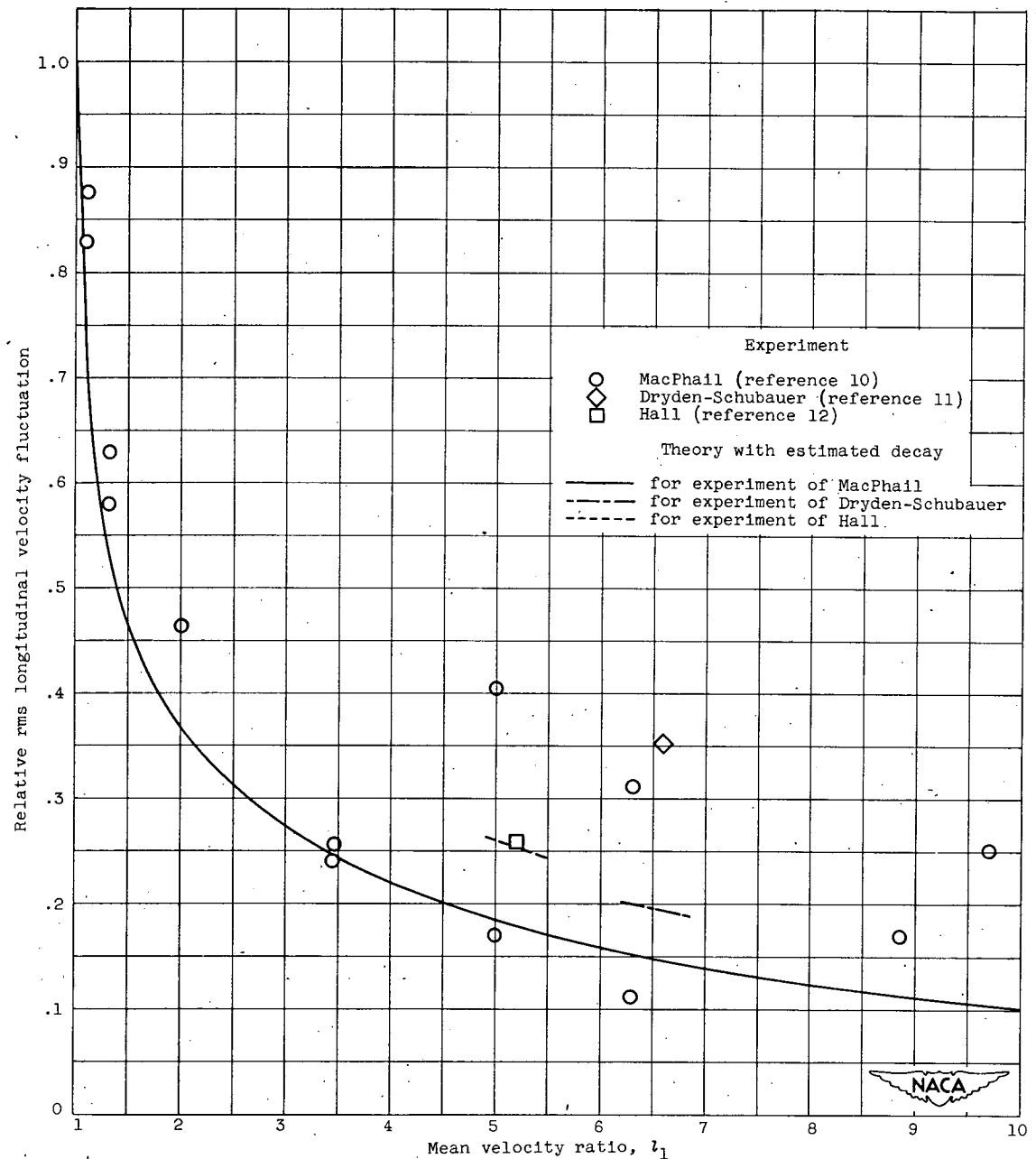
Figure 7. - Comparison of predicted axisymmetric contraction effect with experiment for longitudinal component of turbulence, with decay allowed for in first approximation. Initial isotropic turbulence assumed.
