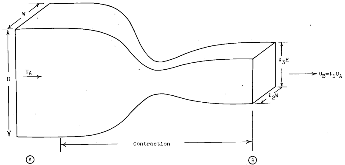
(a) Tunnel geometry.
