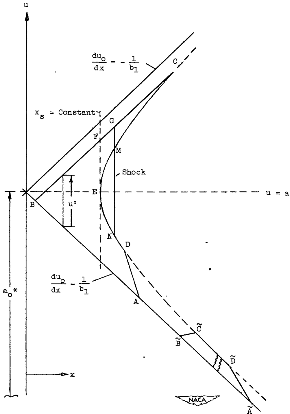
Figure 1.- Distortion of expansion pulse near M_0 = 1 in the velocity plane.
