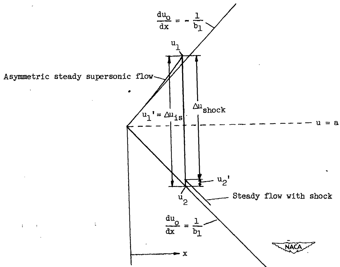
Figure 2.- Conditions for stationary trailing shock.
