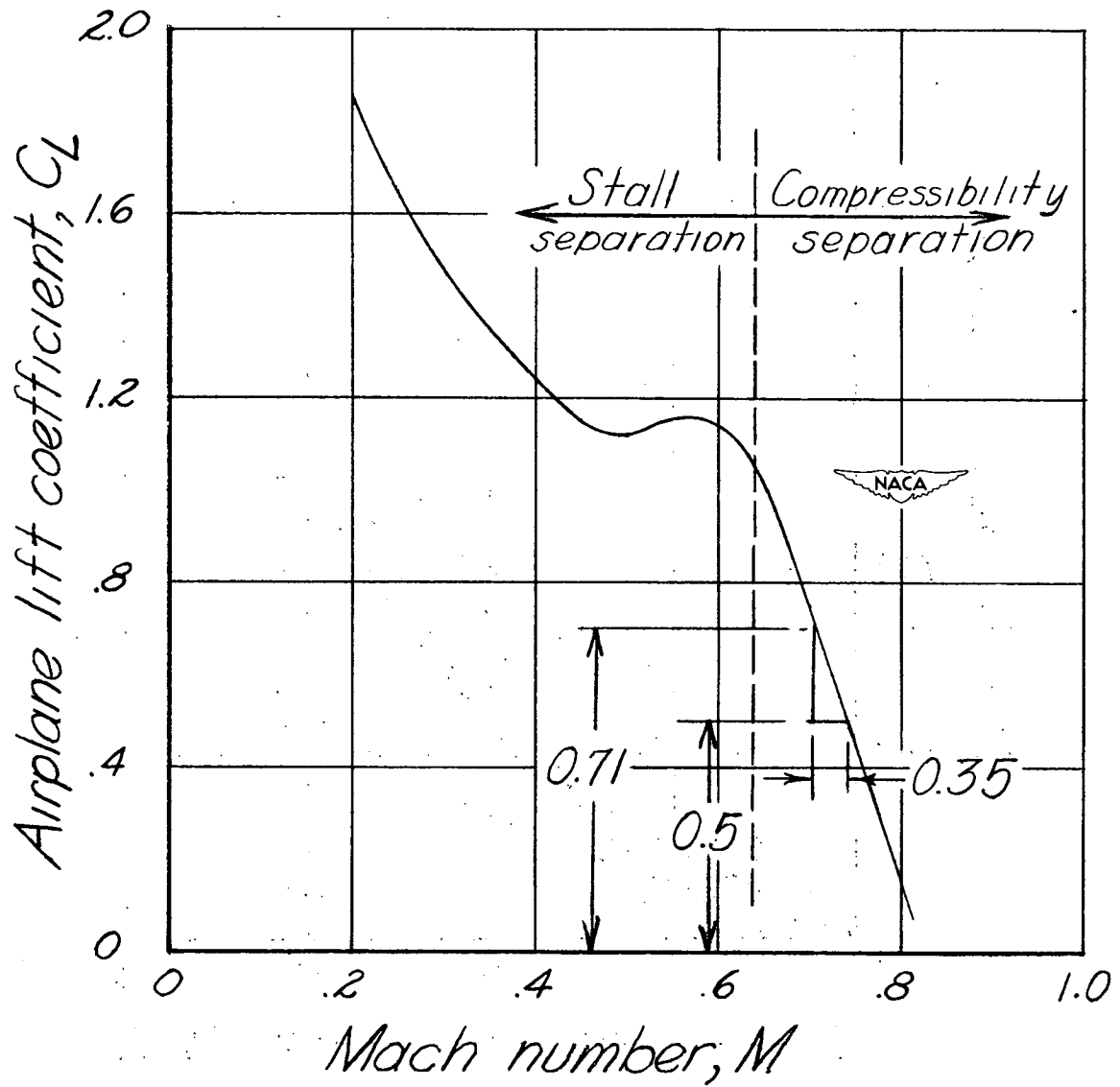
Figure 1.- Typical buffeting boundary for high-speed fighter airplane 1.
