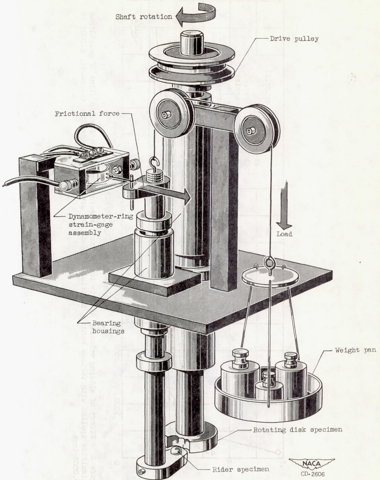
Figure 2. - Schematic diagram of endurance apparatus.
