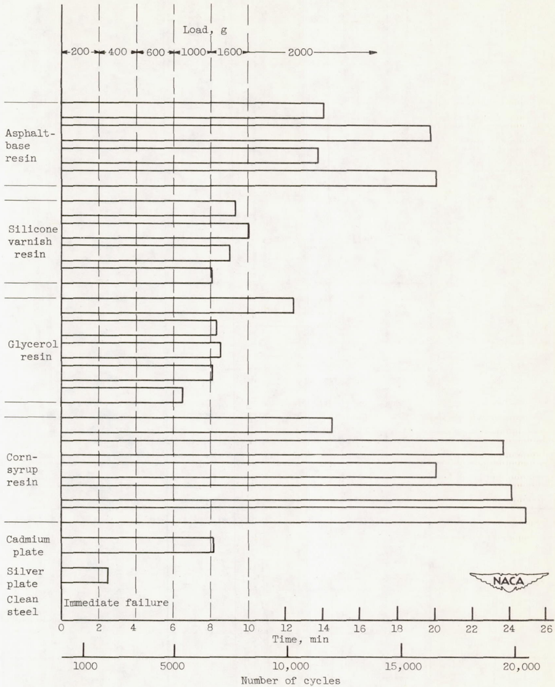
Figure 4. - Endurance tests, showing total number of cycles to failure of solid-film lubricants of MoS 2 using four different resin forming liquids. Sliding velocity, 425 feet per minute.
