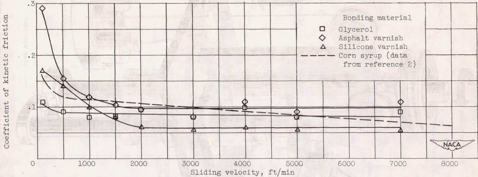
Figure 3. - Effect of sliding velocity on friction of steel specimens coated with solid films of molybdenum disulfide applied with various bonding materials. Load, 269 grams; approximate film thickness, 0.0002 to 0.0005 inch.
