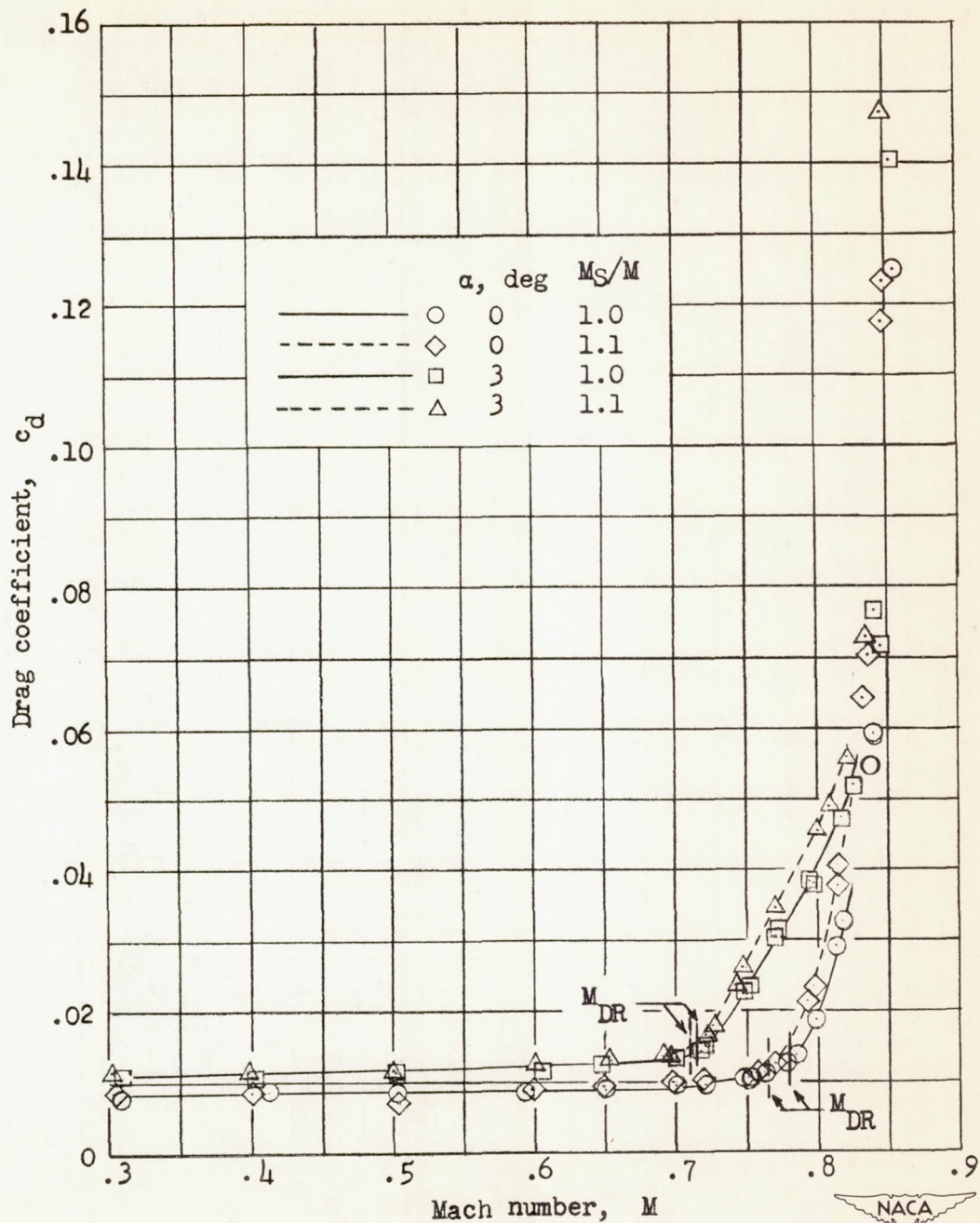
(b) Wing panel with nacelle symmetrically aligned.
