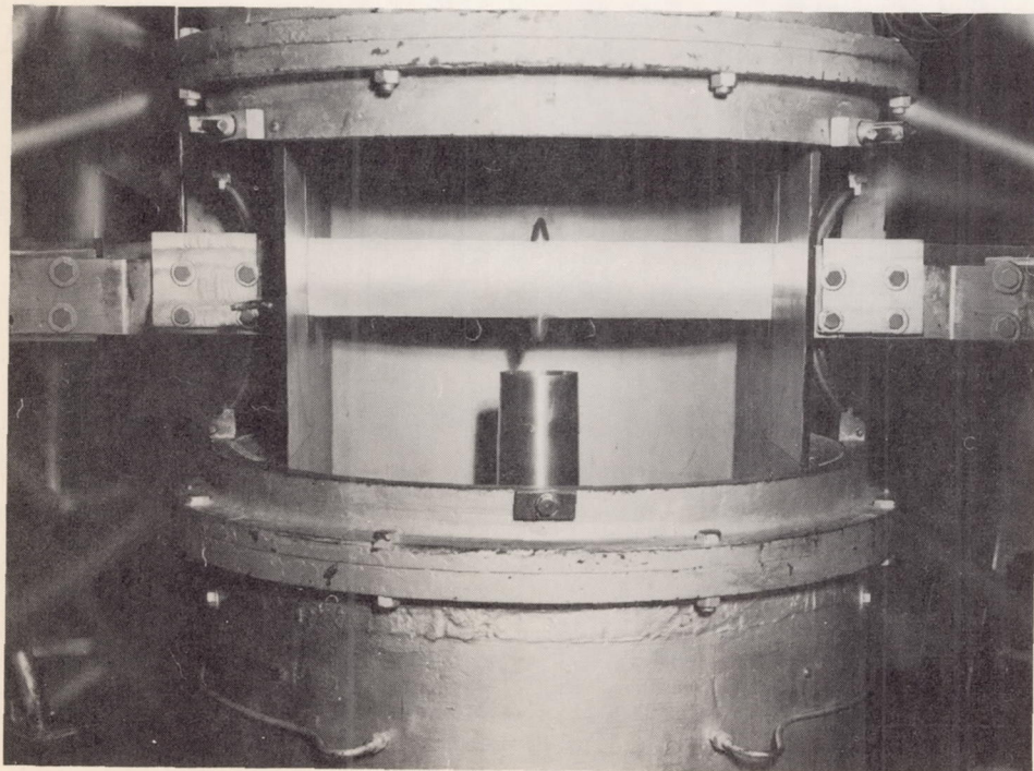
(b) Underslung configuration mounted in Langley 24-inch high-speed tunnel.
