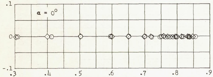
(b) Wing panel with nacelle symmetrically aligned.
