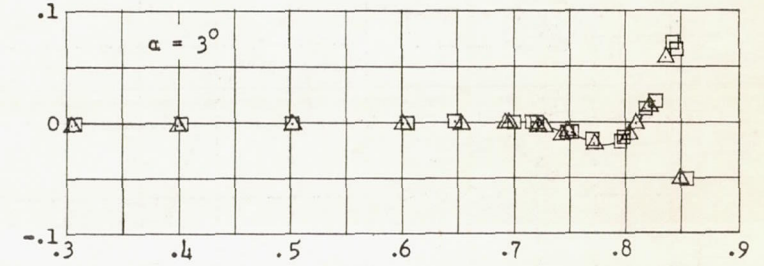
(b) Wing panel with nacelle symmetrically aligned.
