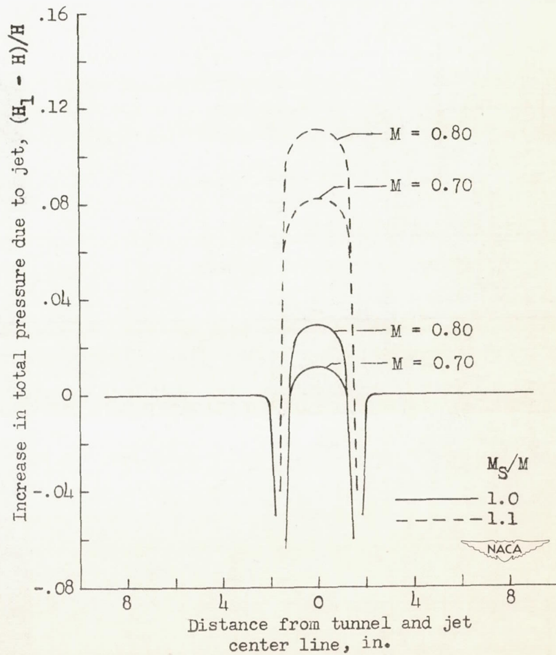
Figure 2.- Effect of jet on static-pressure distribution and total-pressure distribution across the Langley 24-inch high-speed tunnel at the quarter-chord position of the wing panel.
