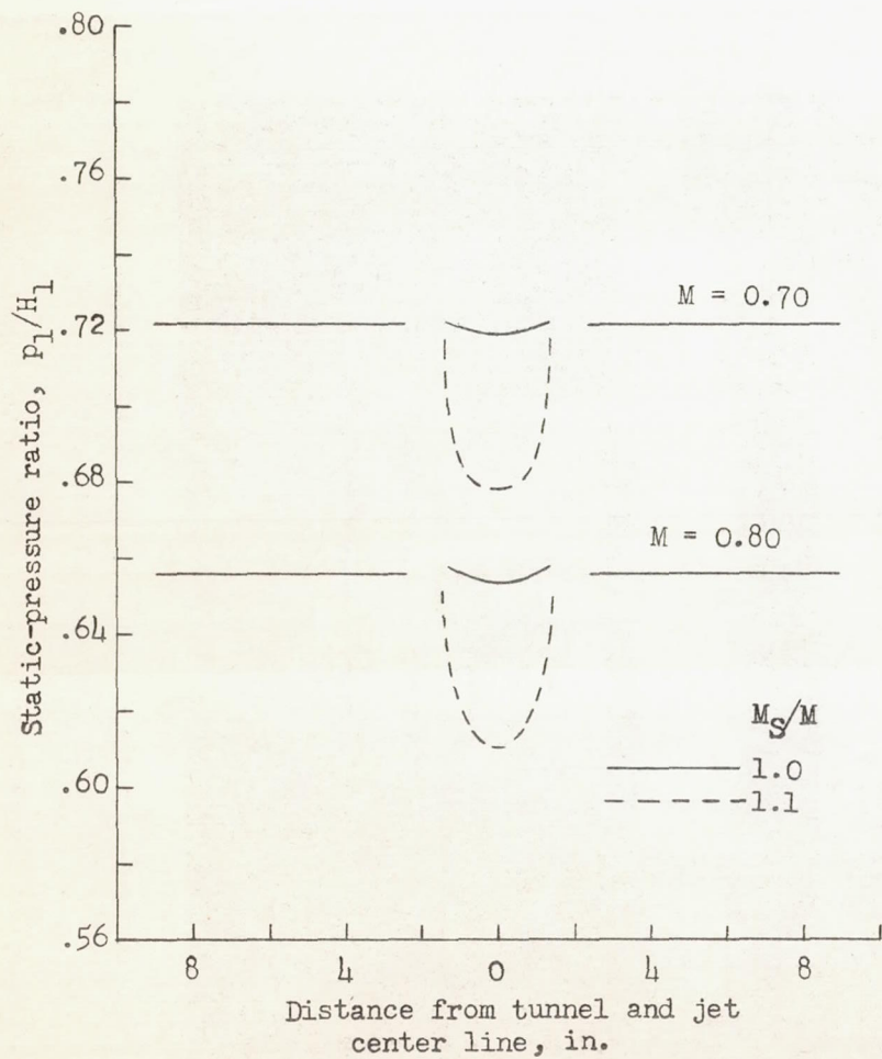
Figure 2.- Effect of jet on static-pressure distribution and total-pressure distribution across the Langley 24-inch high-speed tunnel at the quarter-chord position of the wing panel.
