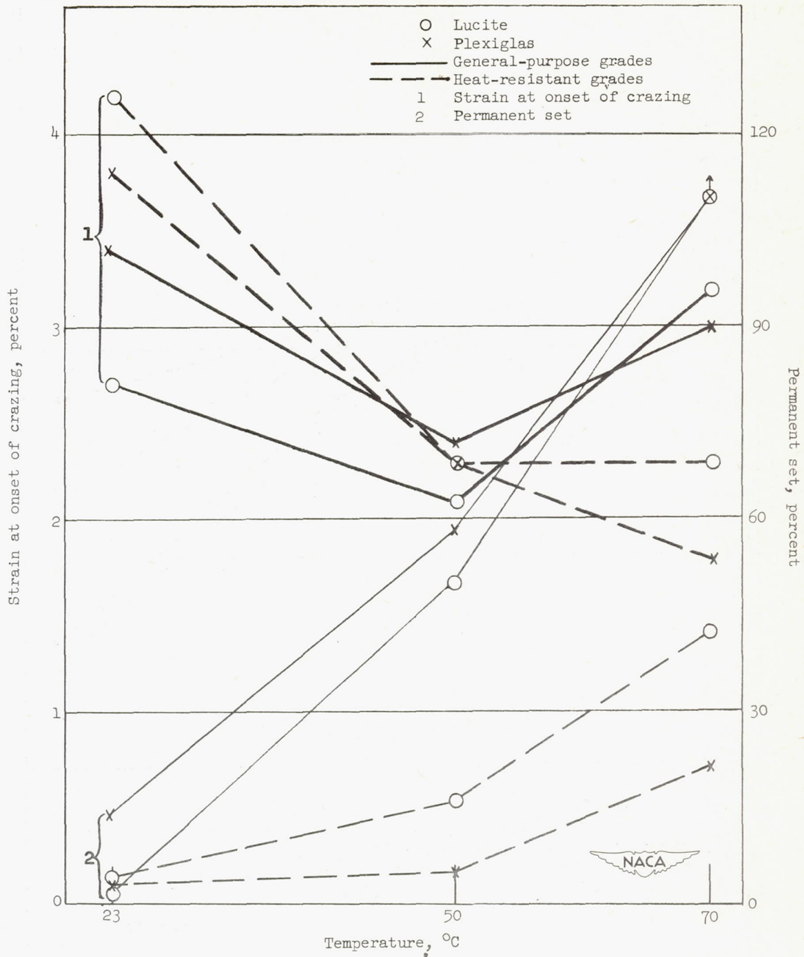
Figure 5.- Variation of strain at onset of crazing and permanent set with temperature for acrylic plastics.
