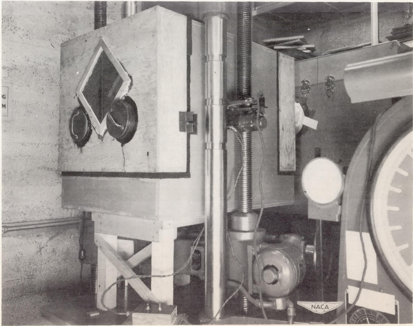
Figure 1.- Front view of tensile test enclosure in place in testing machine; conditioning unit can be seen at right.
