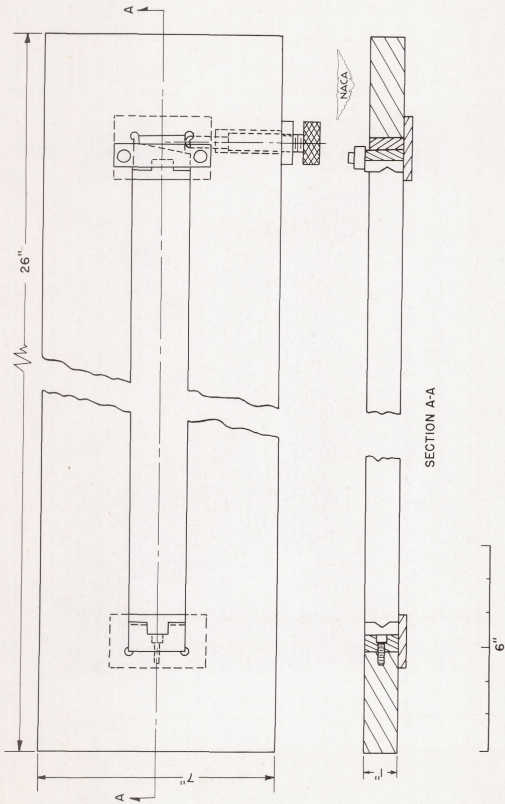
Figure 17.- Testing jig.
