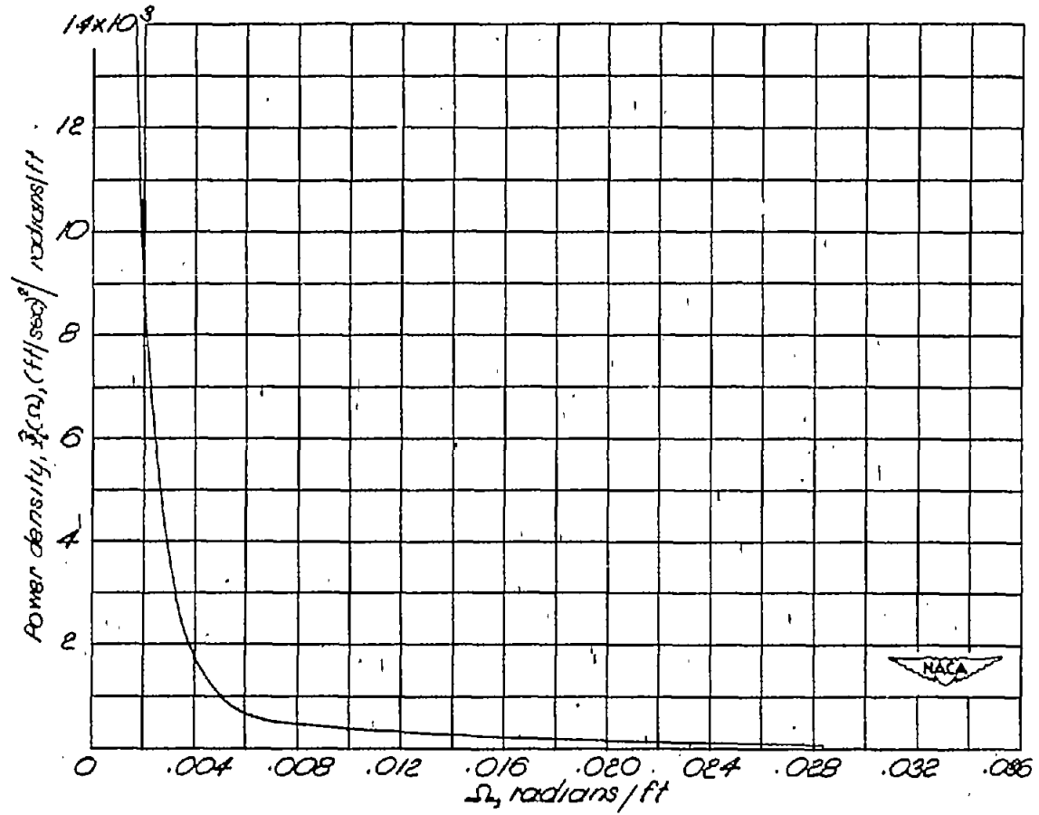
Figure 2.- Normalized power-spectral-density function for atmospheric vertical gust velocity \hat{\phi}_1(\Omega) .
