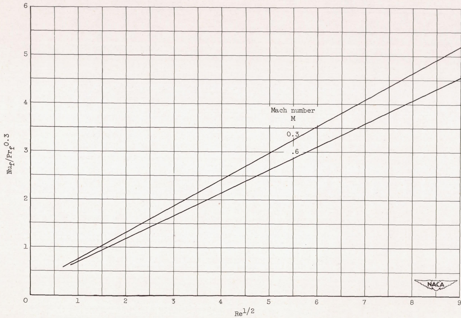
Figure 34. - Calibration curves for hot-wire anemometer probes.
