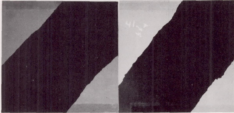
(a) Sample A; etched tungsten; nominal diameter, 0.0002 inch; actual diameter, 0.000248 inch; X5064.
