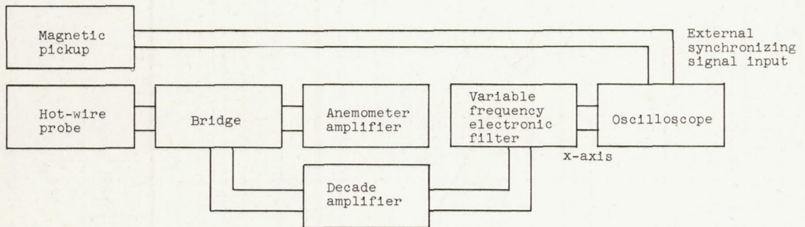
(b) Velocity profile measurements.
