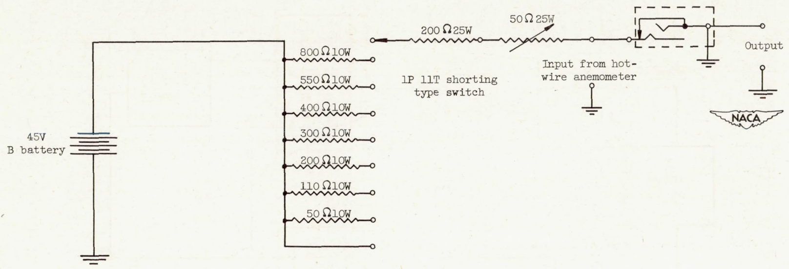
Figure 13. - Auxiliary current supply for hot-wire anemometer.
