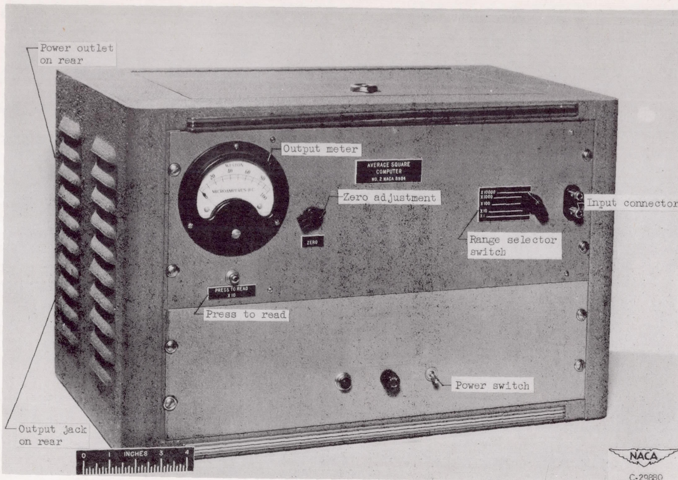
Figure 30. - Average-square computer.
