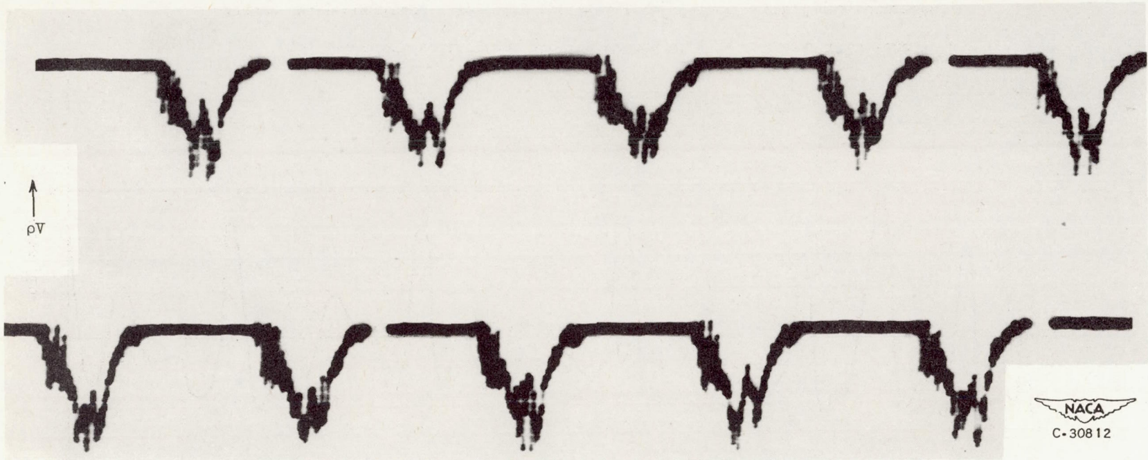
Figure 27. - Hot-wire signals from a single-stage axial-flow compressor with five rotating stall regions.
