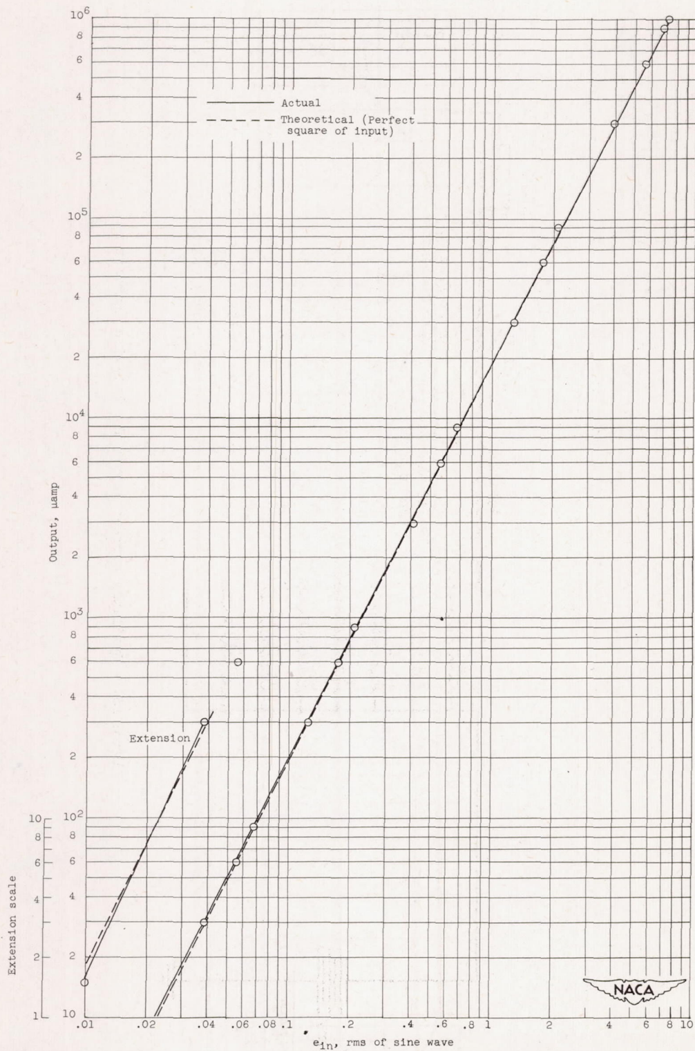
Figure 12. - Calibration for average-square computer number 2.
