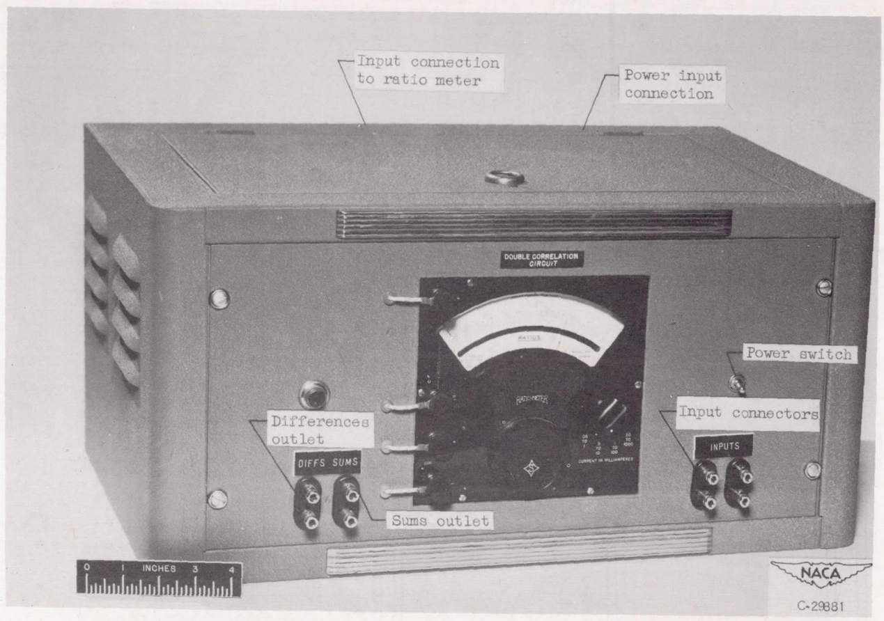
Figure 32. - Double-correlation instrument.
