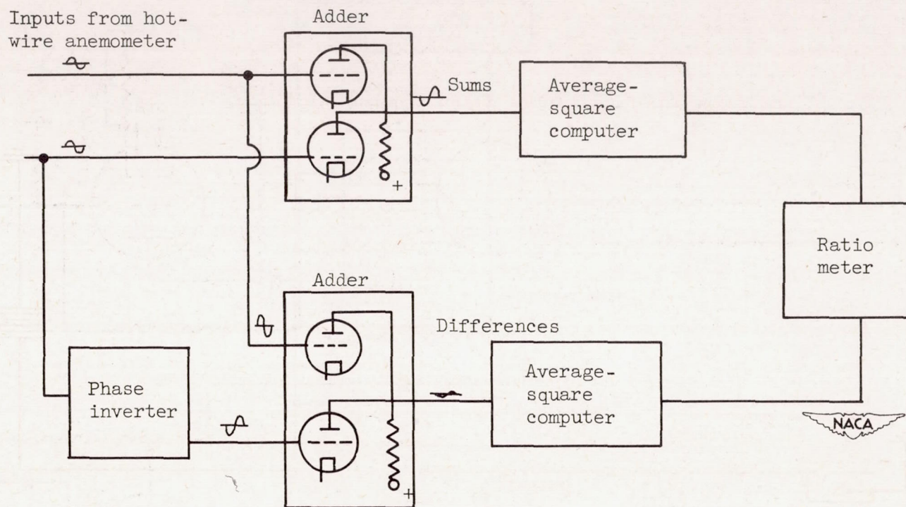
Figure 14. - Simplified diagram of double-correlation computer.
