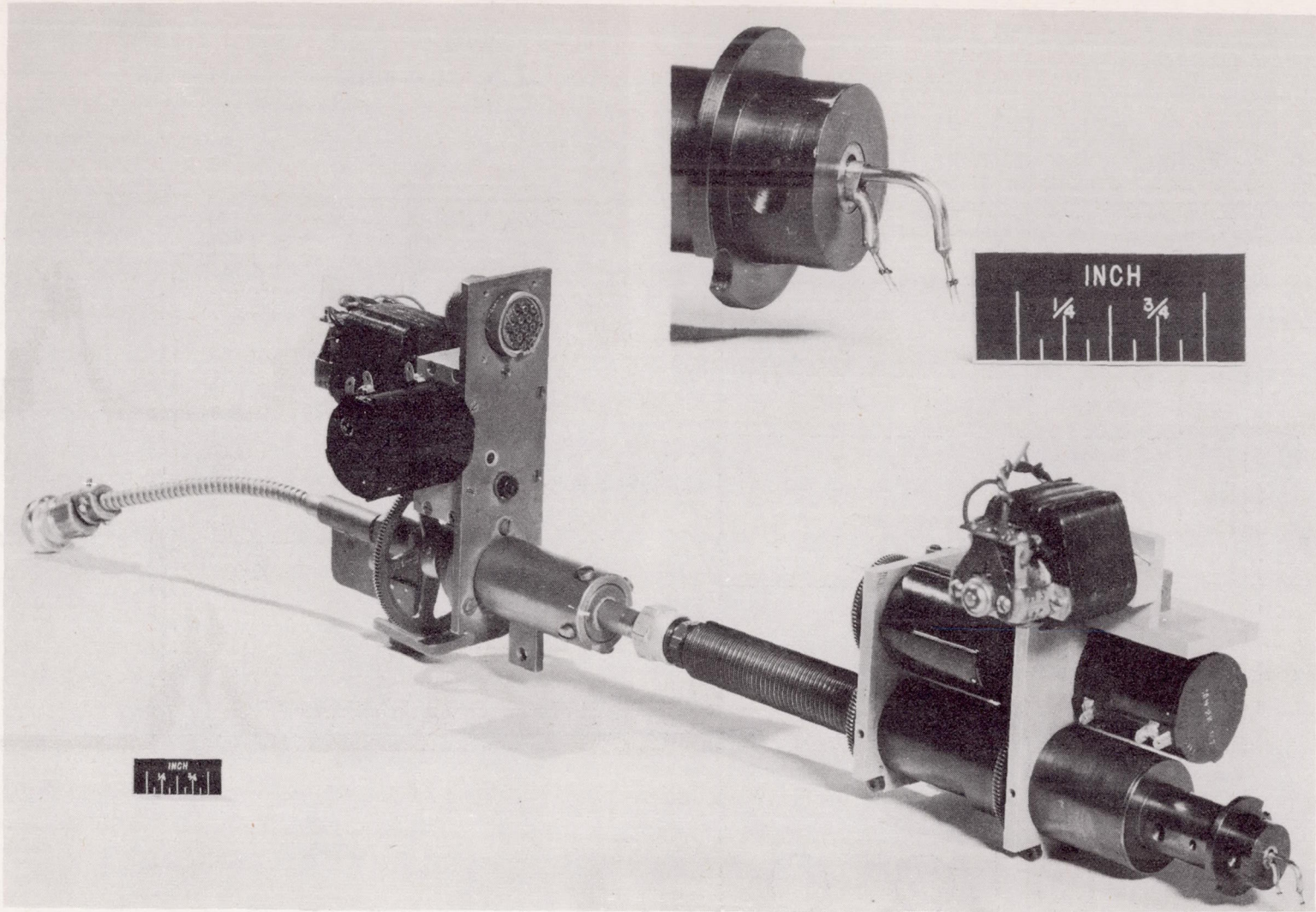
Figure 28. - Double-correlation probe and actuators.
