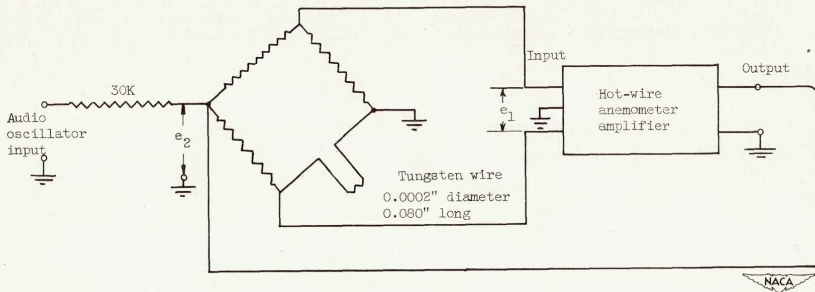
Figure 7. - Diagram for frequency-response measurements of hot-wire anemometer.
