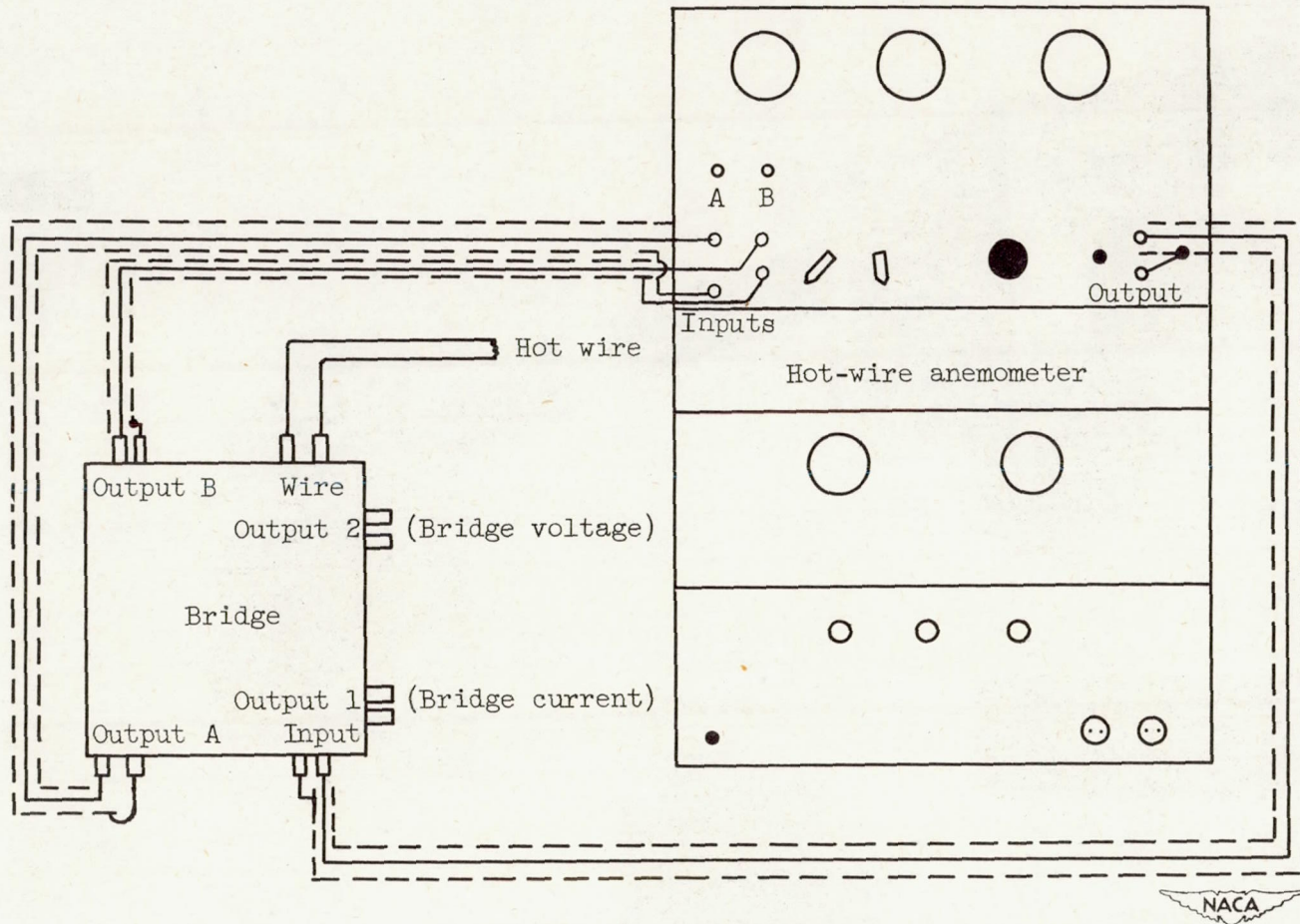
Figure 29. - Hot-wire anemometer to bridge connections.
