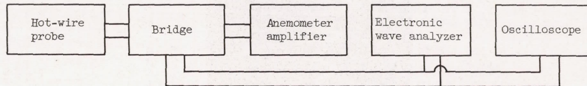
(f) Spectrum of turbulence measurements (method 2).
