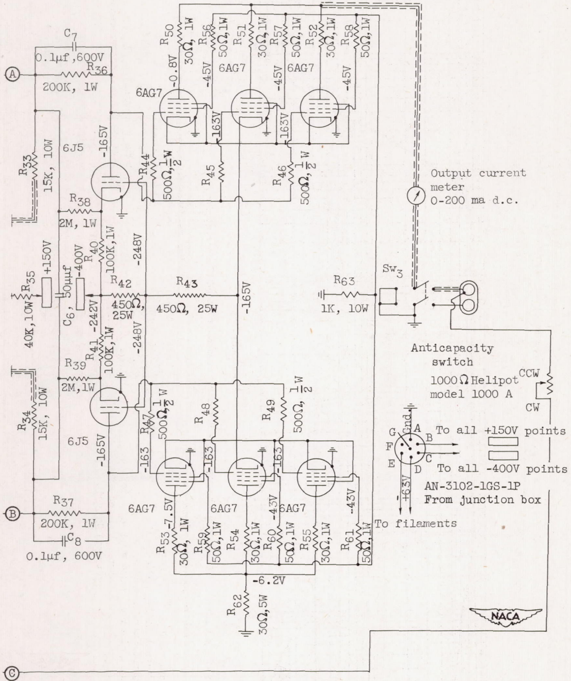
Figure 2. - Hot-wire anemometer with d-c amplifier.
