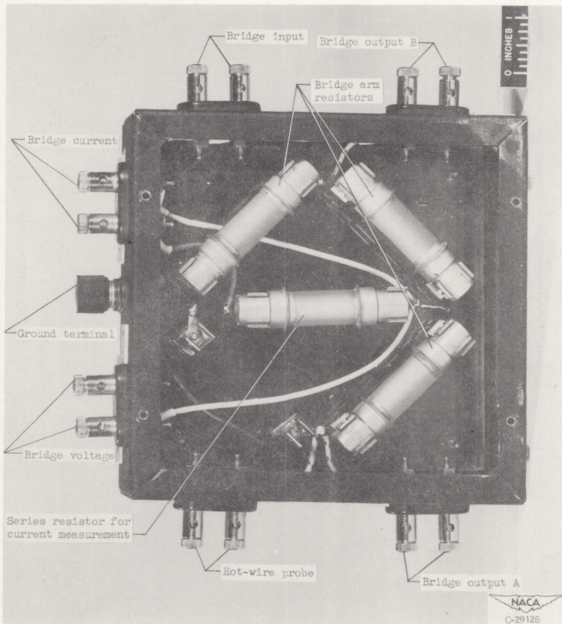
Figure 5. - Hot-wire bridge.
