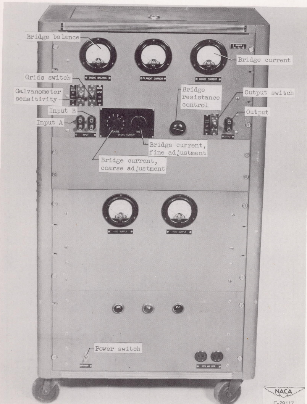
Figure 1. - Constant-temperature hot-wire anemometer amplifier.
