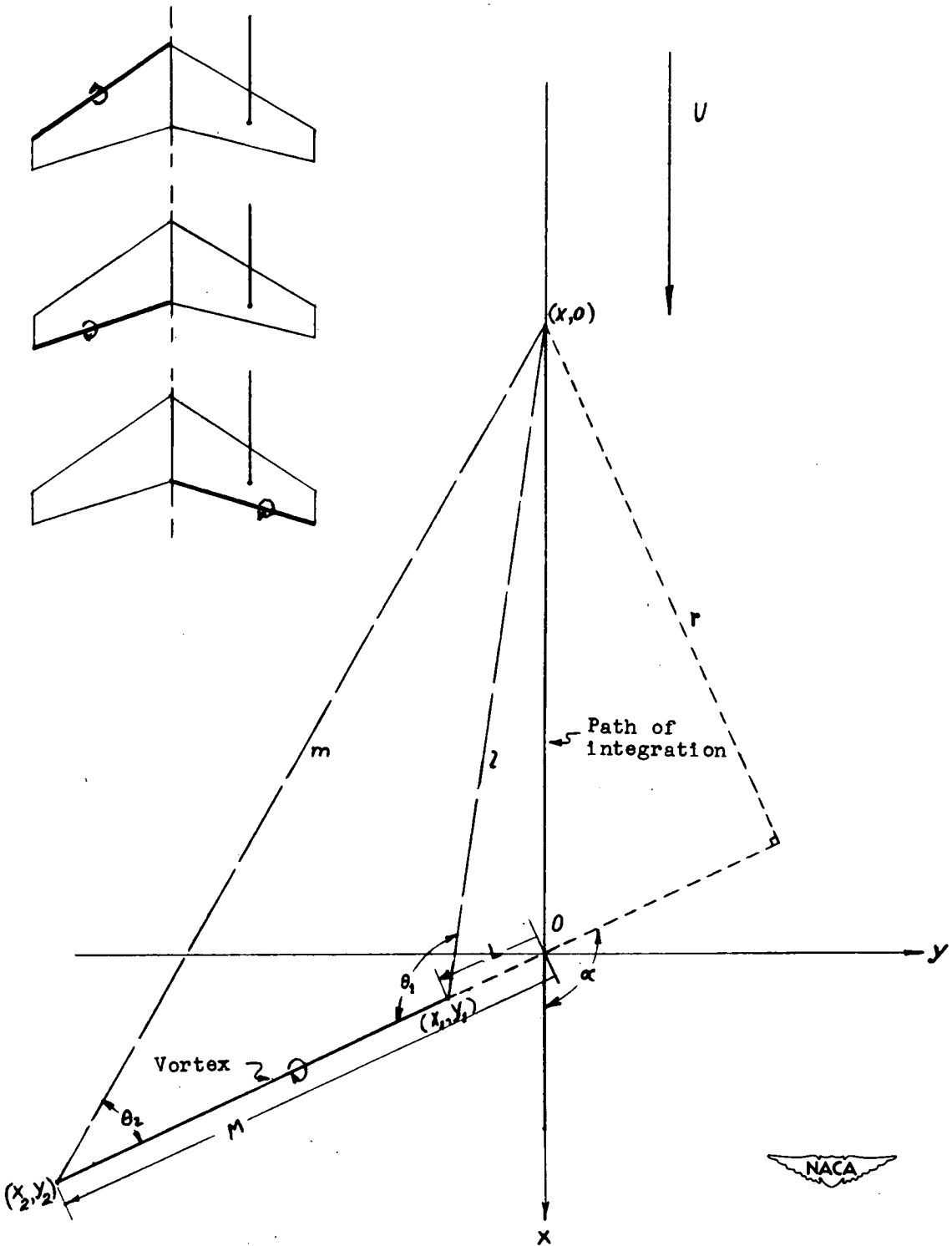
Figure 9.- Geometrical relationships for case II. Heavy lines in small sketches show relative positions of vortex and path of integration for three different conditions for which this case applies.
