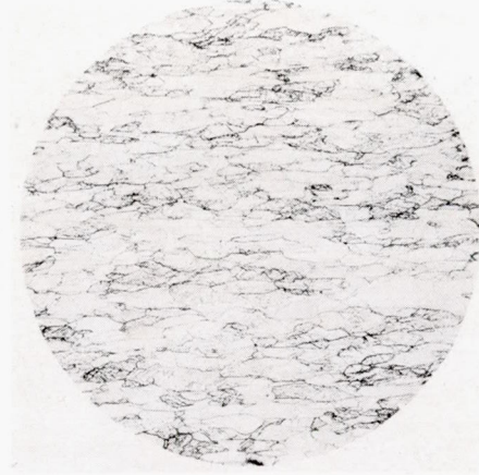
(c) Swaged 50 percent from 0.177-inch diameter recrystallized rod.
