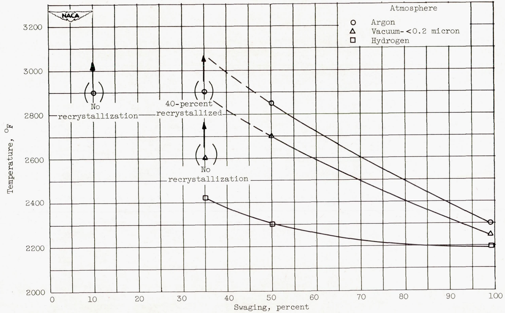
Figure 5. - Effect of atmosphere on total 1-hour recrystallization temperature of molybdenum (lot 3).
