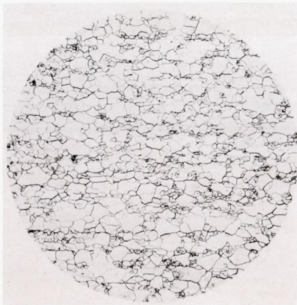
(a) Recrystallized.
