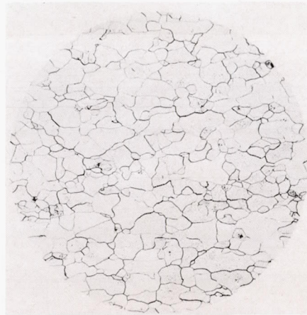
(b) Recrystallized.
