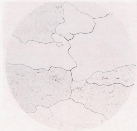
(e) Recrystallized.
