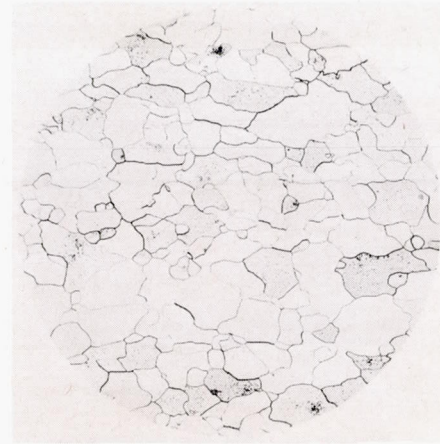
(c) Recrystallized.
