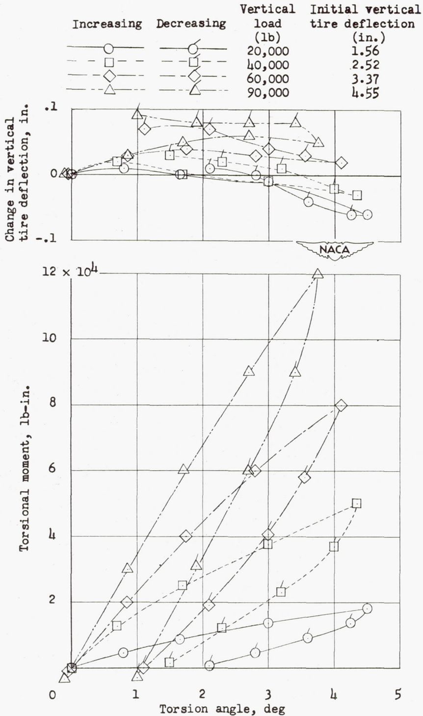
(a) Initial inflation pressure, 270 pounds per square inch.
