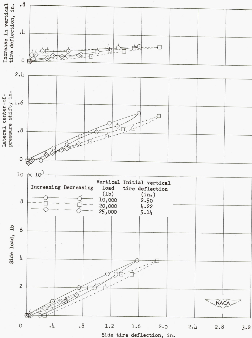
(c) Initial inflation pressure, 65 pound per square inch.
