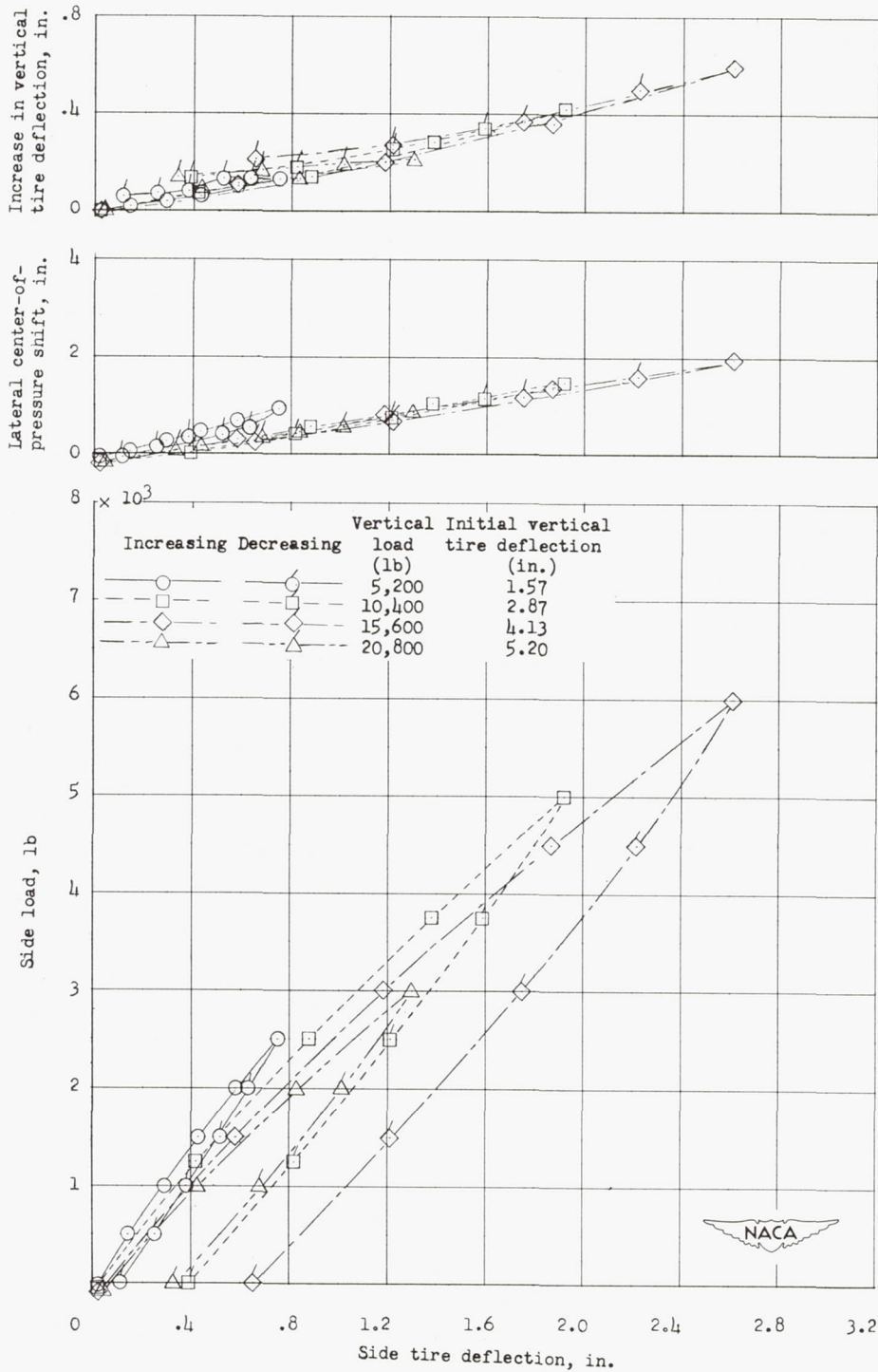
(b) Initial inflation pressure, 55 pounds per square inch.
