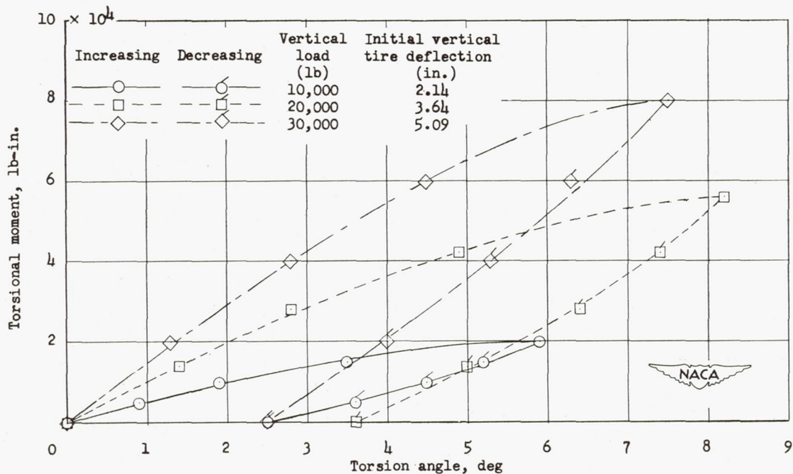
(b) Initial inflation pressure, 85 pounds per square inch.
