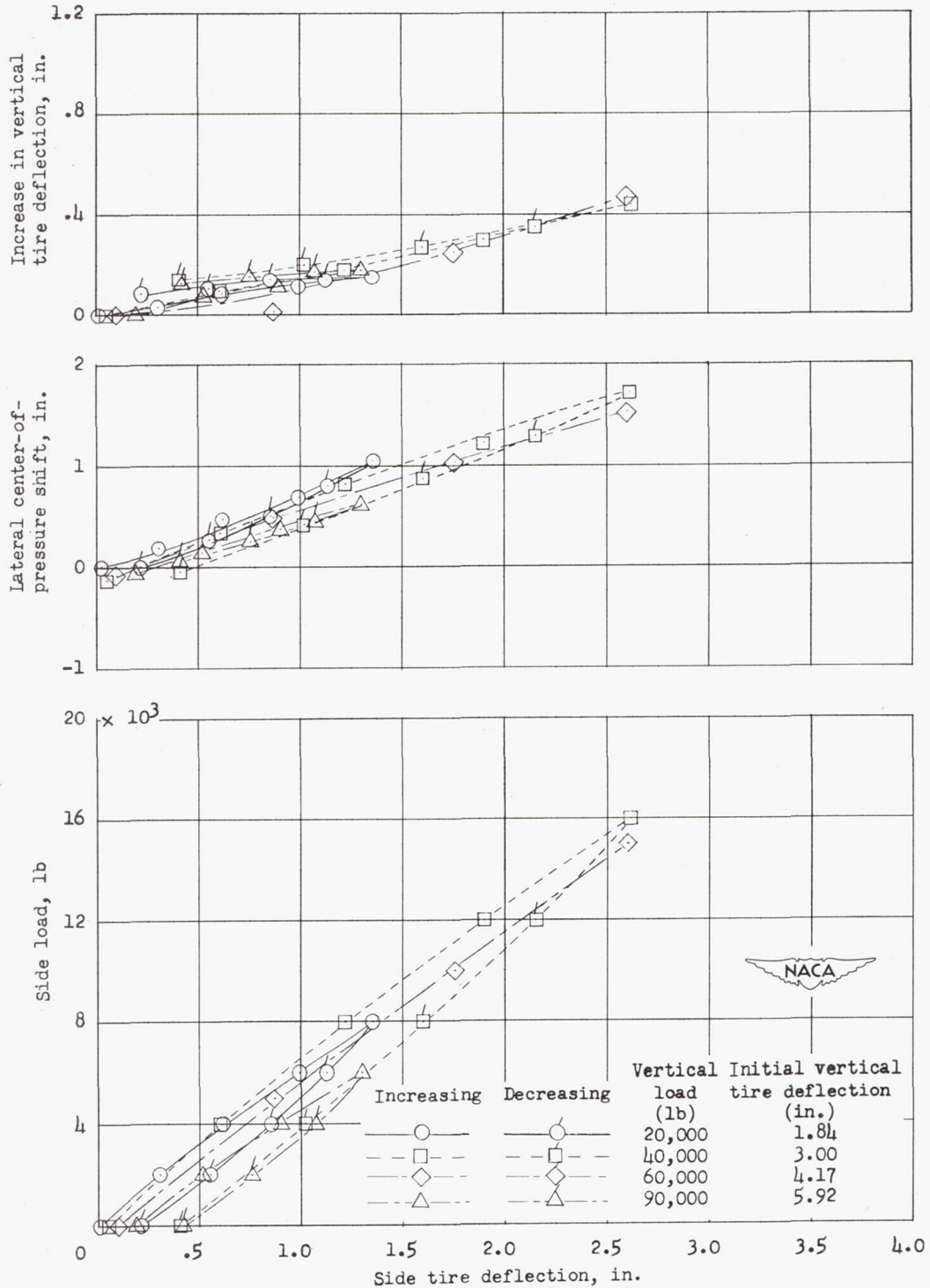
(a) Initial inflation pressure, 200 pounds per square inch.
