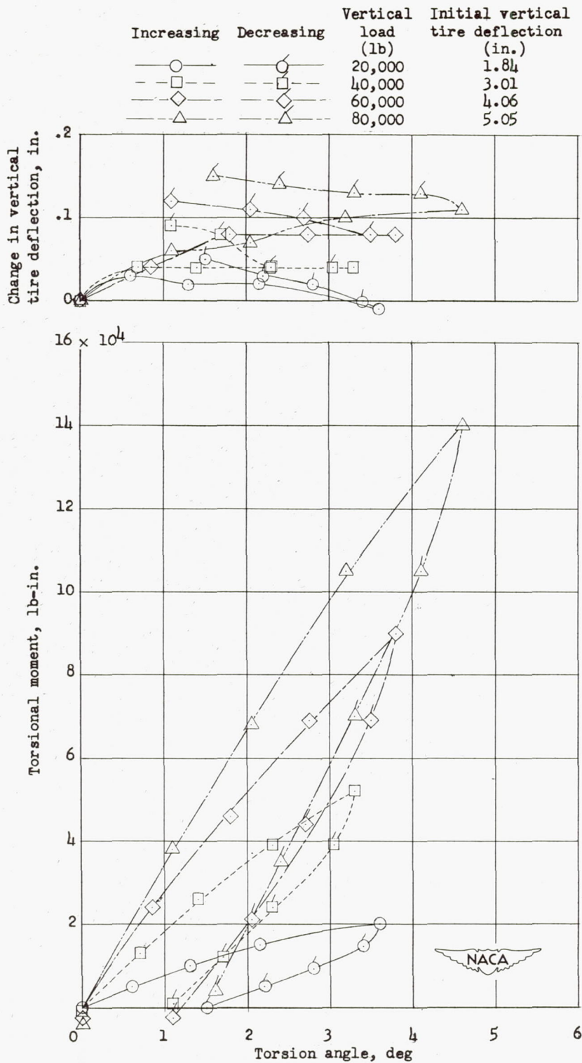
(c) Initial inflation pressure, 200 pounds per square inch.
