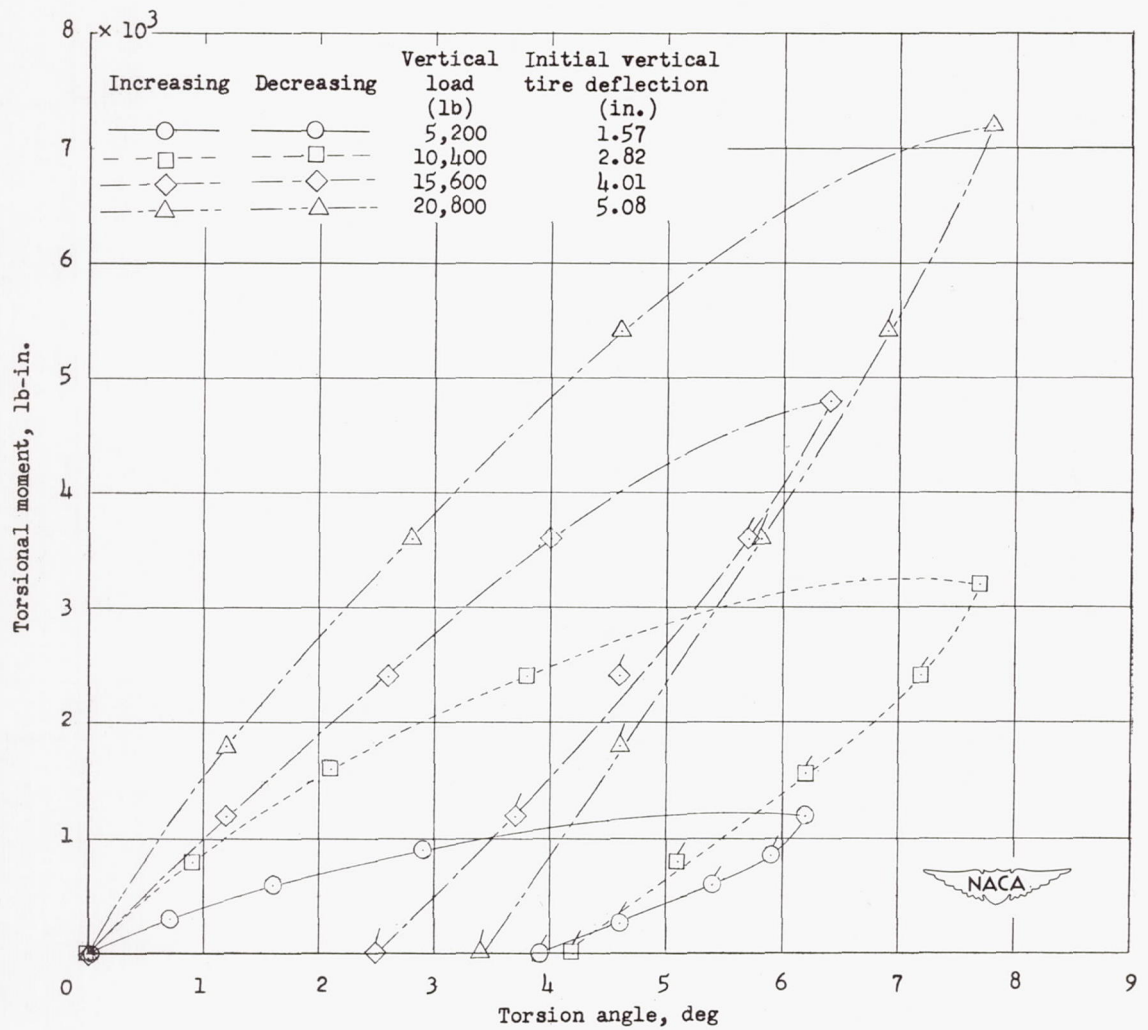
(b) Initial inflation pressure, 55 pounds per square inch.
