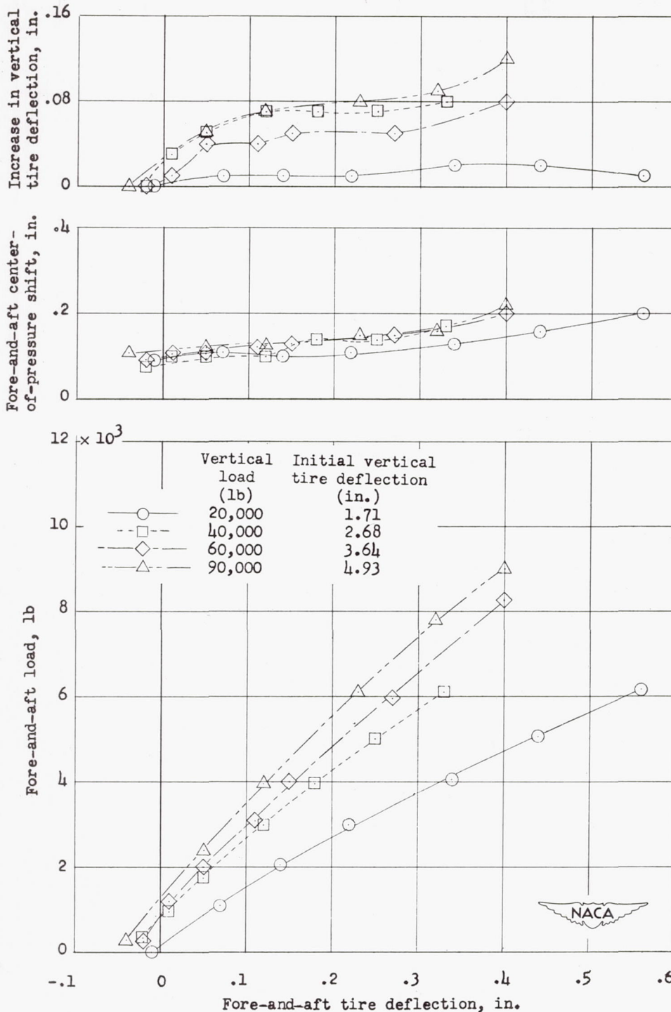
(b) Initial inflation pressure, 240 pounds per square inch.
