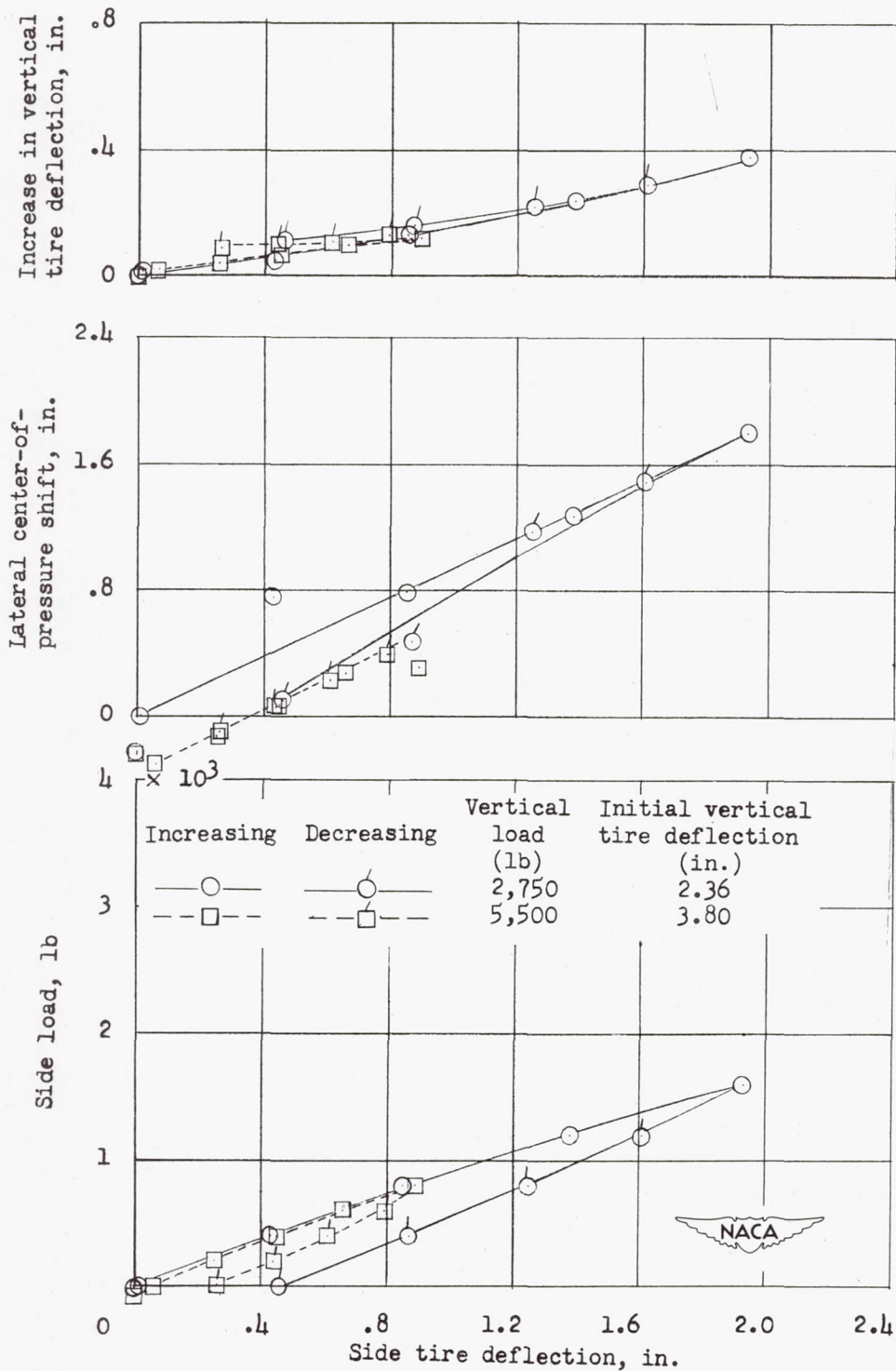
(d) Initial inflation pressure, 24 pounds per square inch.
