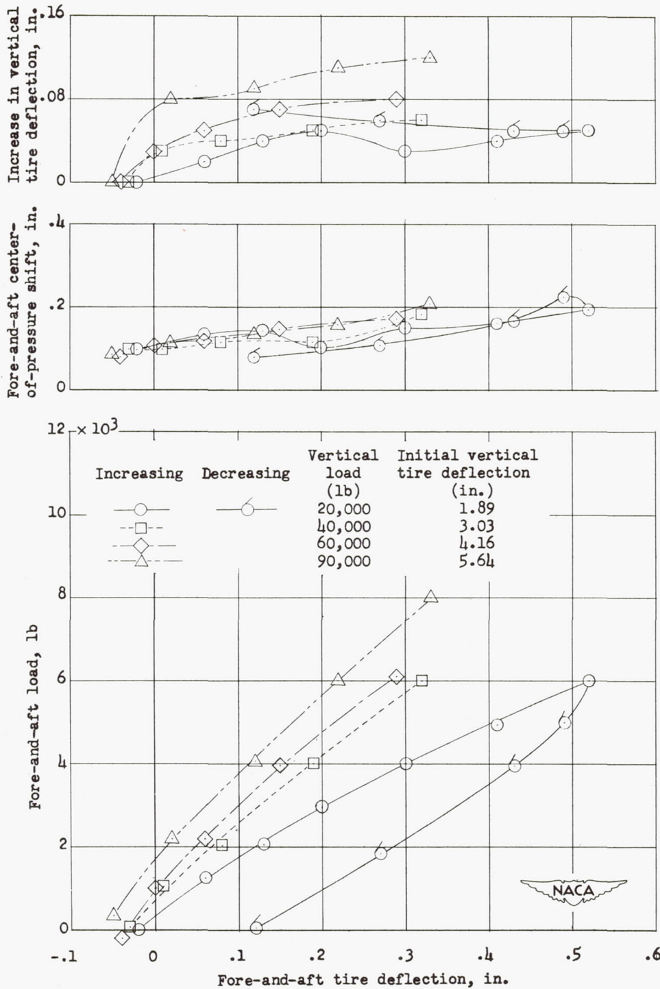
(c) Initial inflation pressure, 200 pounds per square inch.
