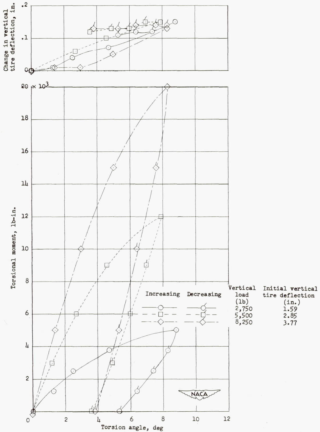
(b) Initial inflation pressure, 40 pounds per square inch.
