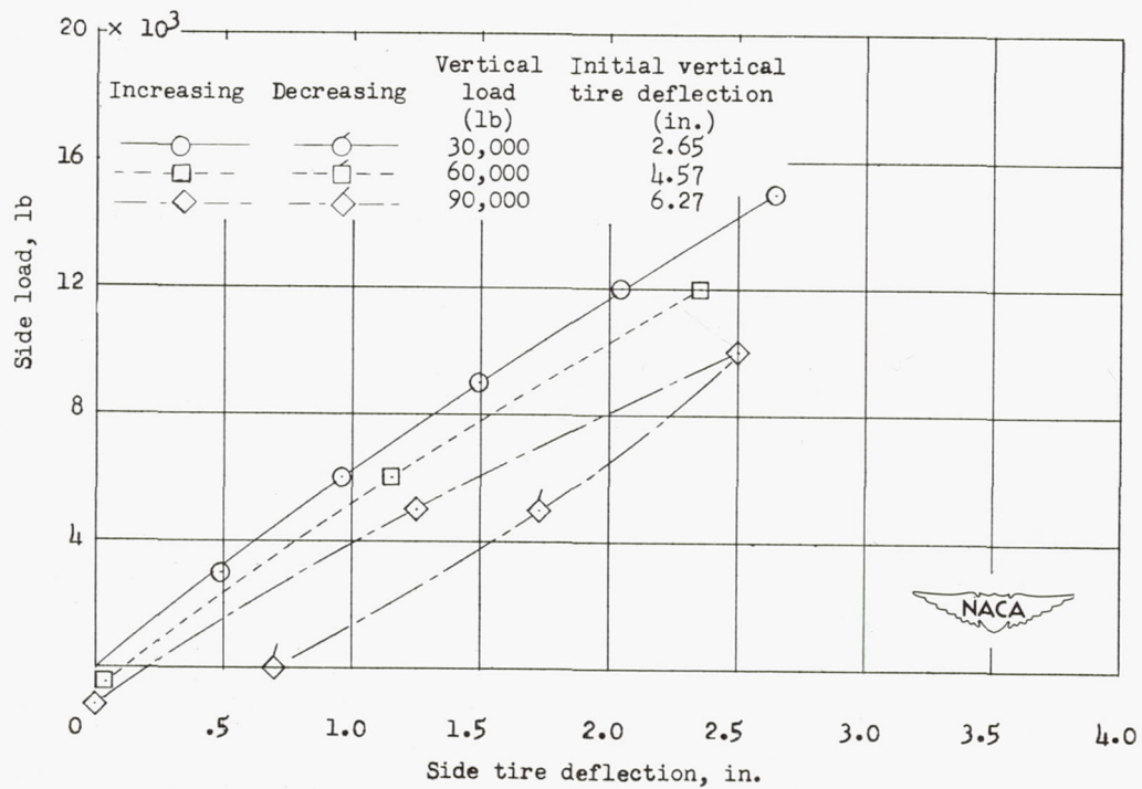
(b) Initial inflation pressure, 180 pounds per square inch.
