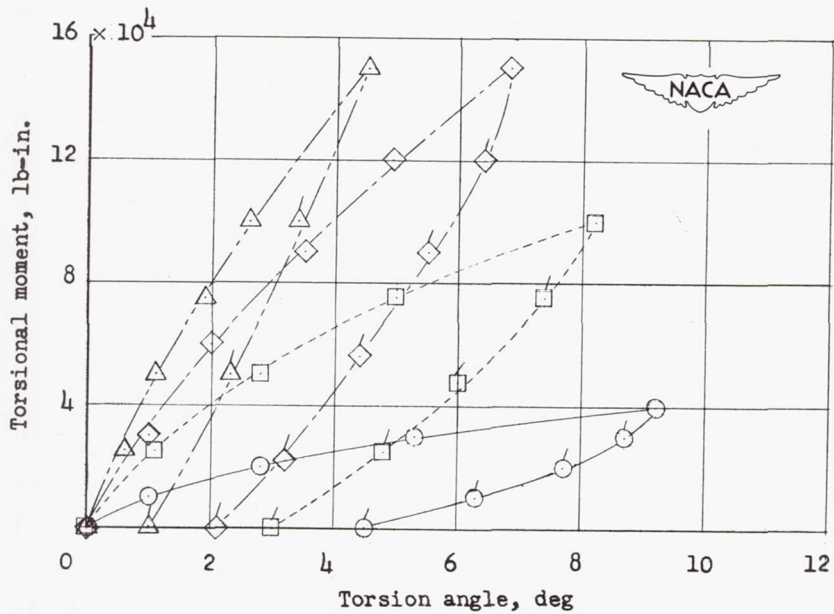
(b) Initial inflation pressure, 180 pounds per square inch.
