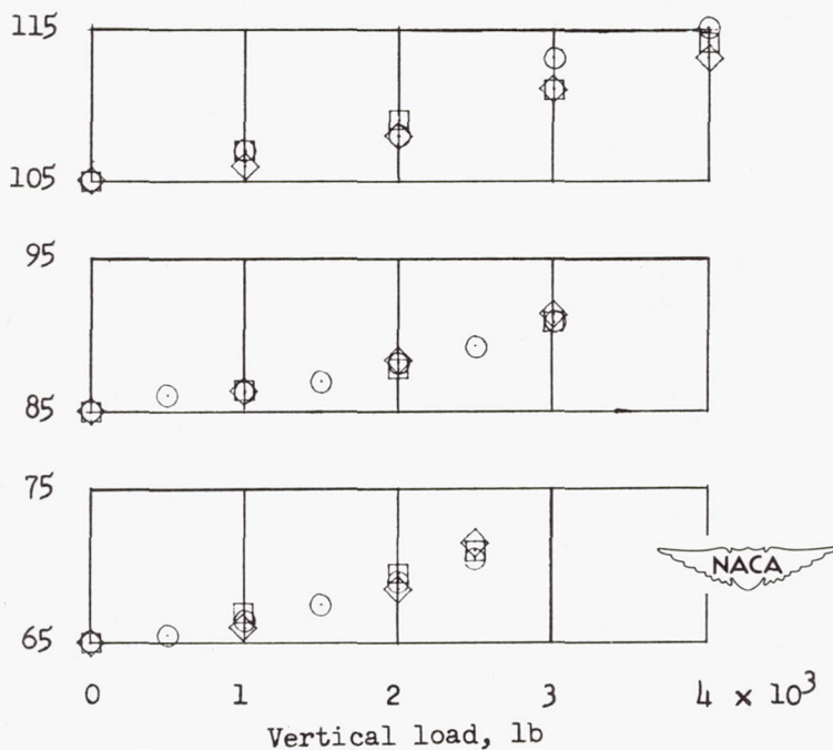
(b) Tire pressure against vertical load.
