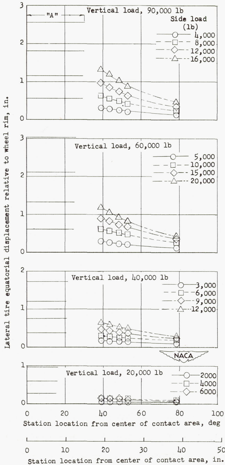
(b) Initial inflation pressure, 240 pounds per square inch.
