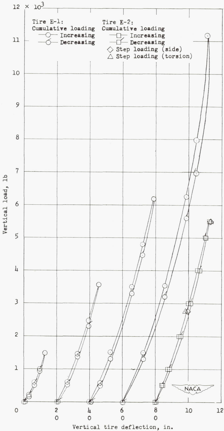
(d) Initial inflation pressure, 32 pounds per square inch; tires E-1 and E-2.
