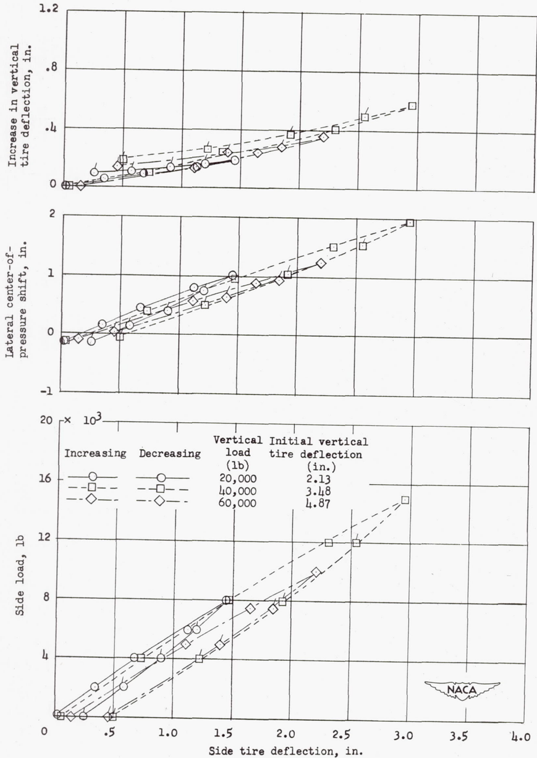
(c) Initial inflation pressure, 160 pounds per square inch.
