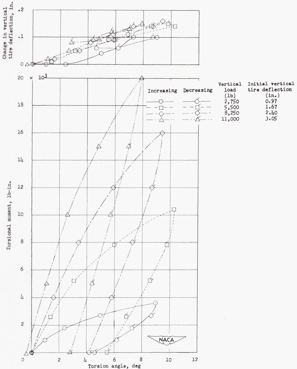
(a) Initial inflation pressure, 80 pounds per square inch.
