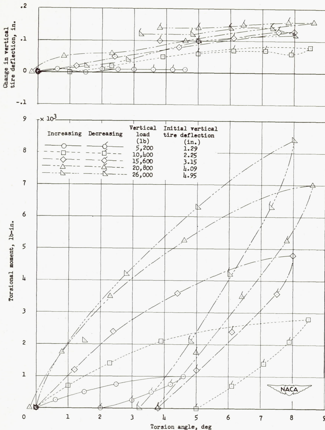
(a) Initial inflation pressure, 75 pounds per square inch.
