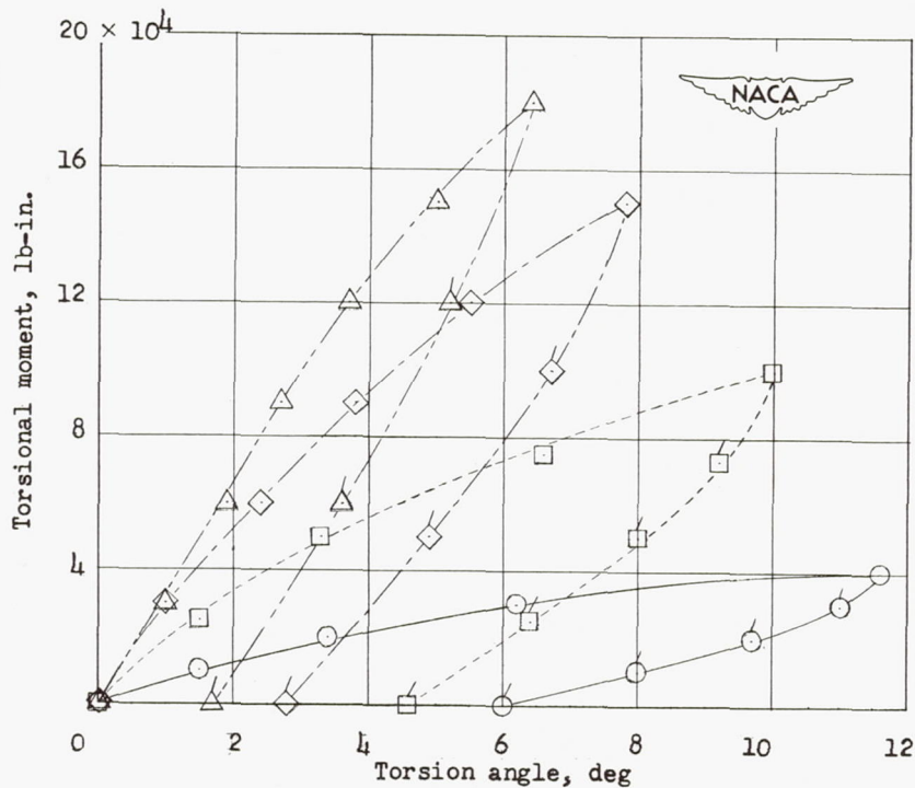
(a) Initial inflation pressure, 200 pounds per square inch.
