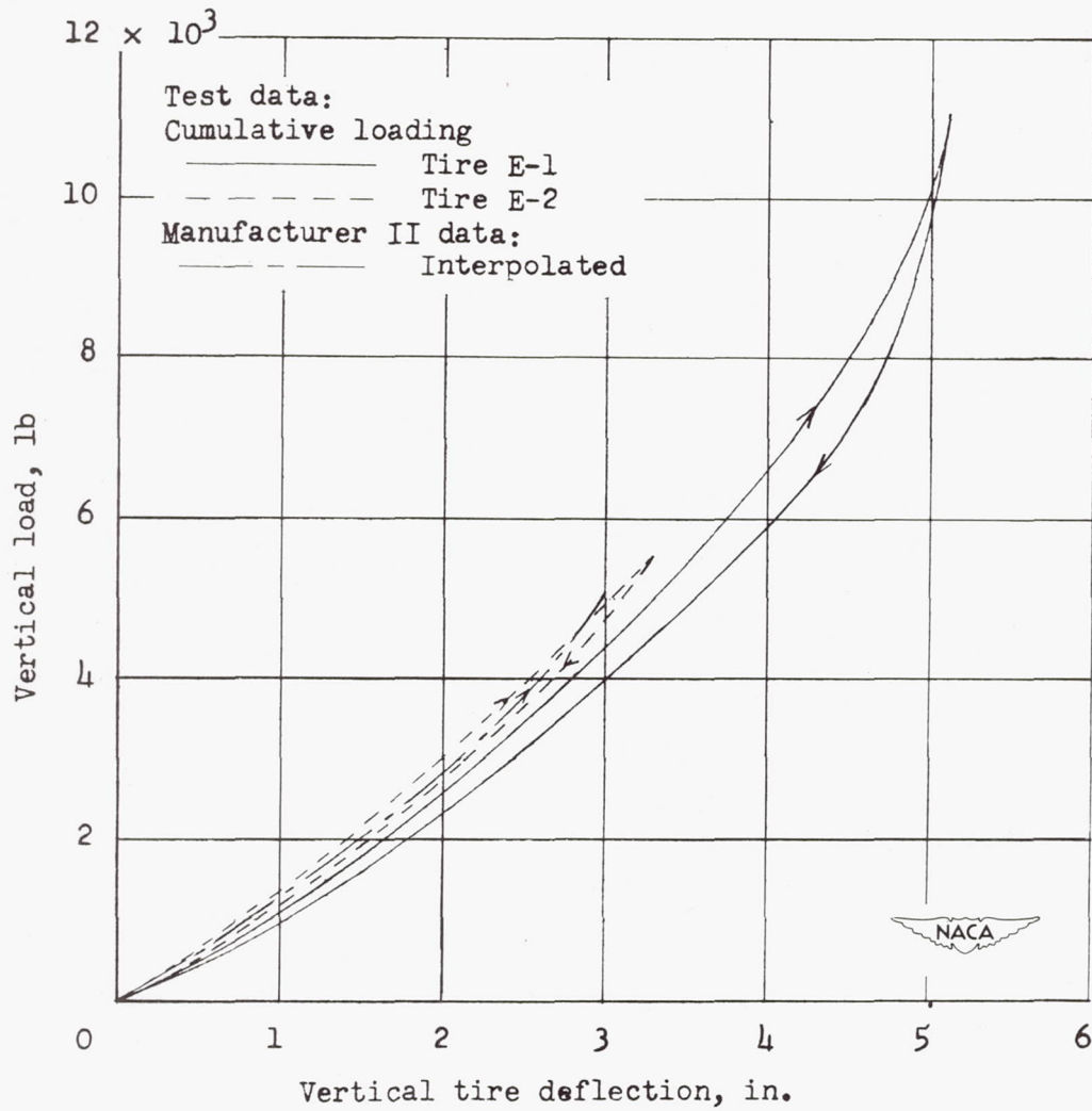
(b) Initial inflation pressure, 32 pounds per square inch.
