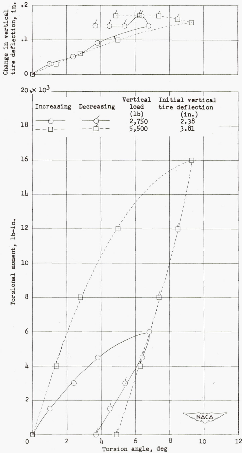
(d) Initial inflation pressure, 24 pounds per square inch.
