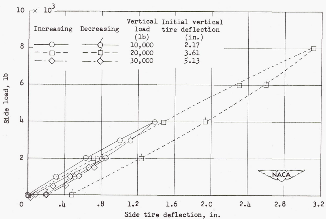
(b) Initial inflation pressure, 85 pounds per square inch.
