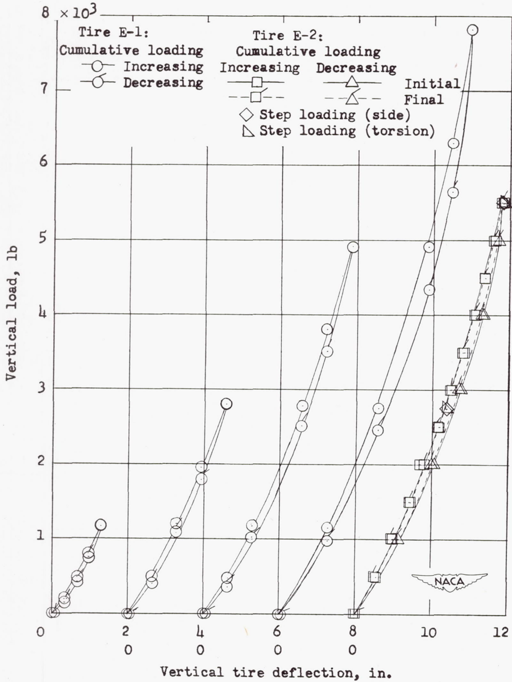
(e) Initial inflation pressure, 24 pounds per square inch; tires E-1 and E-2.
