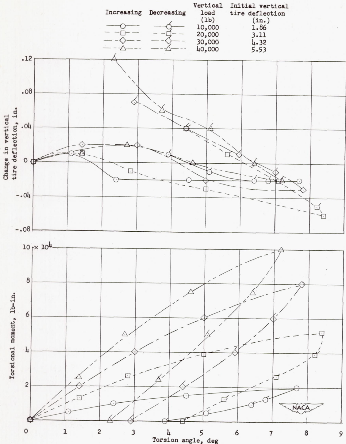
(a) Initial inflation pressure, 105 pounds per square inch.
