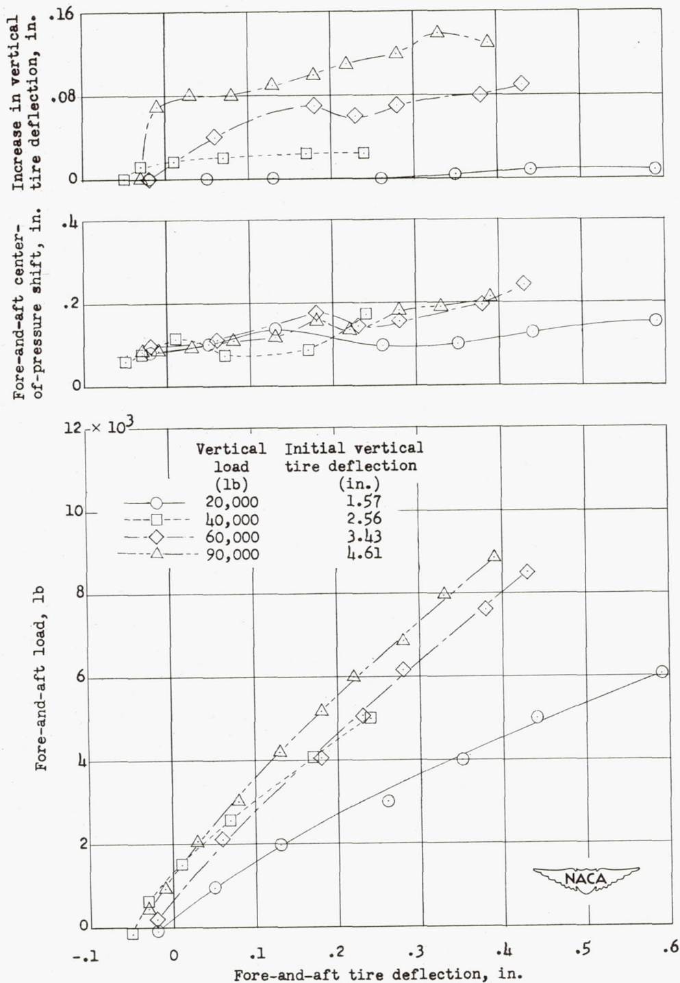
(a) Initial inflation pressure, 270 pounds per square inch.
