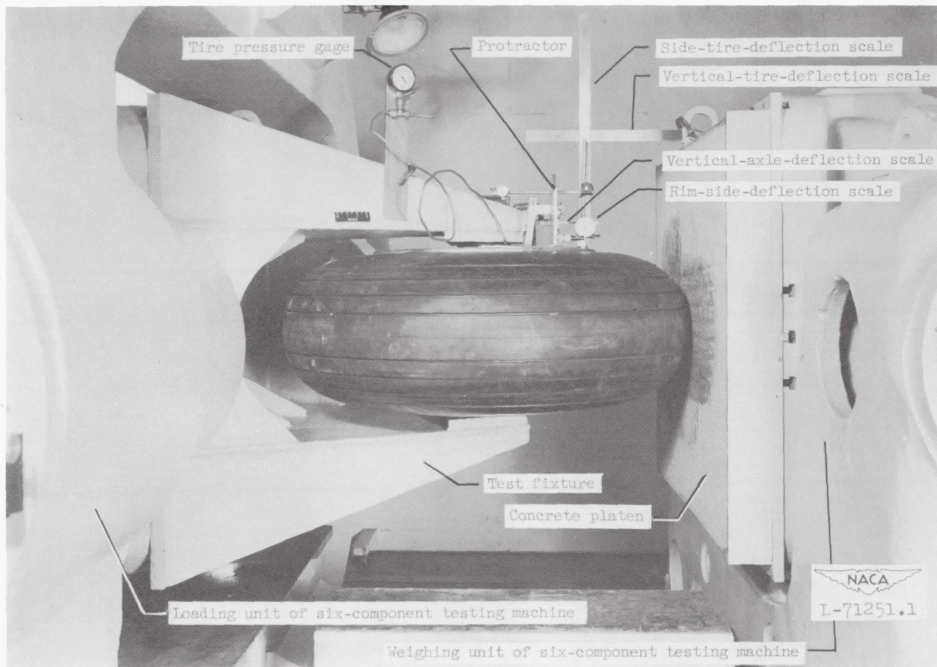
(a) Undeformed position. Inflation pressure, 35 pounds per square inch.
