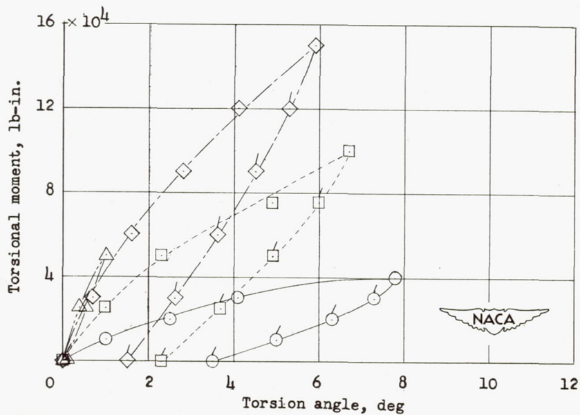
(c) Initial inflation pressure, 160 pounds per square inch.
