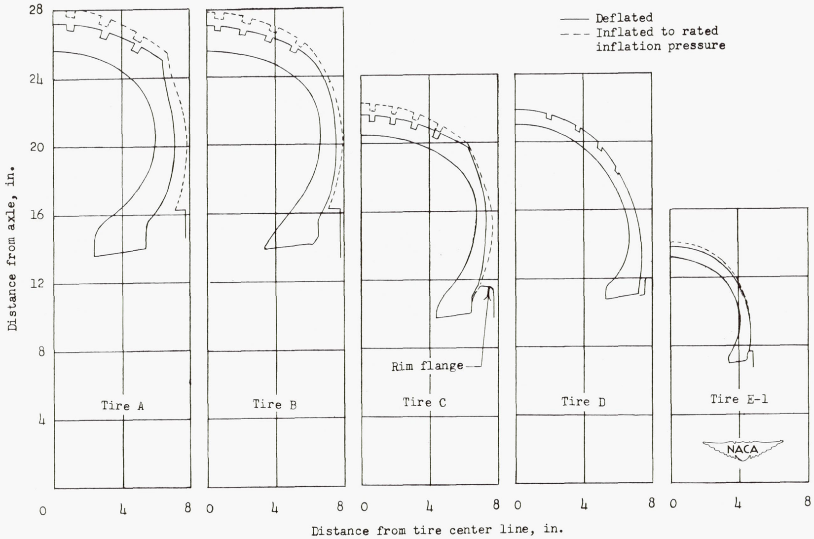
Figure 2.- Tire profiles.
