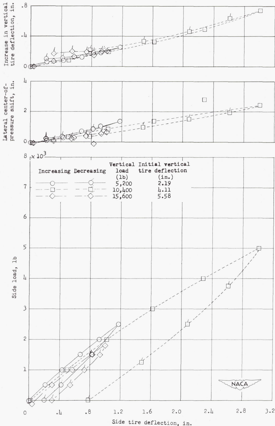
(c) Initial inflation pressure, 35 pounds per square inch.
