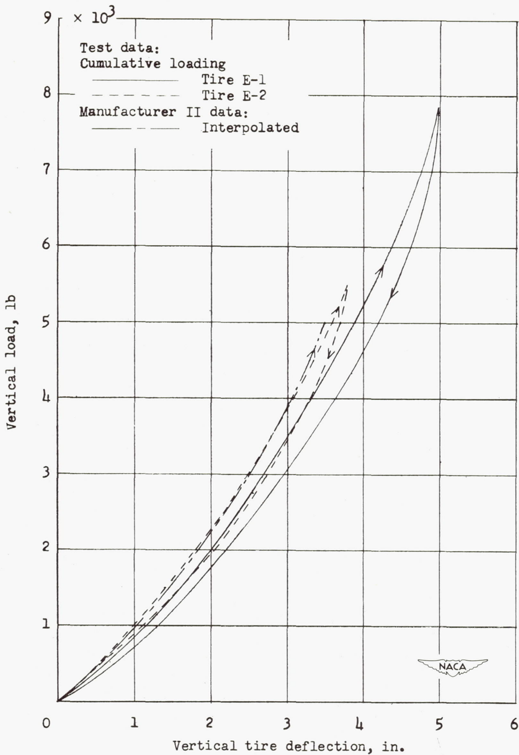
(c) Initial inflation pressure, 24 pounds per square inch.
