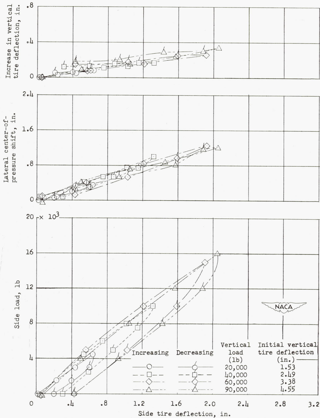
(a) Initial inflation pressure, 270 pounds per square inch.
