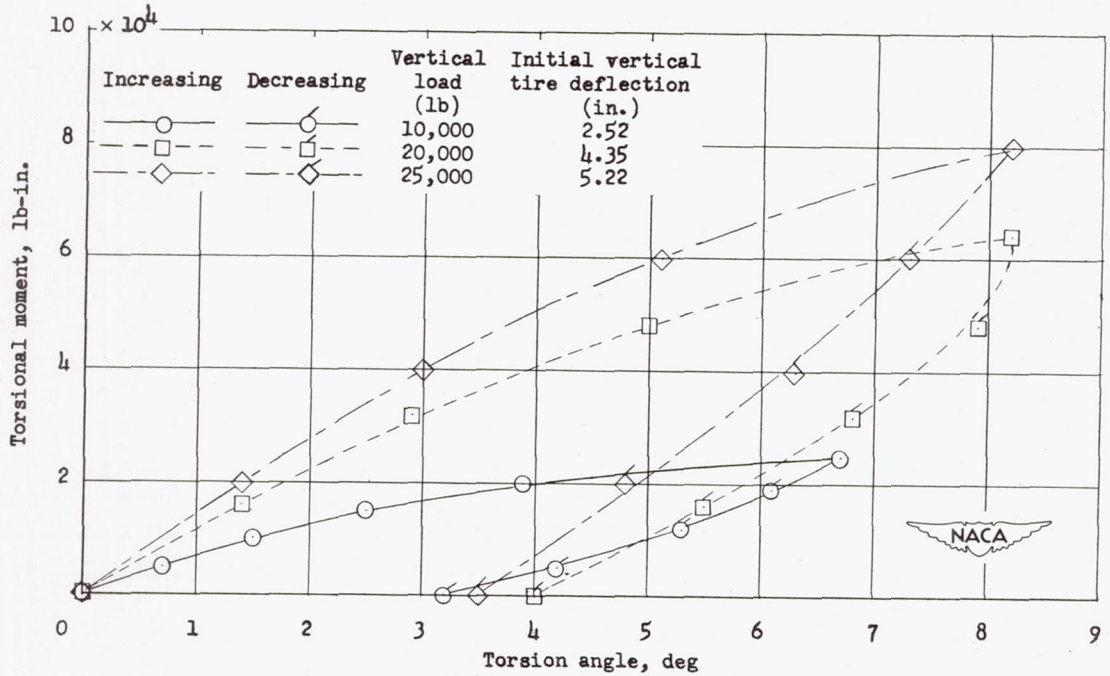
(c) Initial inflation pressure, 65 pounds per square inch.
