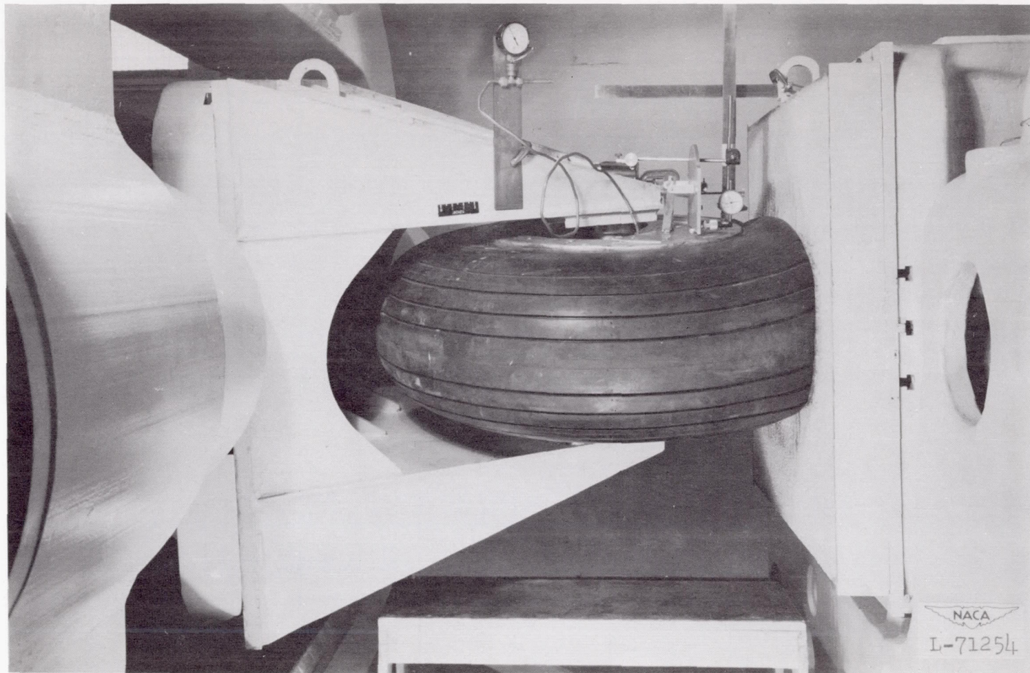
(d) Under 15,000 pounds vertical load and 64,000 pound-inches torsional moment.
