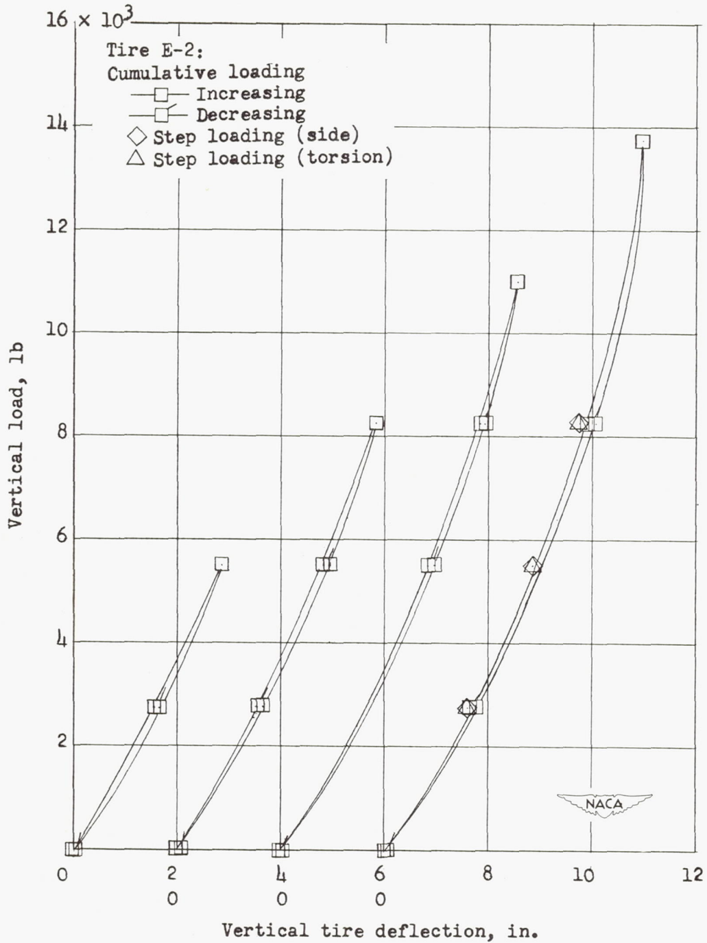
(b) Initial inflation pressure, 40 pounds per square inch; tire E-2.
