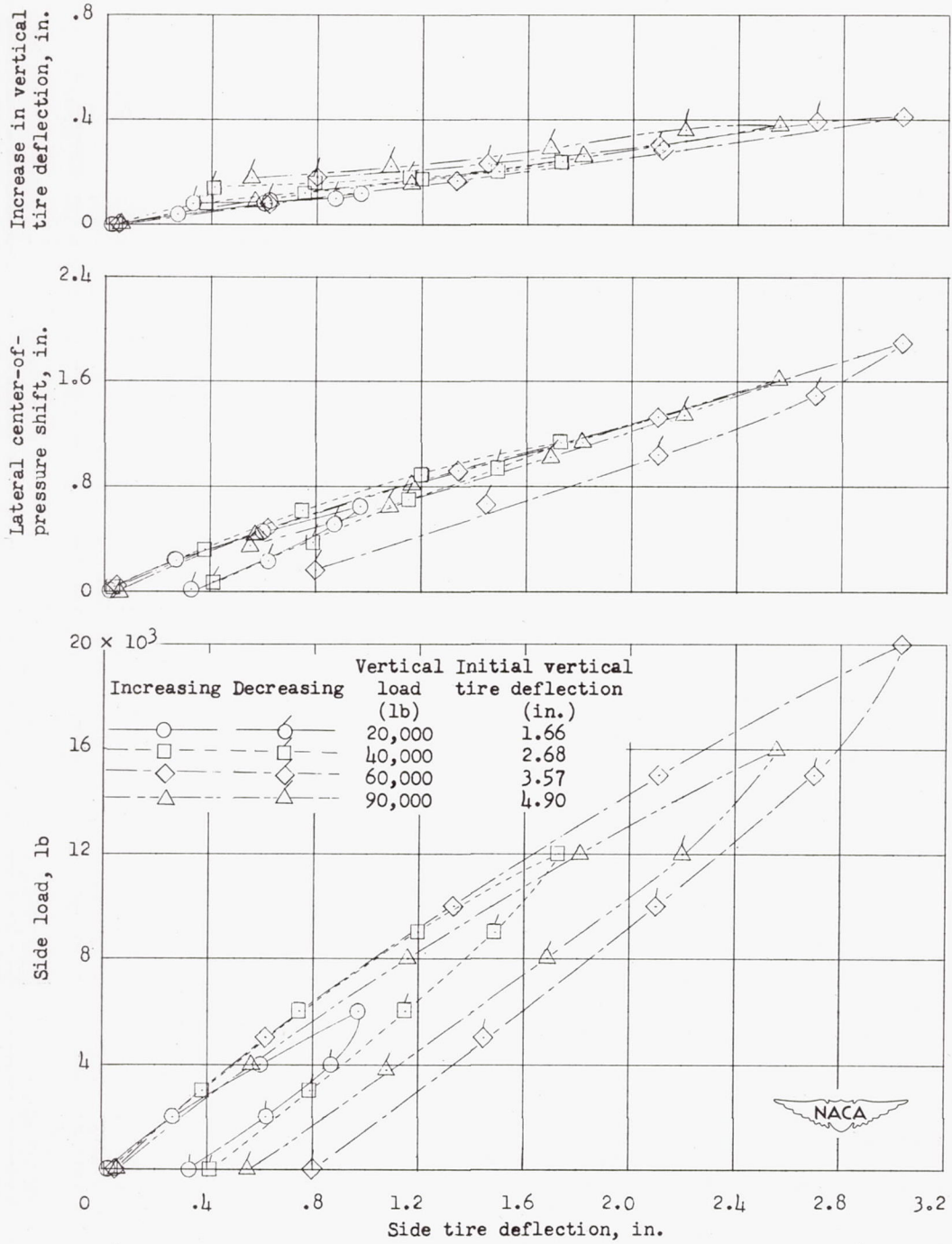
(b) Initial inflation pressure, 240 pounds per square inch.
