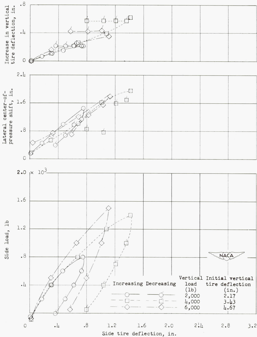
(e) Initial inflation pressure, 0 pounds per square inch.
