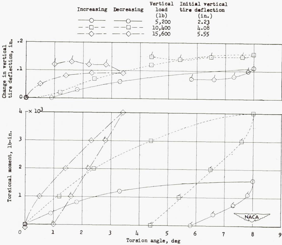
(c) Initial inflation pressure, 35 pounds per square inch.
