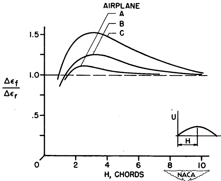
Figure 4.- Strain amplification for single-gust encounter.
