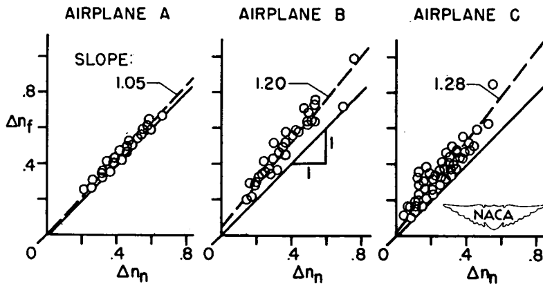
Figure 3.- Acceleration measured in clear rough air.
