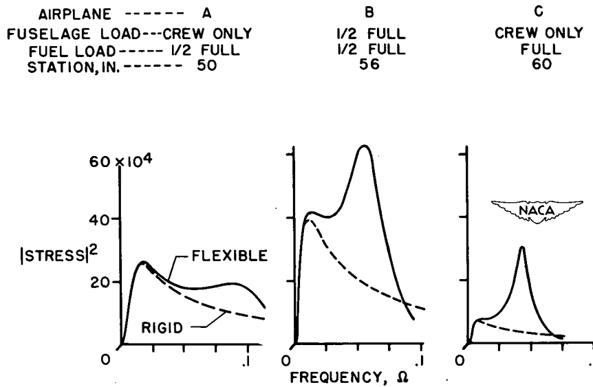
Figure 7.- Transfer functions.
