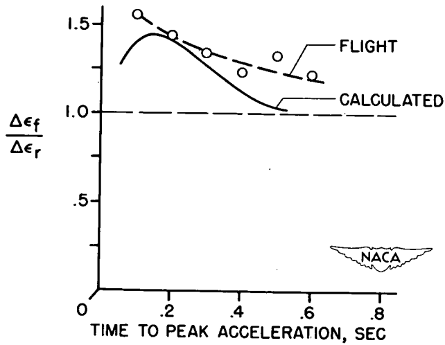
Figure 5.- Rough-air strain amplification for airplane C.
