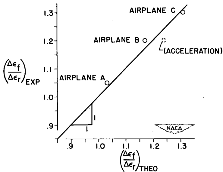
Figure 8.- Strain amplification for continuous turbulence.
