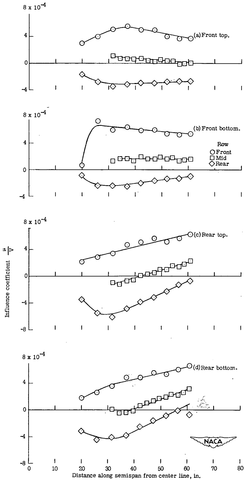
Figure 16.- Influence coefficients for structure B - uncombined left torque bridges.
