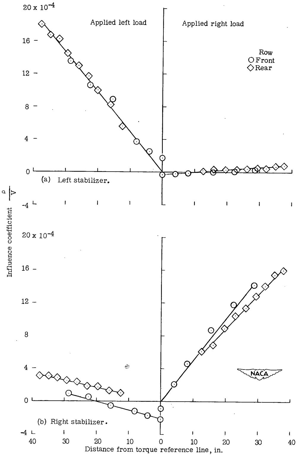
Figure 20.- Influence coefficients for structure B - combined torque bridges.
