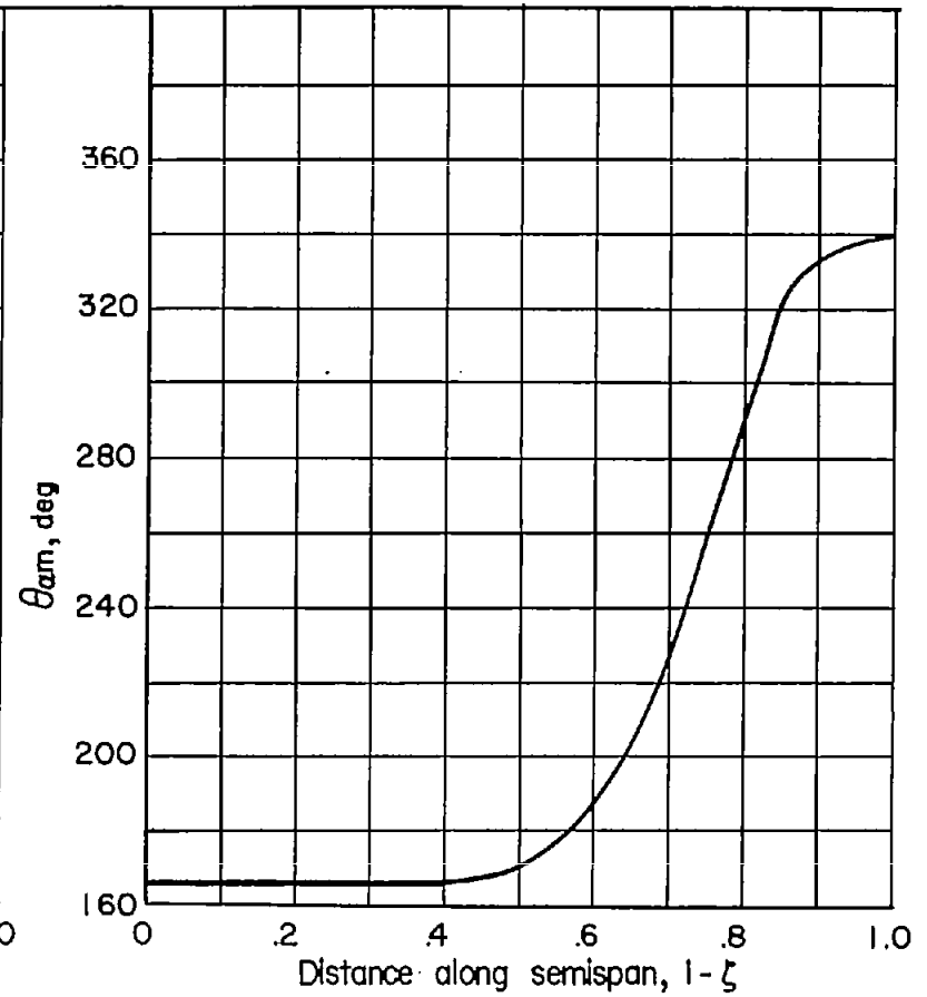
(d) Phase angle between moment vector due to pitching and angular-displacement vector a .
