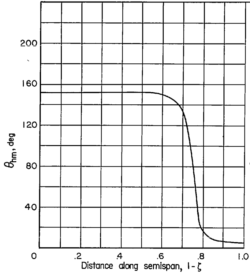
(c) Phase angle between moment vector due to vertical translation and vertical-velocity vector h .
