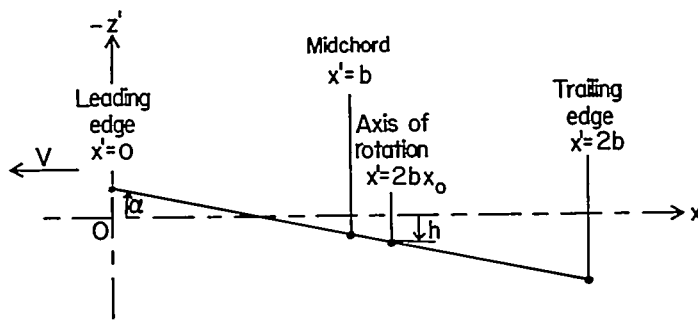
(b) Section y' = y'_m ( x'z' -plane).
