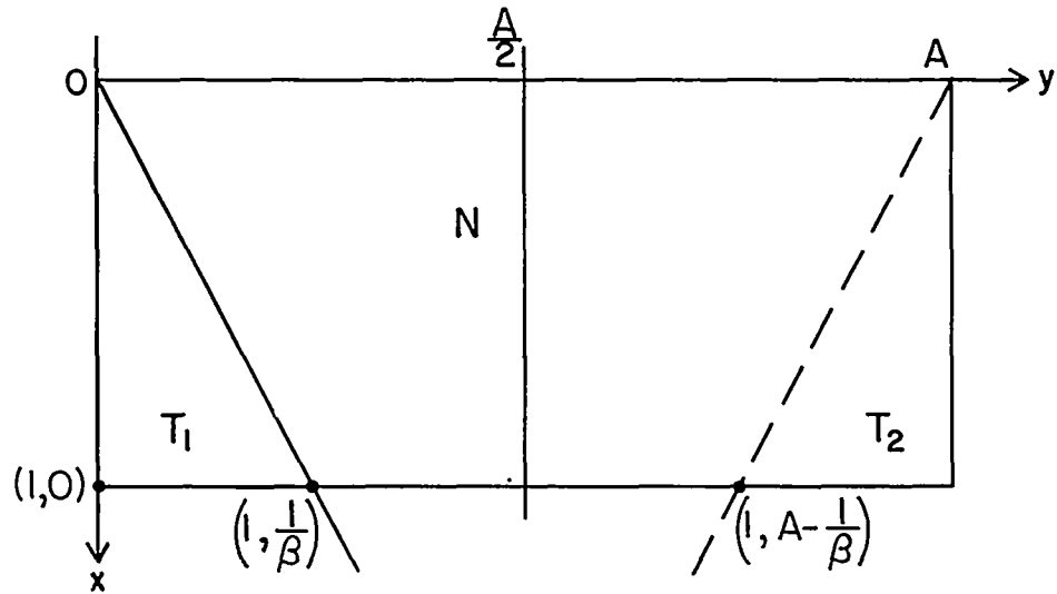
(a) Case 1.- Mach lines from tips do not intersect on wing ( A\beta > 2 ).
