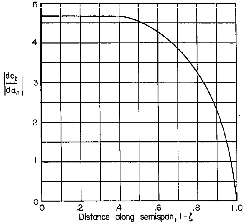
(a) Lift-curve slope associated with vertical translation of wing \left| \frac{dc_1}{da_h} \right| = 4k \sqrt{L_1^2 + L_2^2} .
