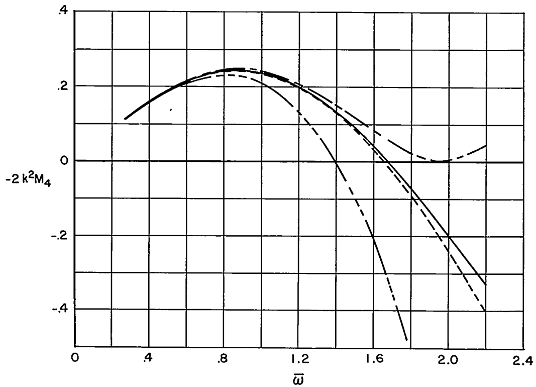
(d) Imaginary part of moment-curve slope associated with pitching of wing.
