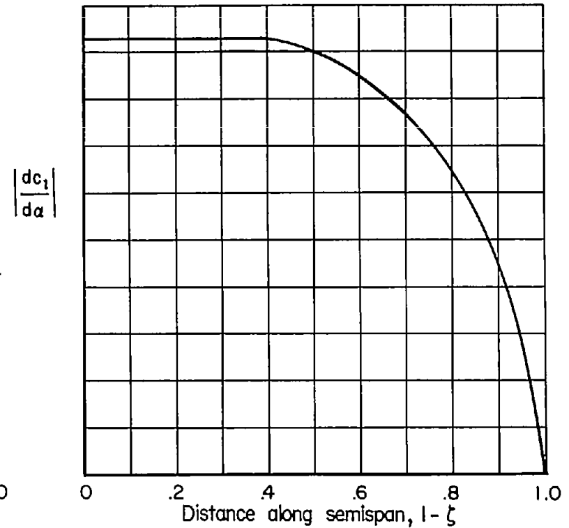
(b) Lift-curve slope associated with pitching of wing \left| \frac{dc_1}{da} \right| = 4k^2 \sqrt{L_3^2 + L_4^2} .
