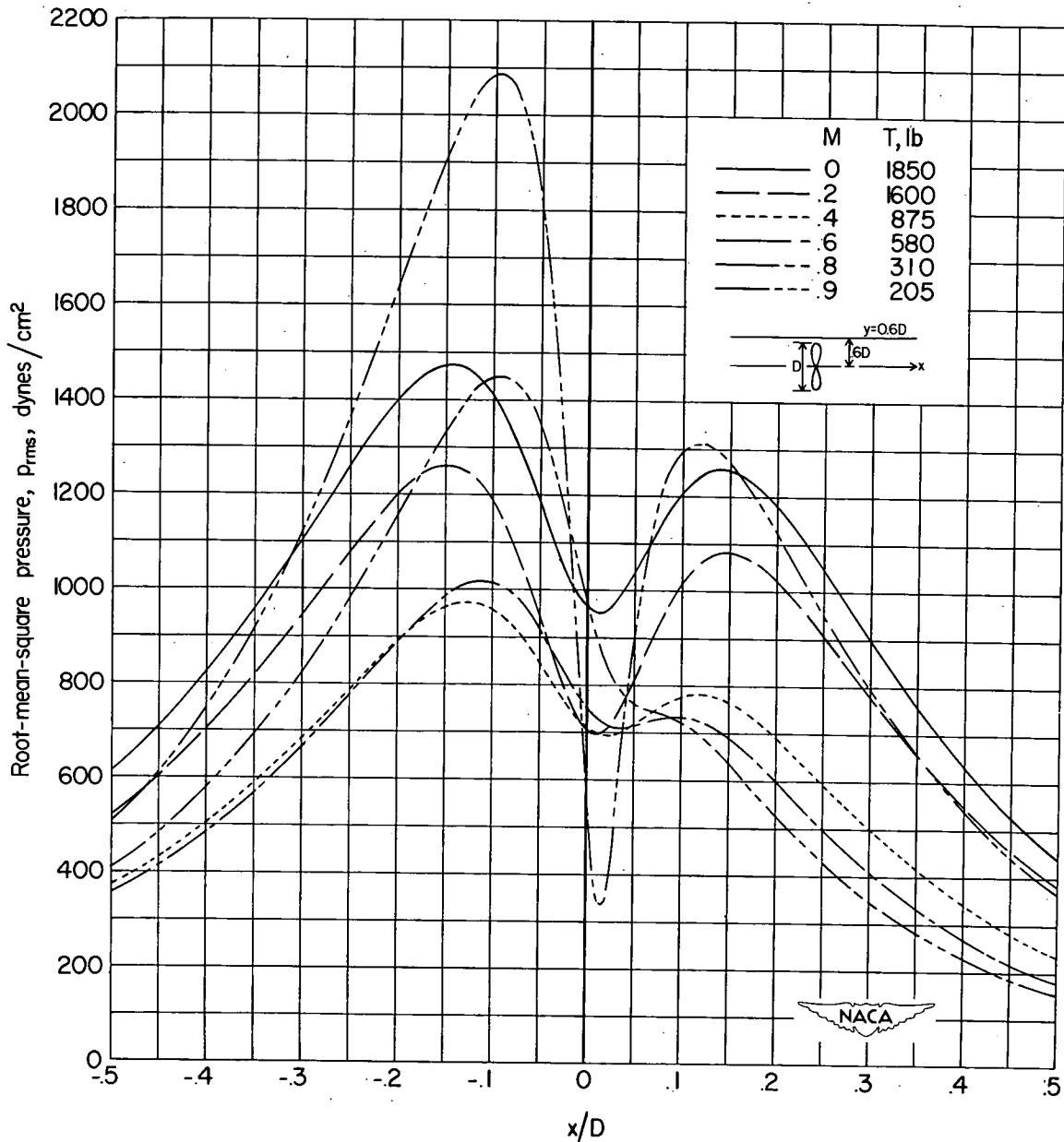
Figure 4.- Distribution of the root-mean-square pressures for the fundamental ( m = 1 ) of a two-blade 10-foot-diameter propeller at several forward-speed Mach numbers. C_p = 0.10 ; k = 0.29686 ; y = 6 feet. (Operating conditions of propeller given in table I.)
