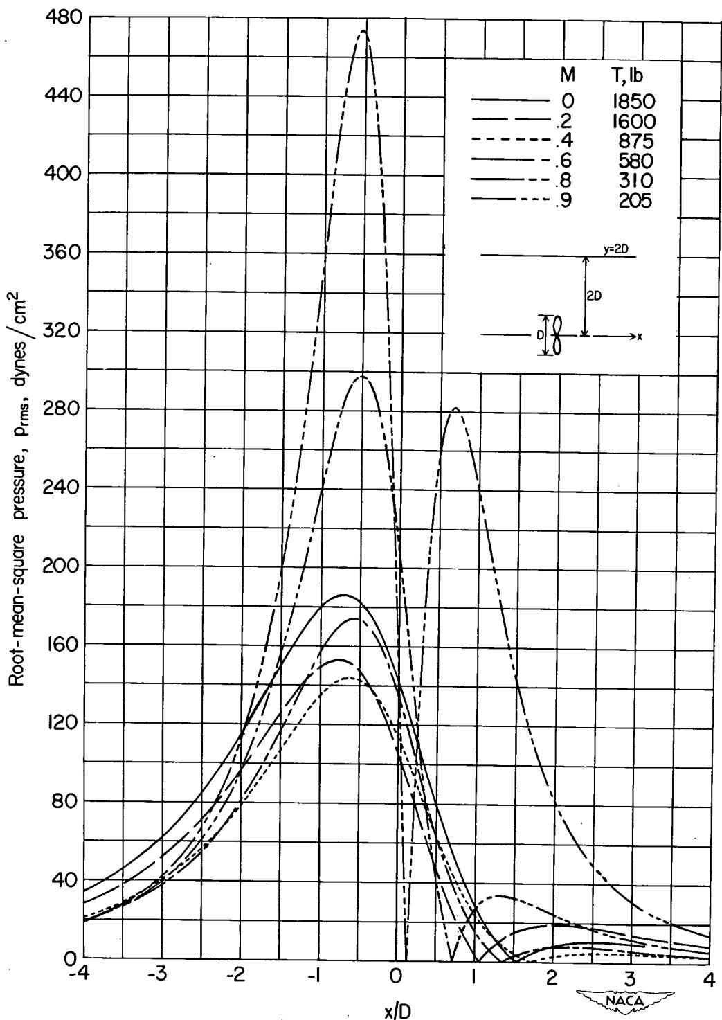
Figure 5.- Distribution of the root-mean-square pressures for the fundamental ( m = 1 ) of a two-blade 10-foot-diameter propeller at several forward-speed Mach numbers. C_p = 0.10 ; k = 0.29686 ; y = 20 feet. (Operating conditions of propeller given in table I.)
