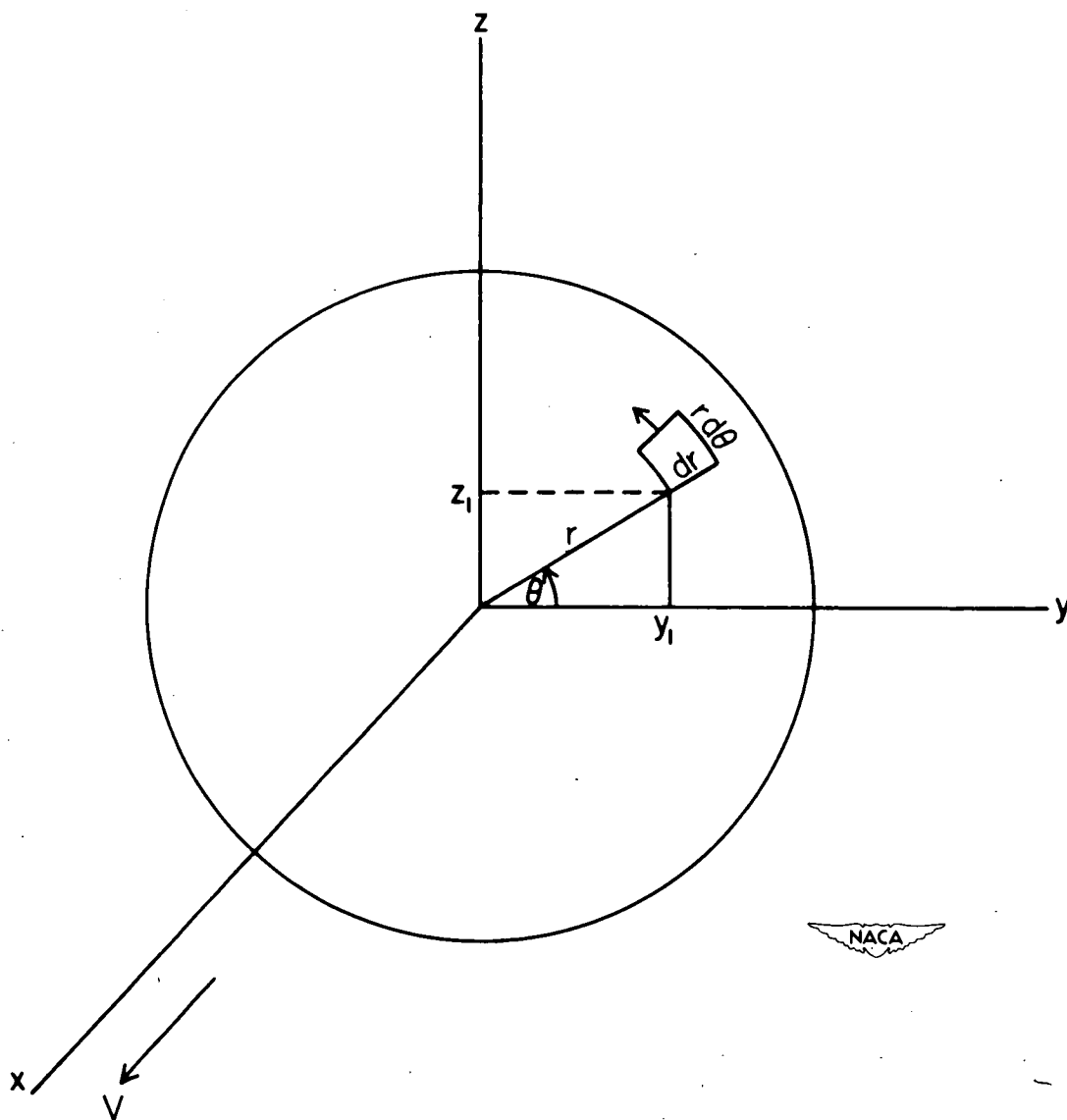
Figure 2.- Propeller disk and coordinate system.
