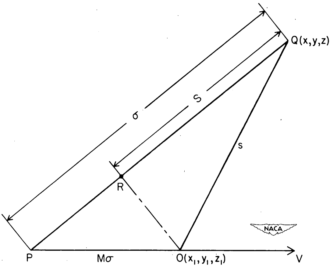
Figure 1.- Geometric representation of s , S , and \sigma .
