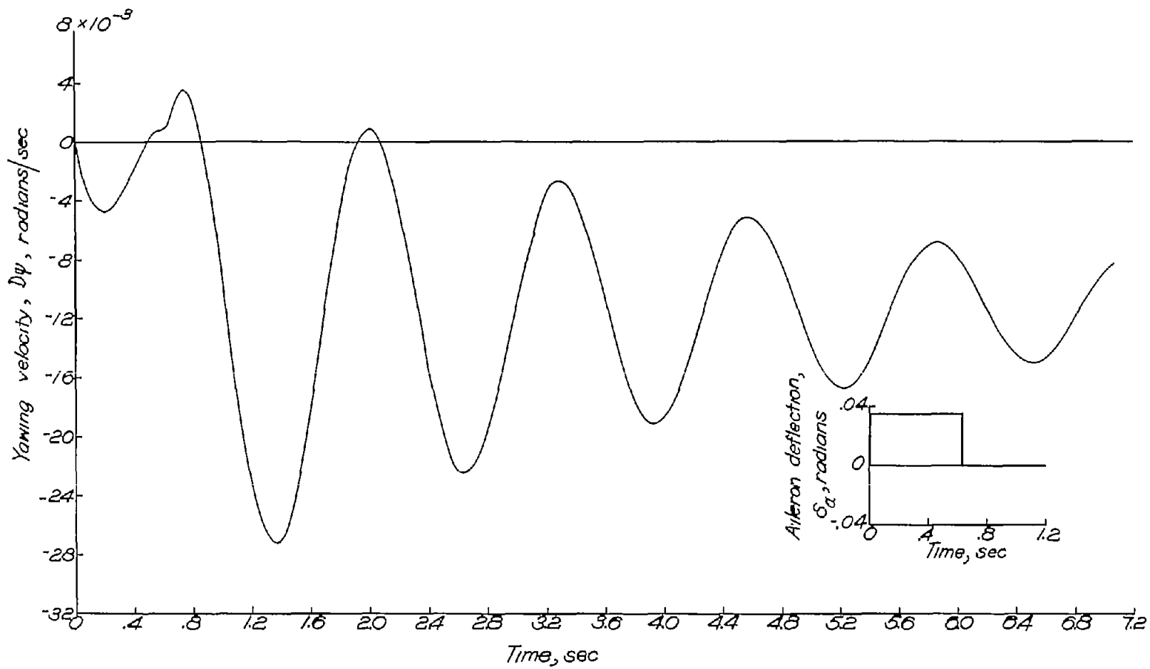
(b) Yawing velocity.
