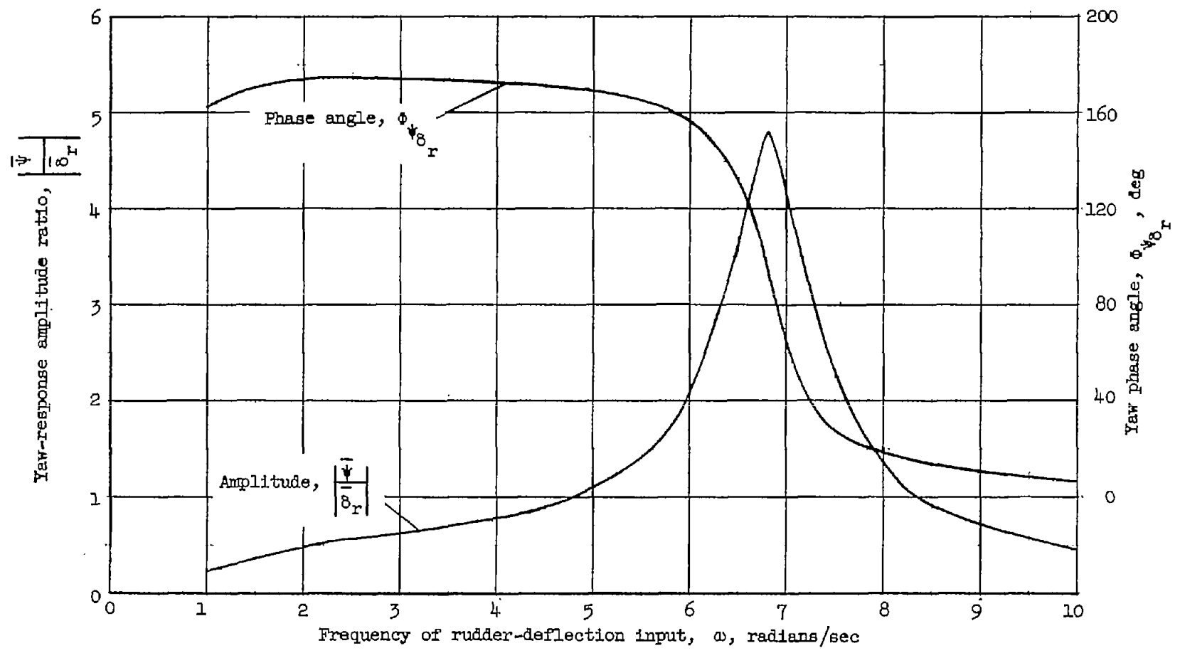
Figure 5.- Frequency response, in yaw due to rudder-deflection input for rigid, high-speed airplane of example given in body of paper.
