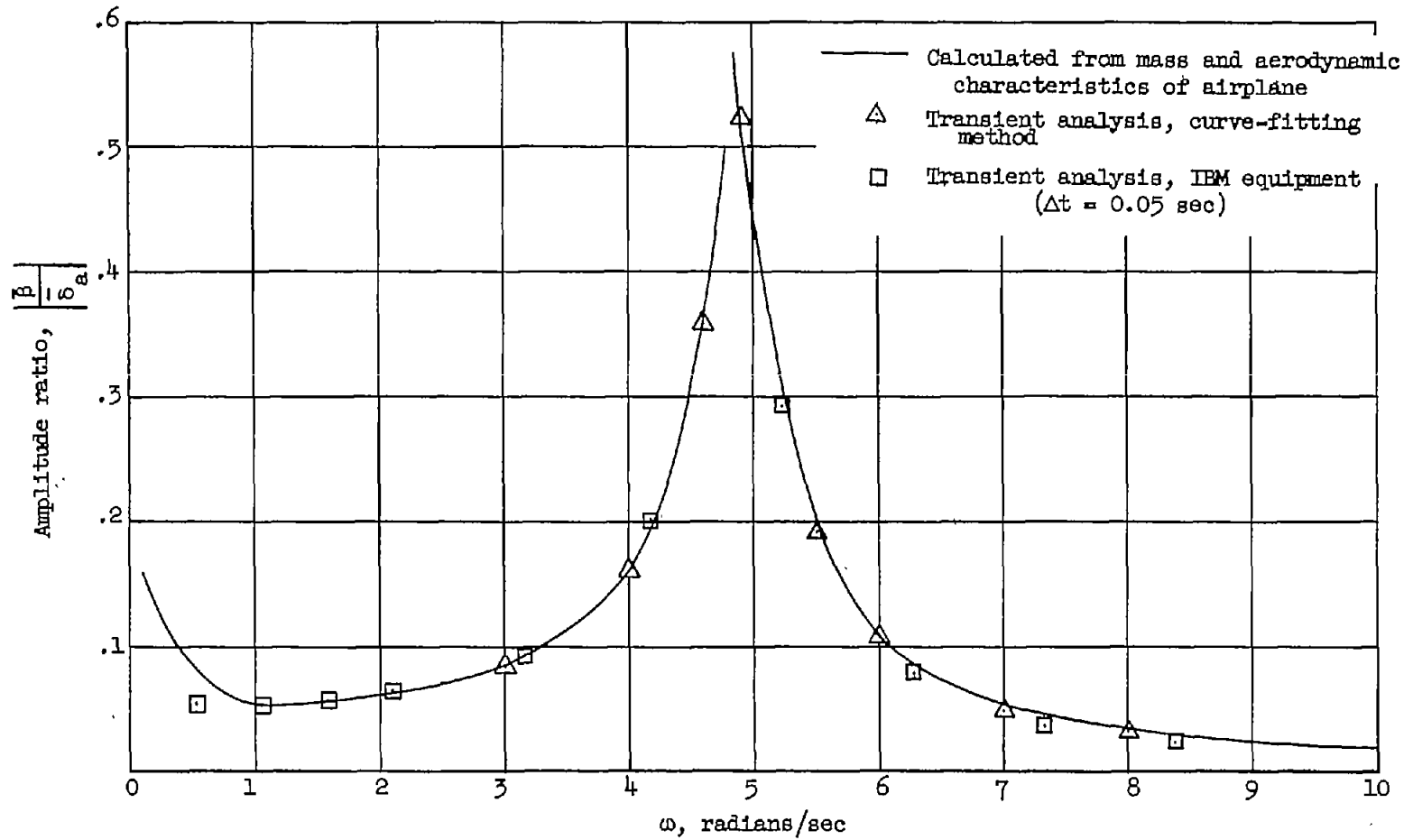
(a) Amplitude ratio \left| \frac{p}{\delta_a} \right| .
