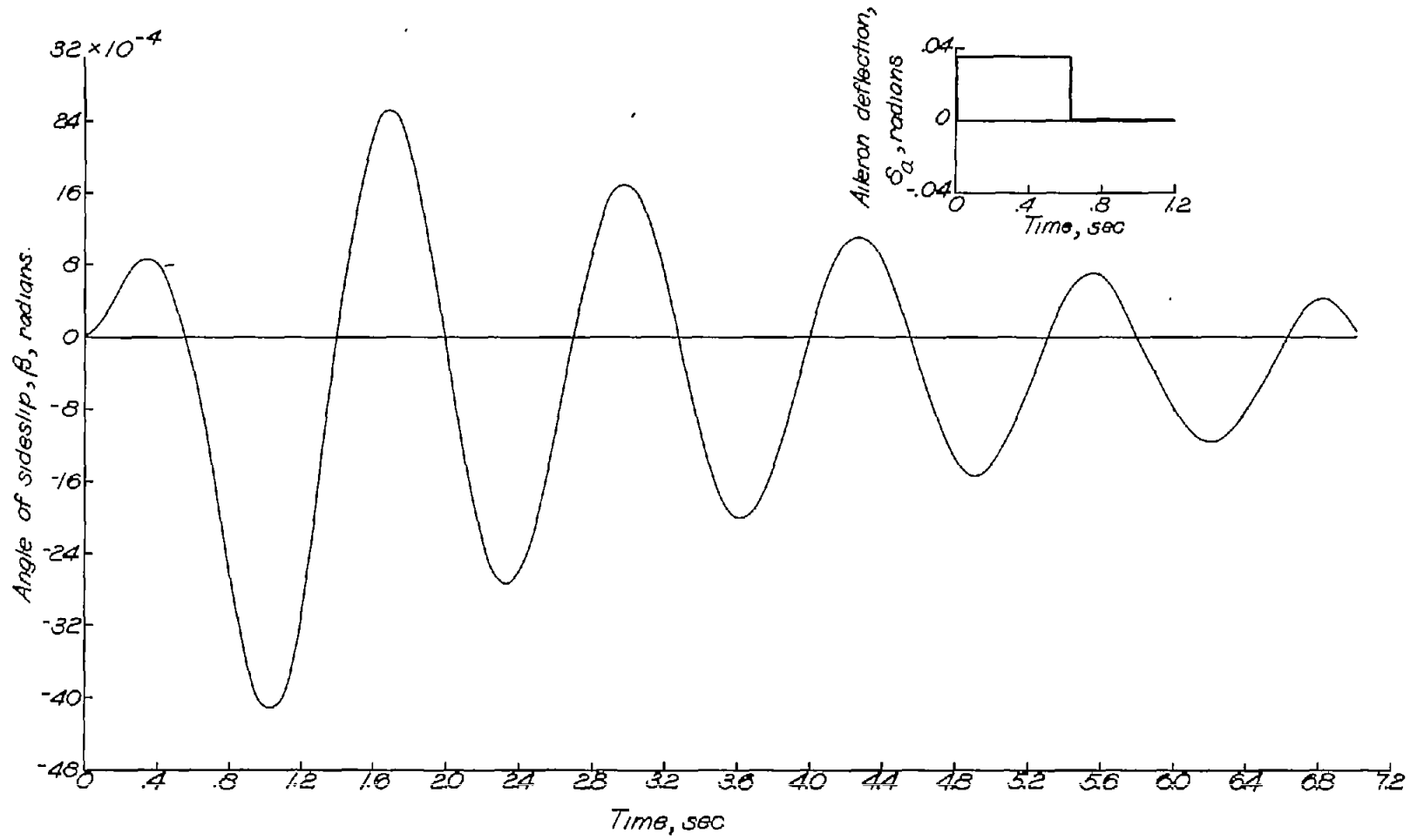
(c) Angle of sideslip.
