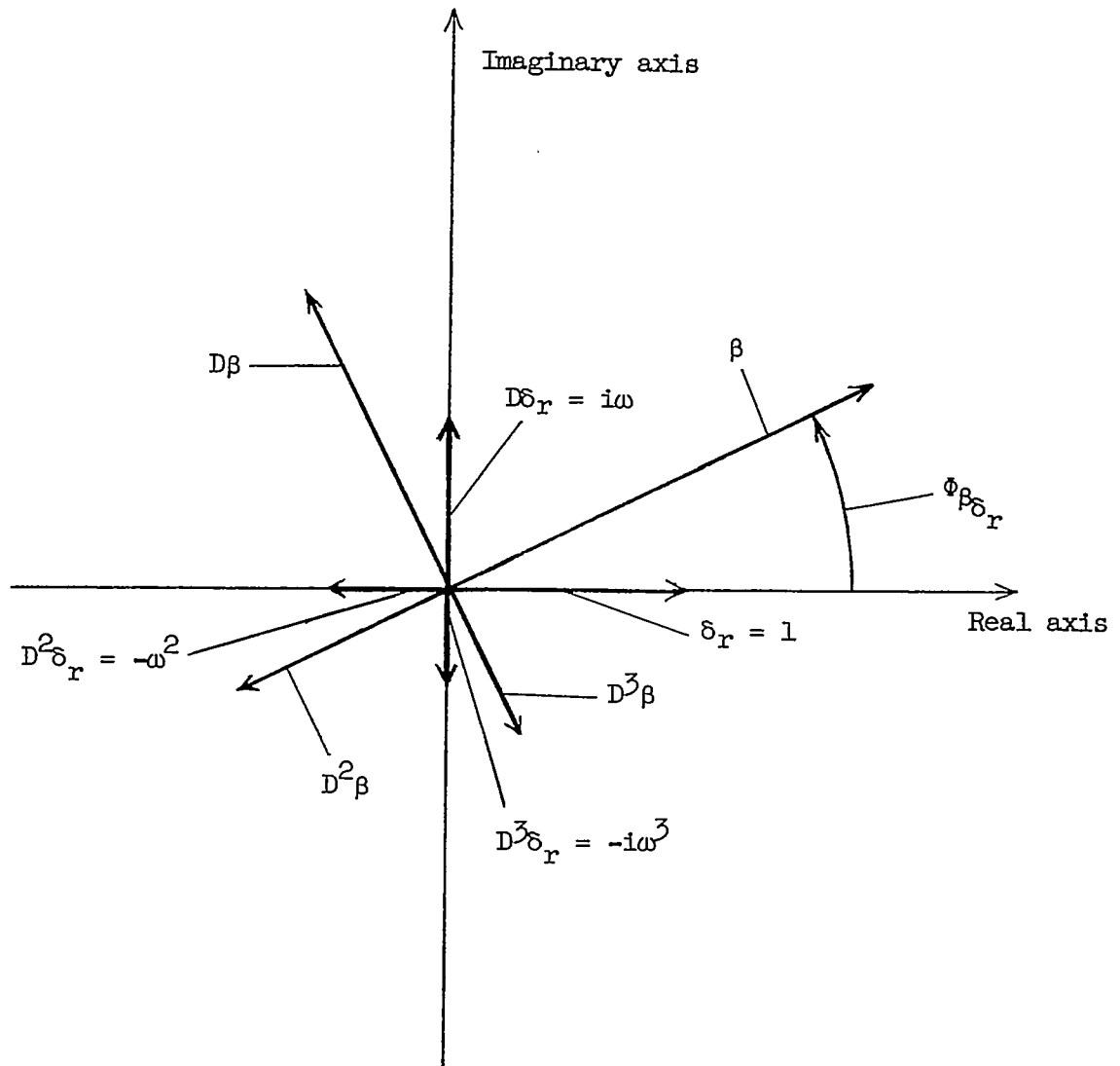
(a) Vector diagram showing relative magnitudes and positions of input \delta_r and output \beta , and their derivatives. \omega = 0.7 radian/sec.
