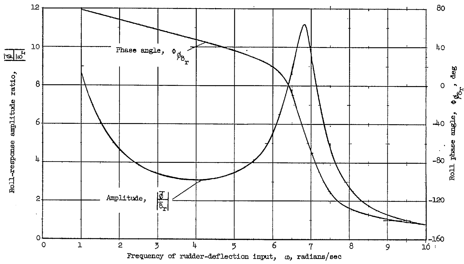
Figure 4.- Frequency response in roll due to rudder-deflection input for rigid, high-speed airplane of example given in body of paper.
