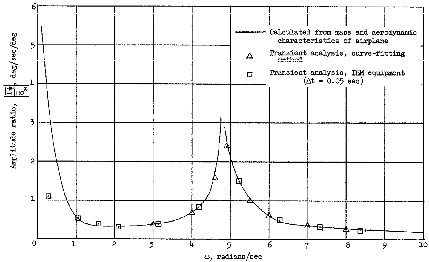
(e) Amplitude ratio \left| \frac{Dv}{\delta_a} \right| .
