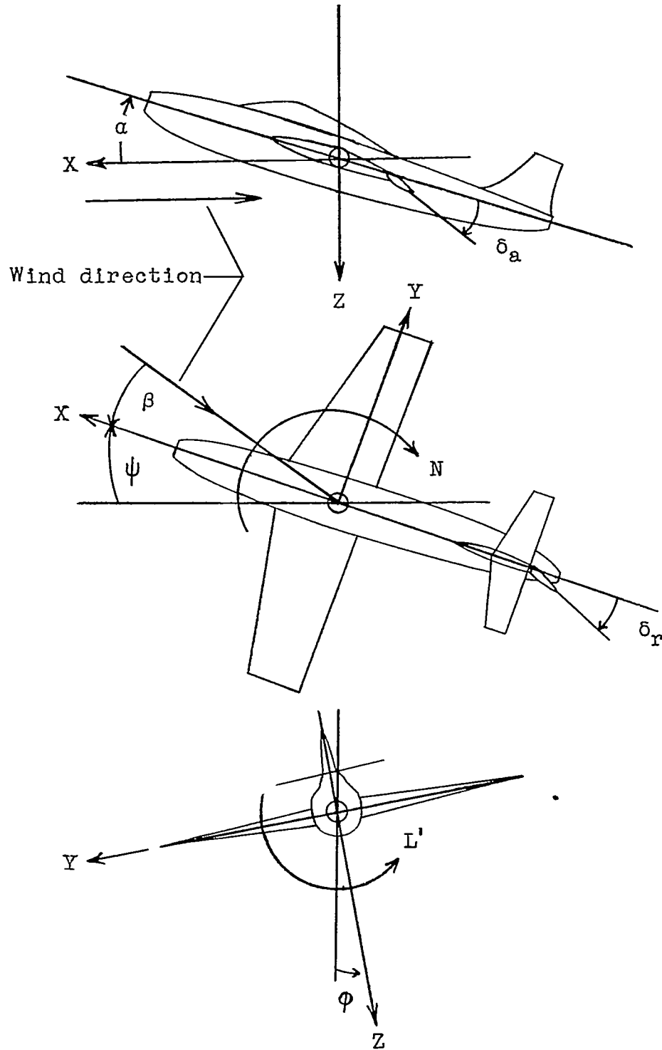
Figure 1.- Stability axis system showing positive directions.
