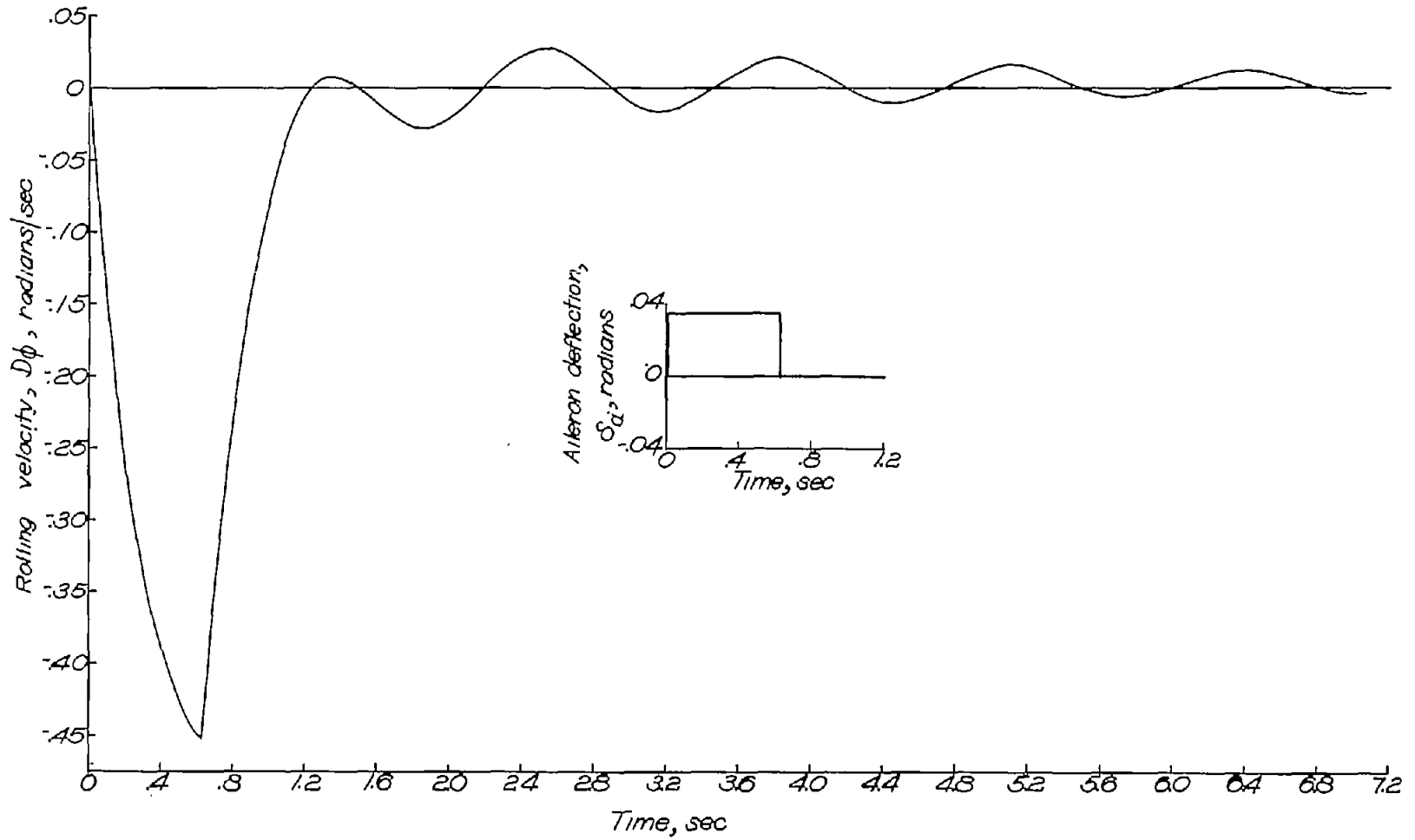
(a) Rolling velocity.
