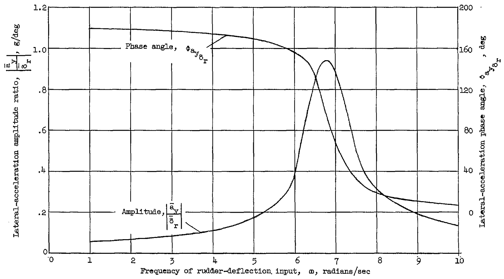
Figure 6.- Frequency response in lateral acceleration due to rudder-deflection input for rigid, high-speed airplane of example given in body of paper.
