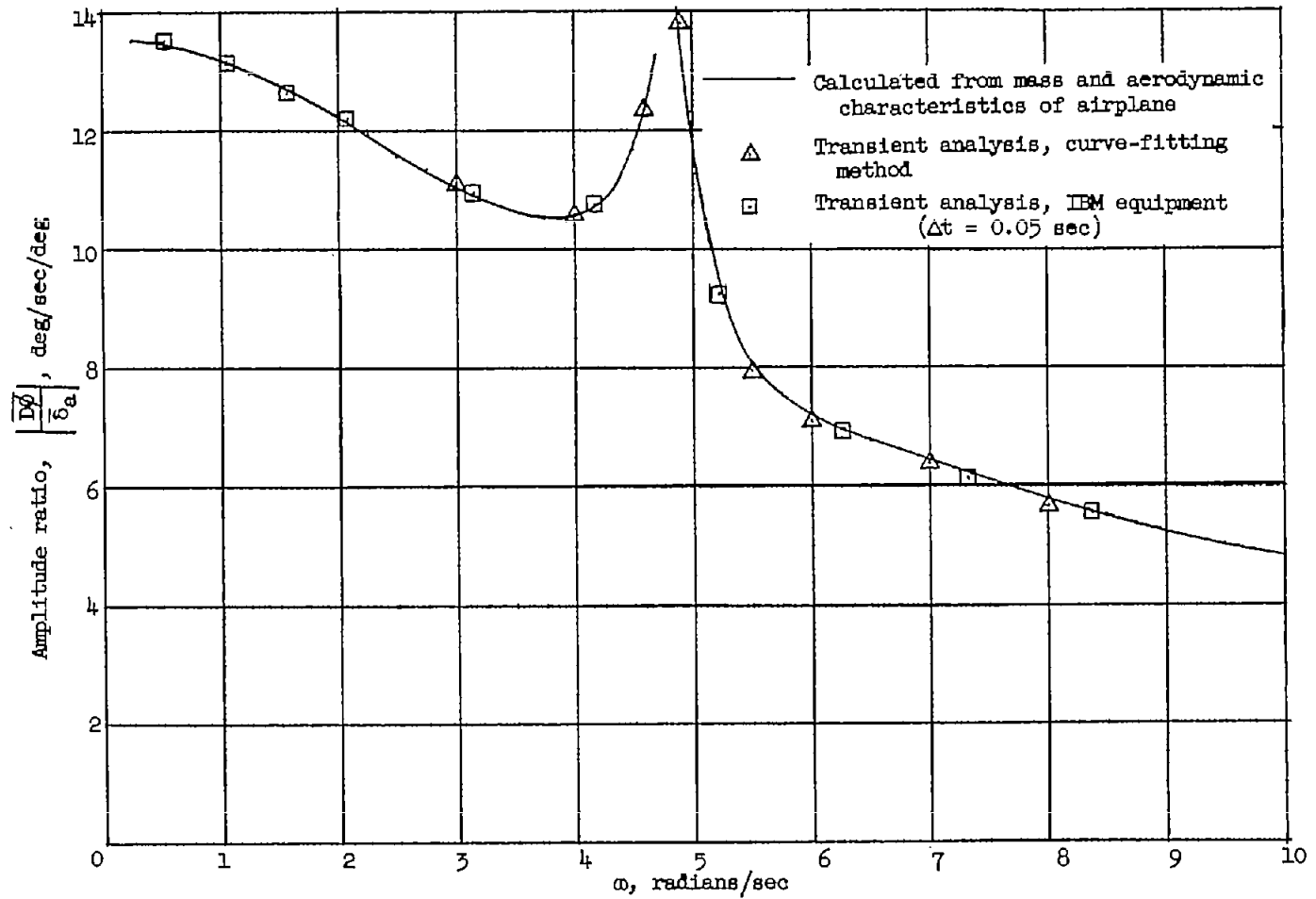
(c) Amplitude ratio \left| \frac{D\phi}{\delta_a} \right| .
