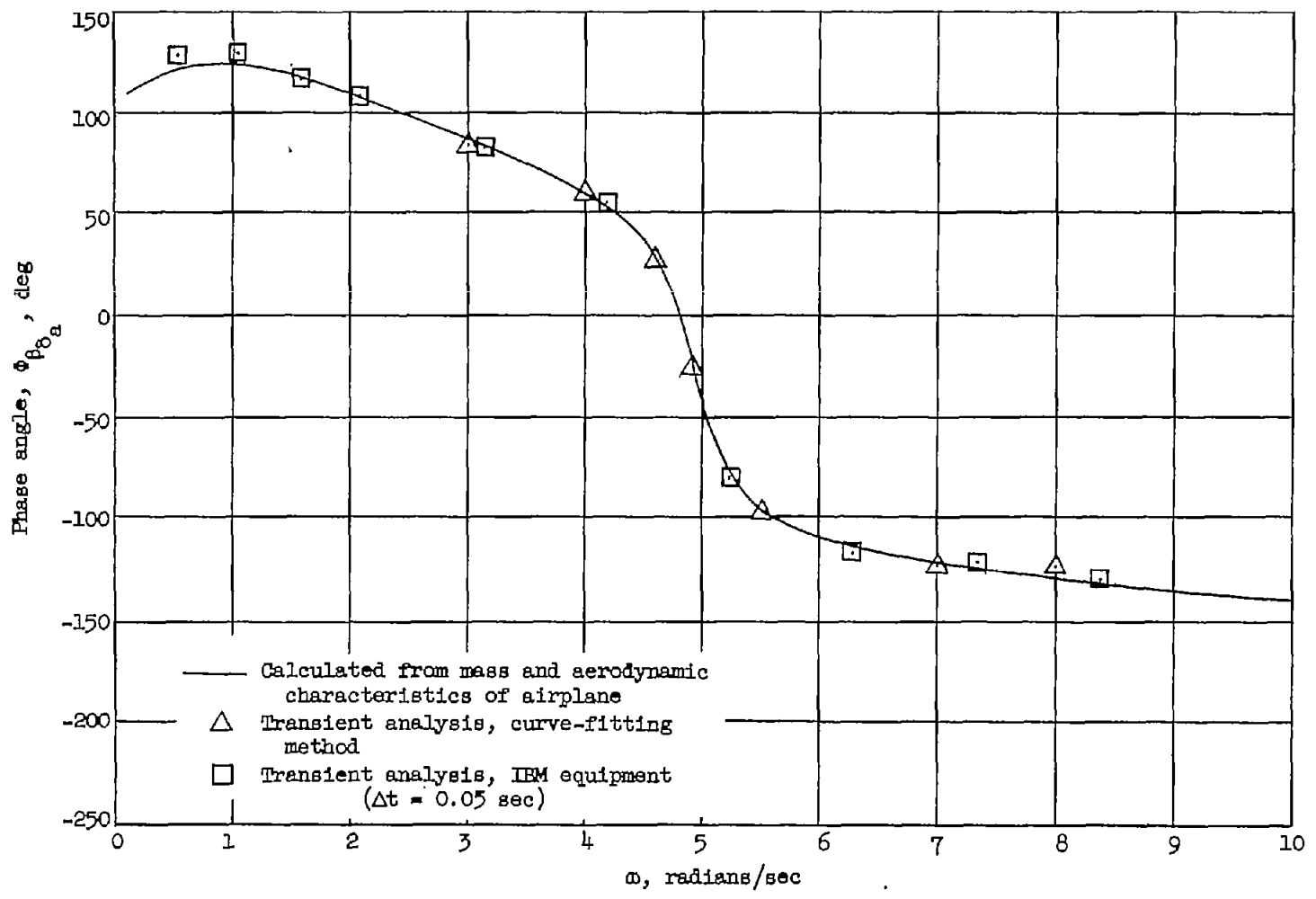
(b) Phase angle \phi_{\beta\delta_a} .
