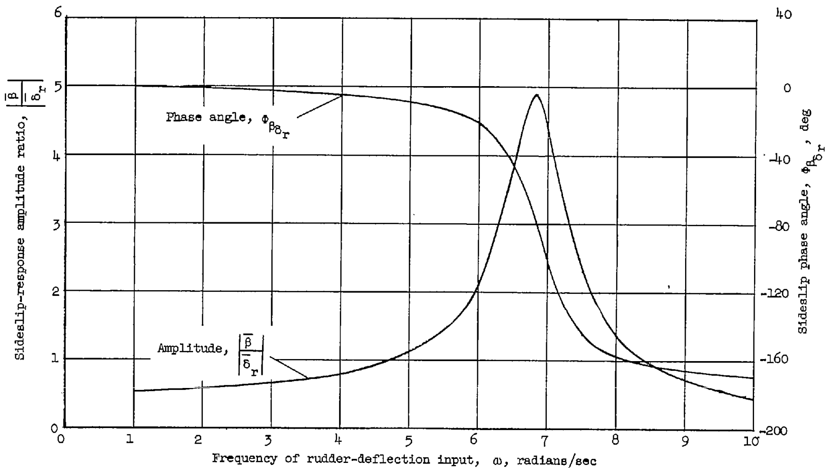
Figure 3.- Frequency response in sideslip due to rudder-deflection input for rigid, high-speed airplane of example given in body of paper.
