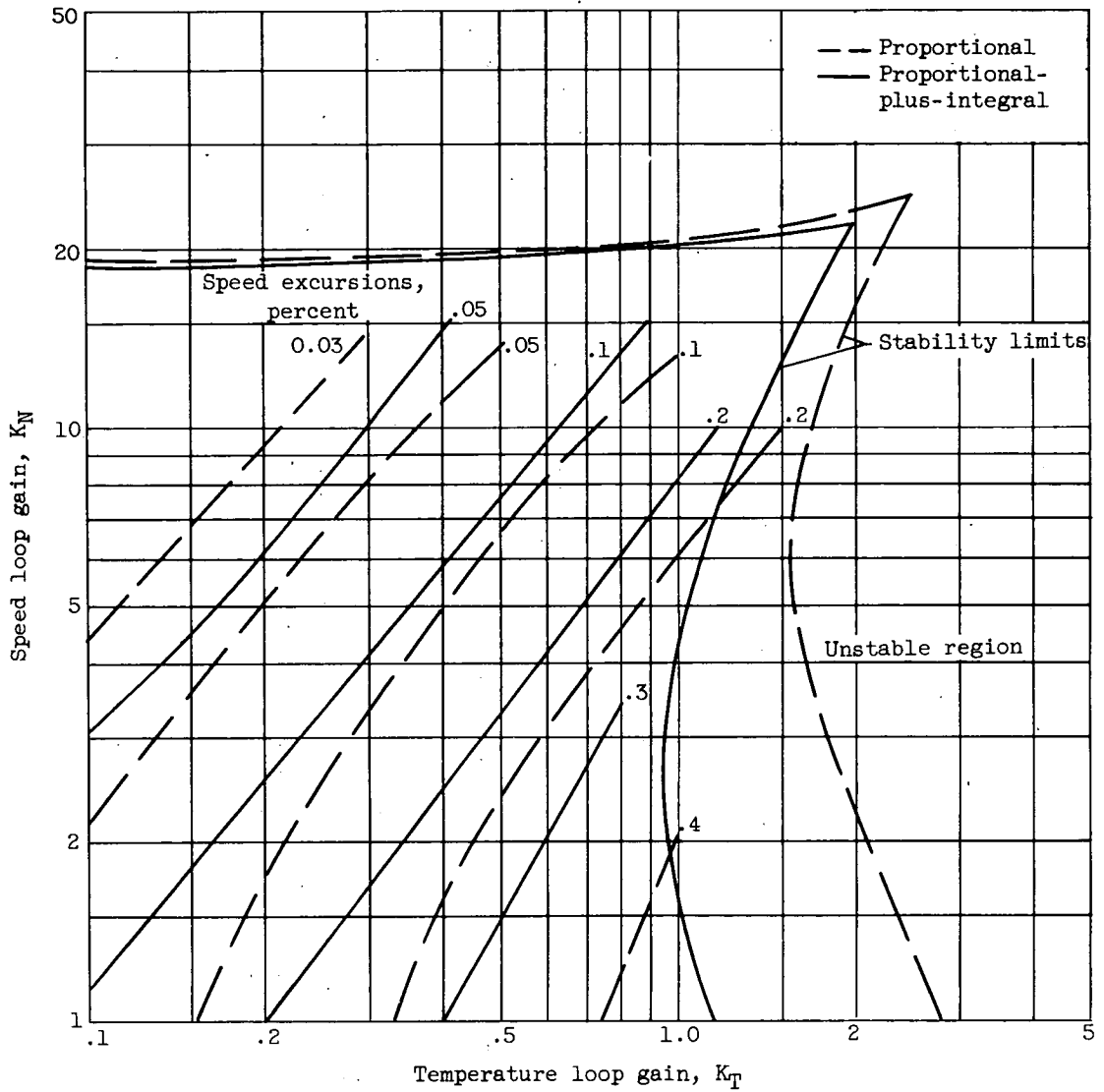
Figure 5. - Maximum speed excursion characteristics of proportional control compared with proportional-plus-integral control.
