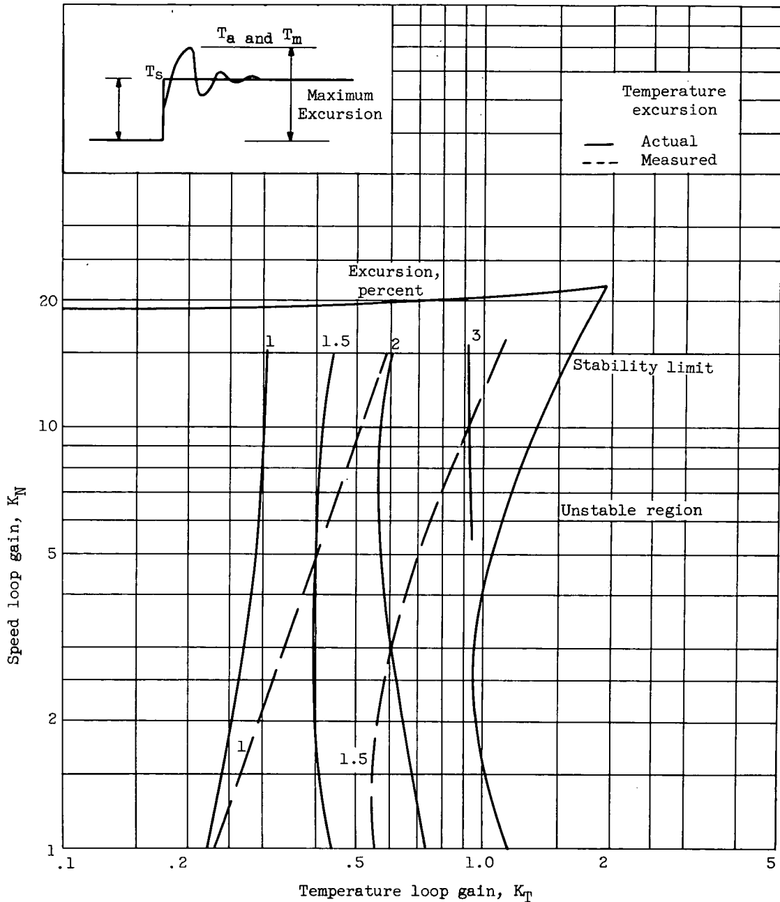
Figure 9. Contour lines of excursions in actual and measured temperature for proportional-plus-integral control superimposed on stability map.
