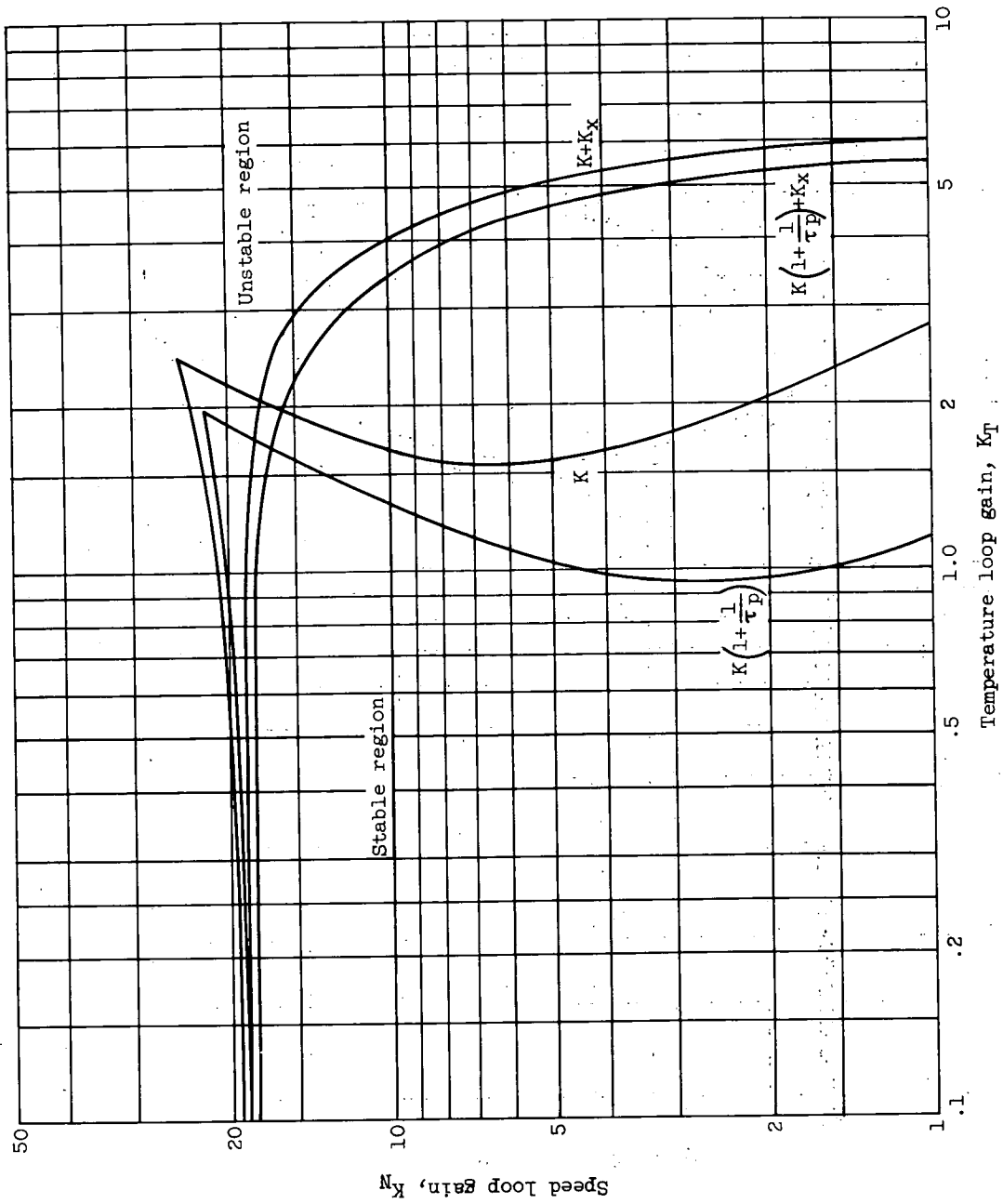
Figure 4.- Comparison of stability limits obtained with four configurations studied in detail. K_x denotes partial compensation X_A .
