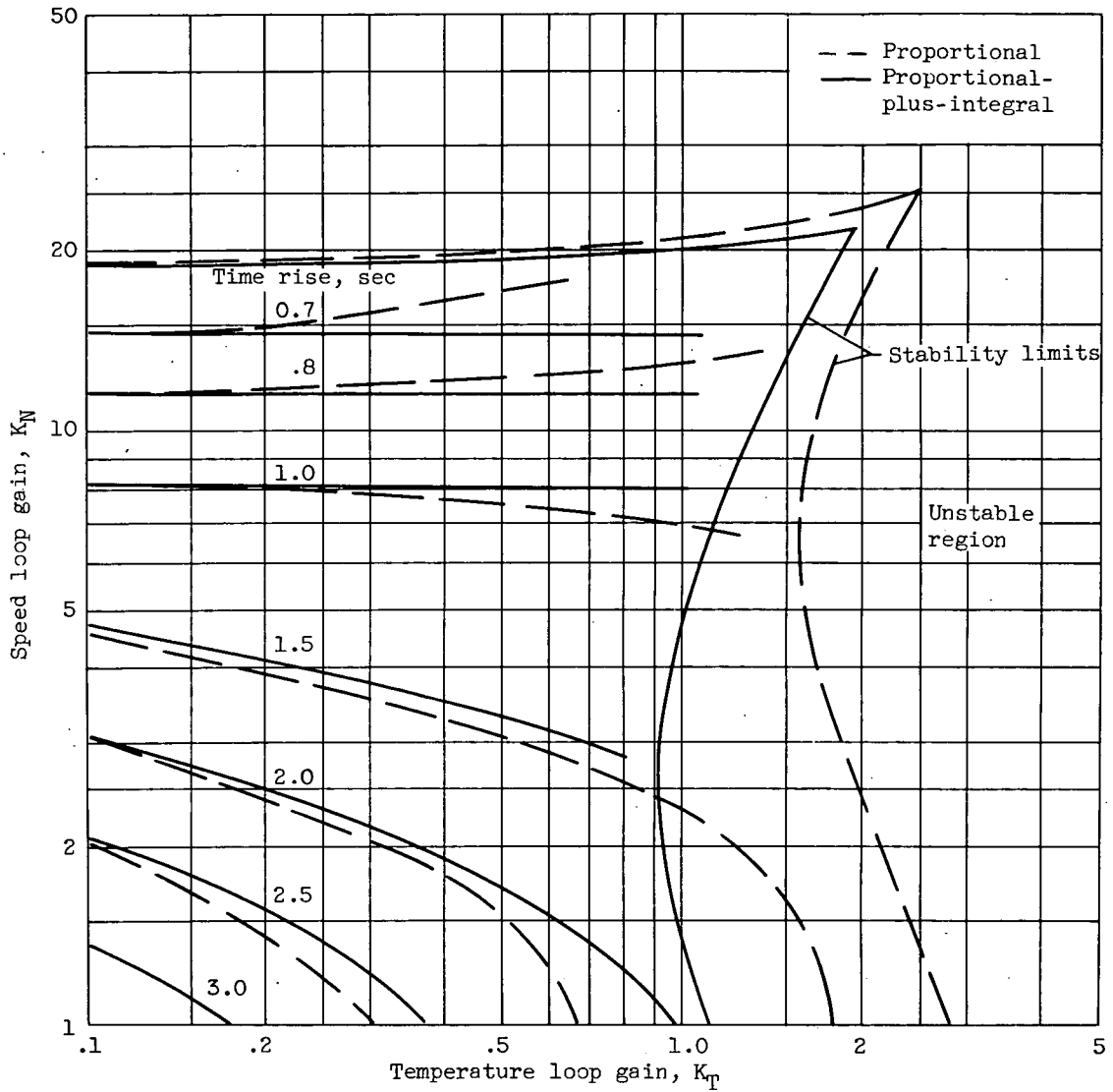
Figure 7. - Time to reach maximum speed excursion with proportional control compared with time when using proportional-plus-integral control.
