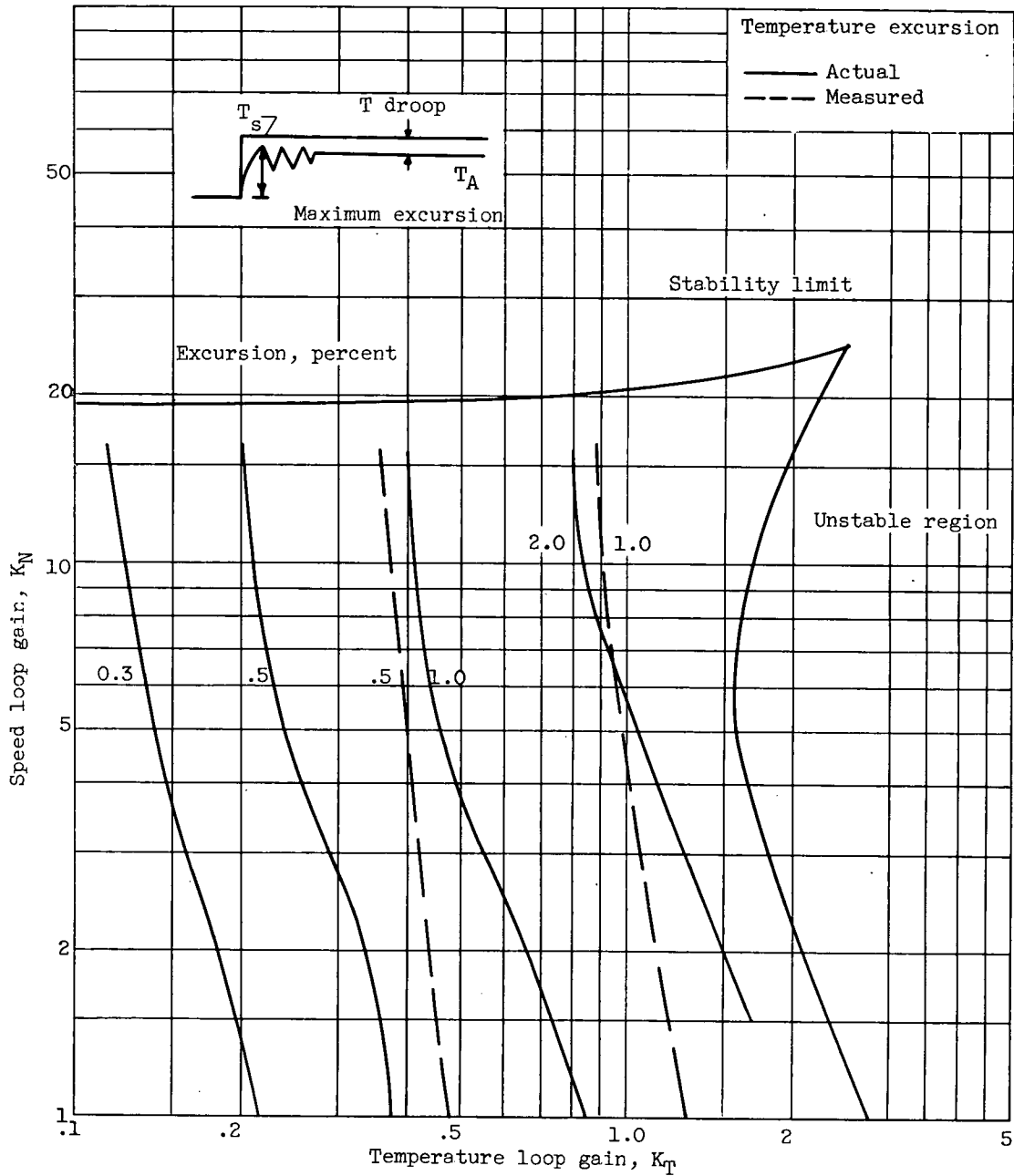
Figure 8. - Proportional control contour lines of actual and measured temperature excursions on stability limit map.
