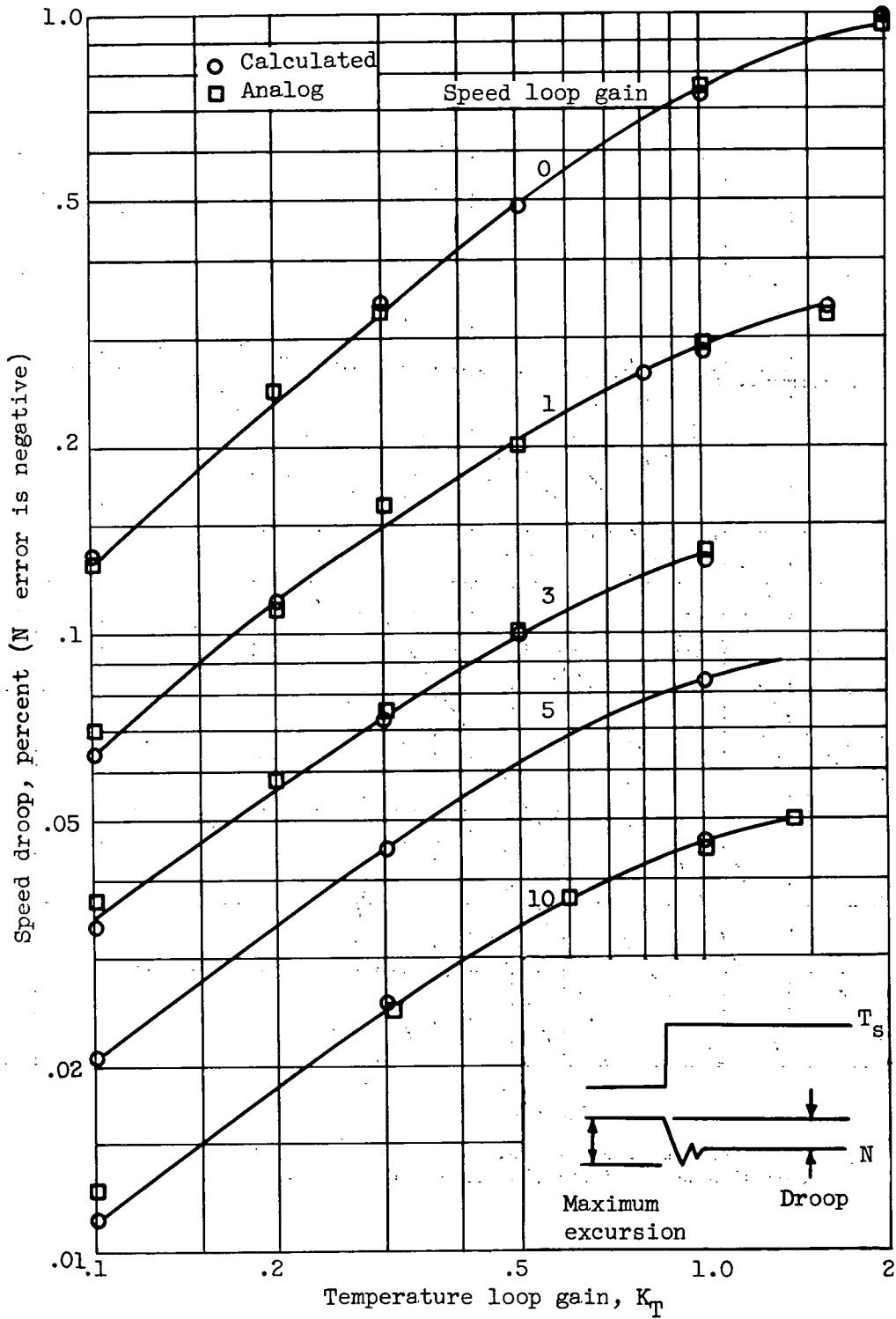
Figure 6. - Speed droop in proportional control with disturbance in set temperature.
