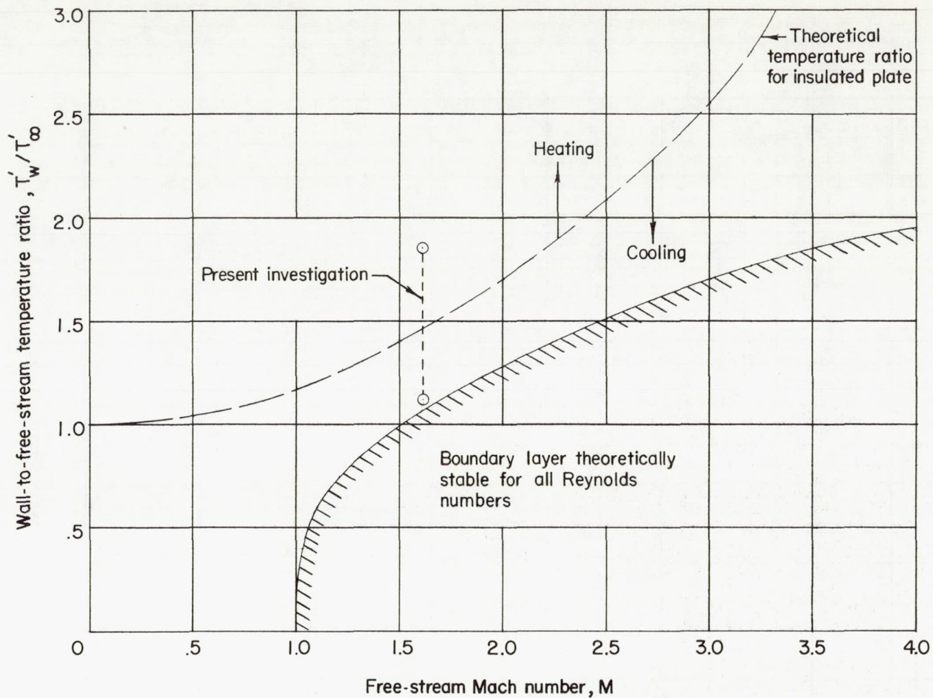
Figure 8.- Heating and cooling range covered in boundary-layer-transition investigation on NACA RM-10 model. Theoretical curve from reference 7.
