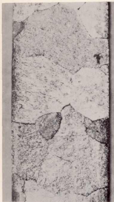
(a) Aluminum I, 0.0004 percent iron.
