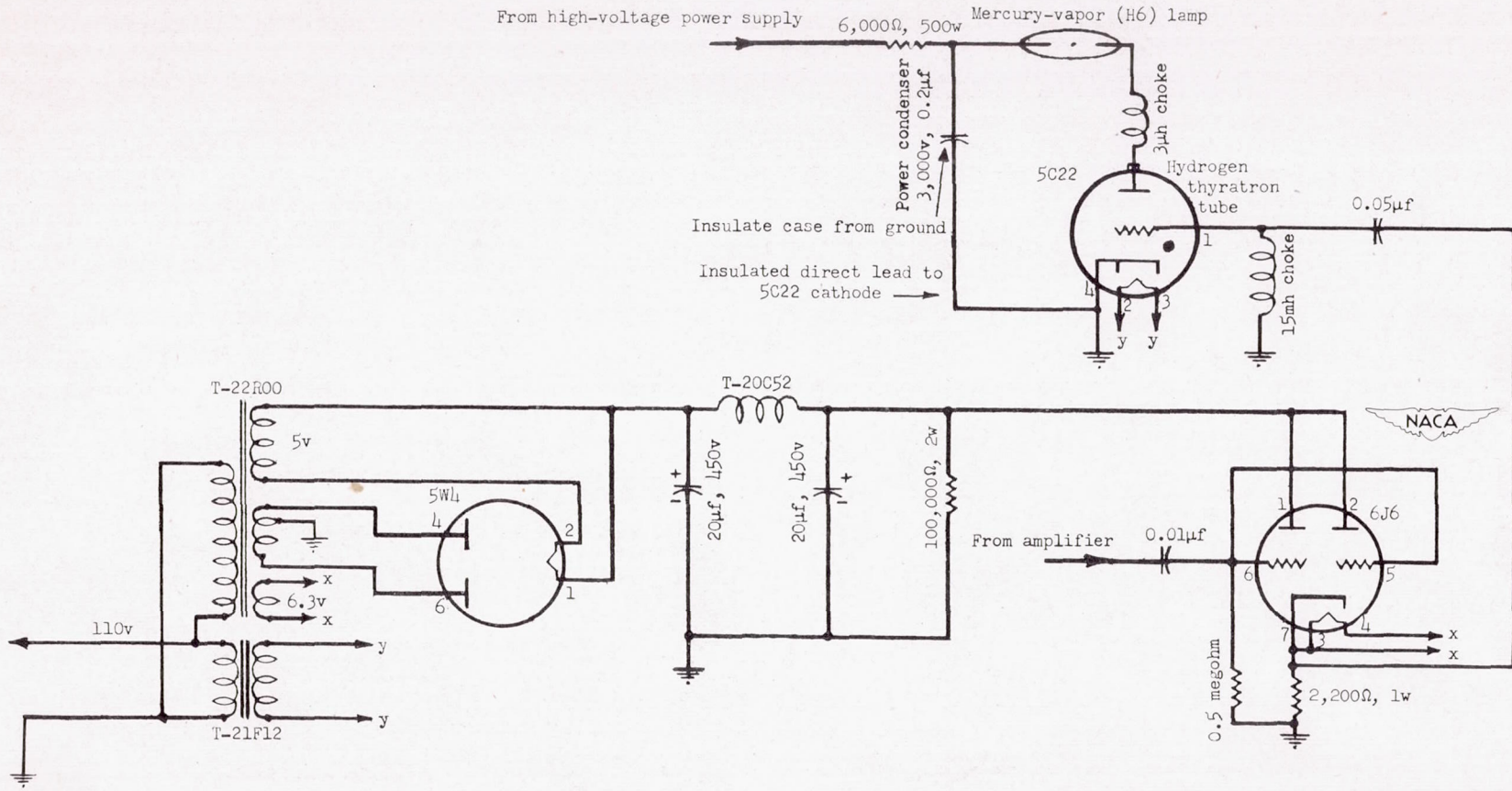
Figure 4.- Modulator.
