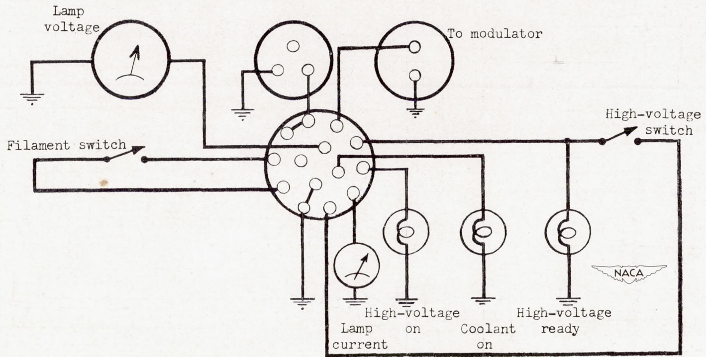
Figure 5.- Control unit.
