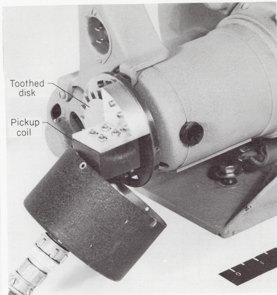
(b) Generator cover removed.
