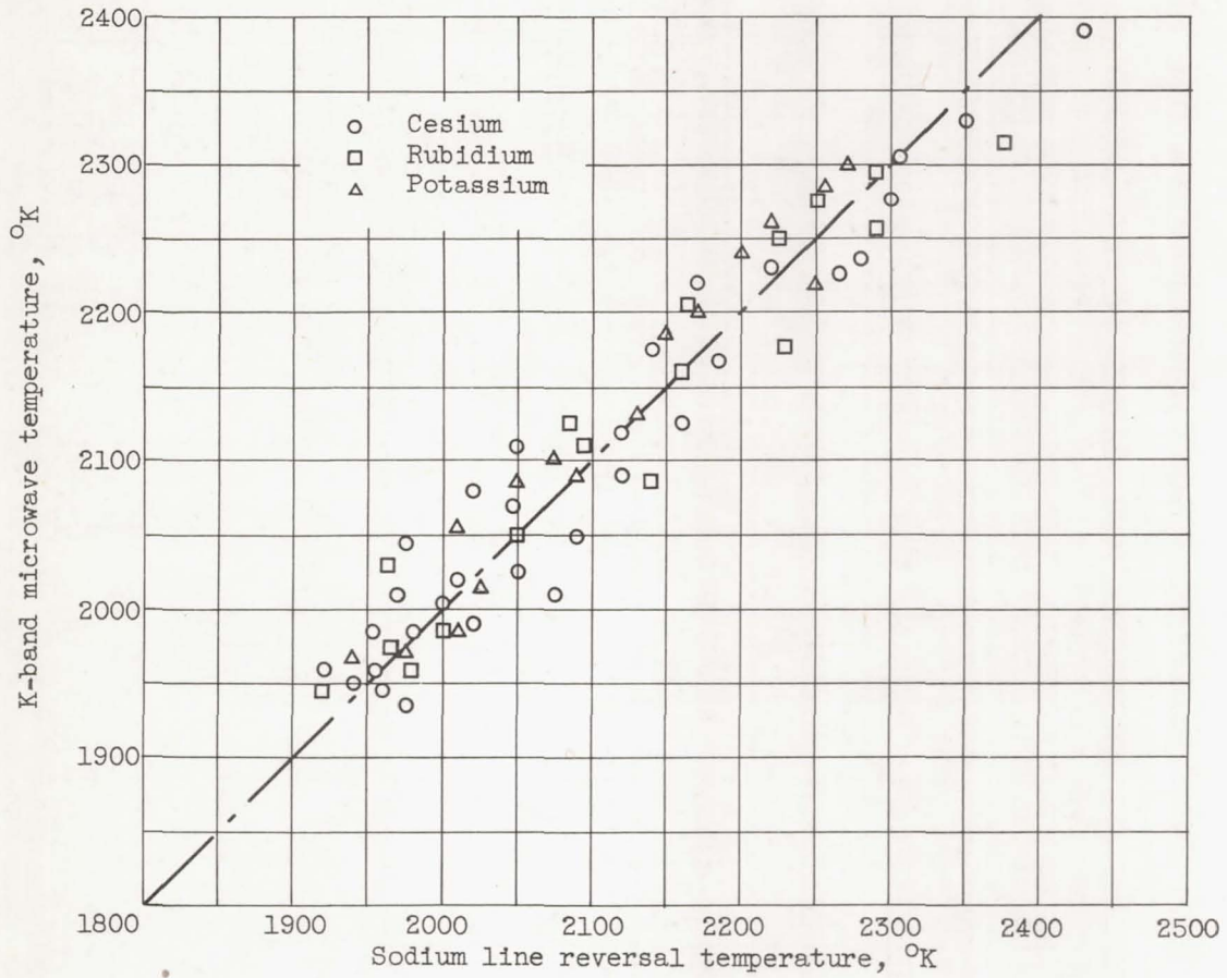
(a) K-band microwaves, obtained for experimental ionization potentials for cesium, rubidium, and potassium.
