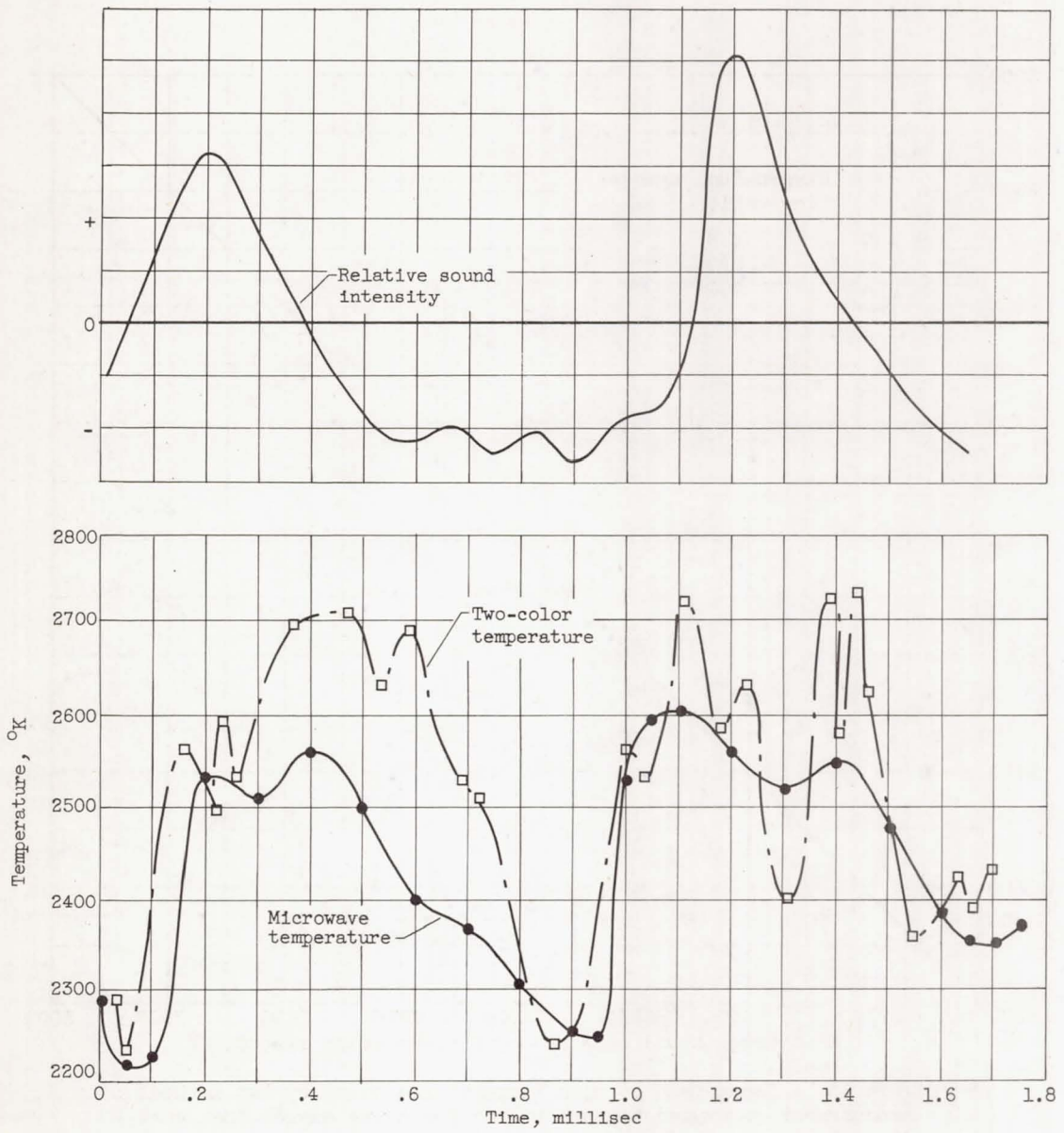
(a) Screaming at approximately 1000 cycles per second.
