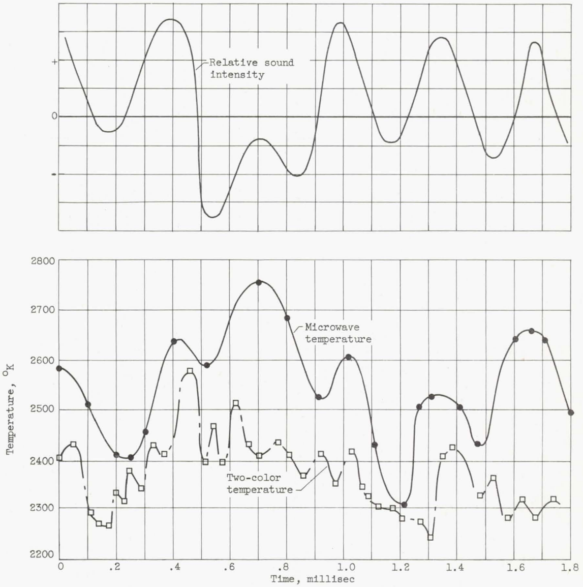
(b) Screaming at approximately 3000 cycles per second.
