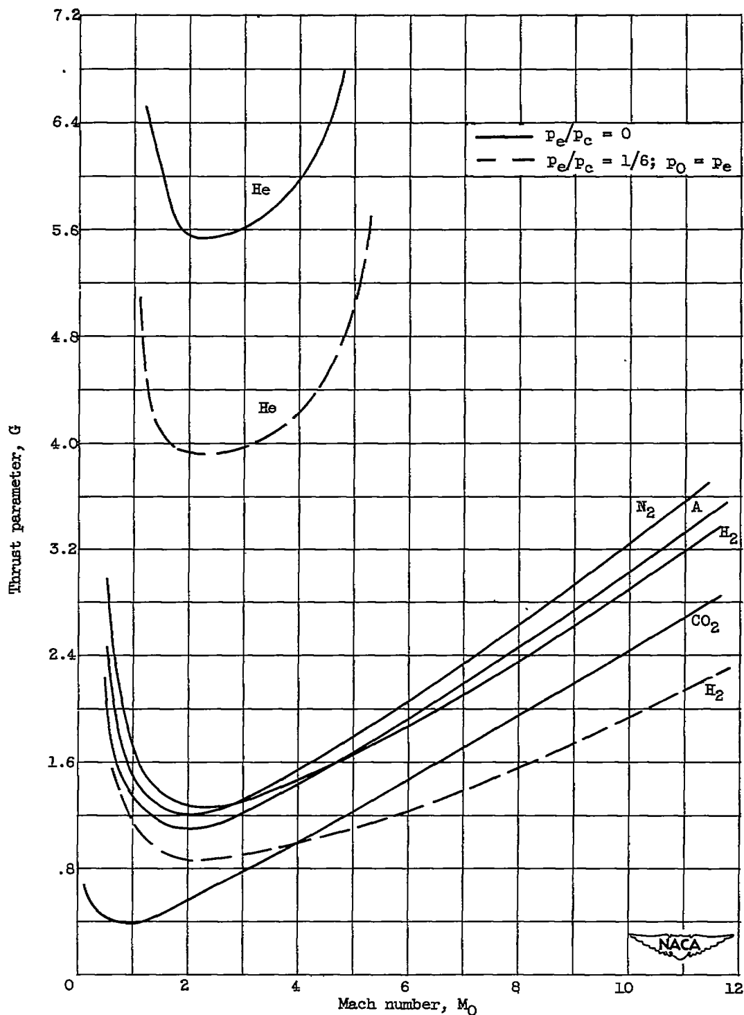
Figure 3. - Continued. Ratio of generated thrust to friction drag as function of Mach number for cooled external surfaces. T_0 = 392.4^\circ R .
