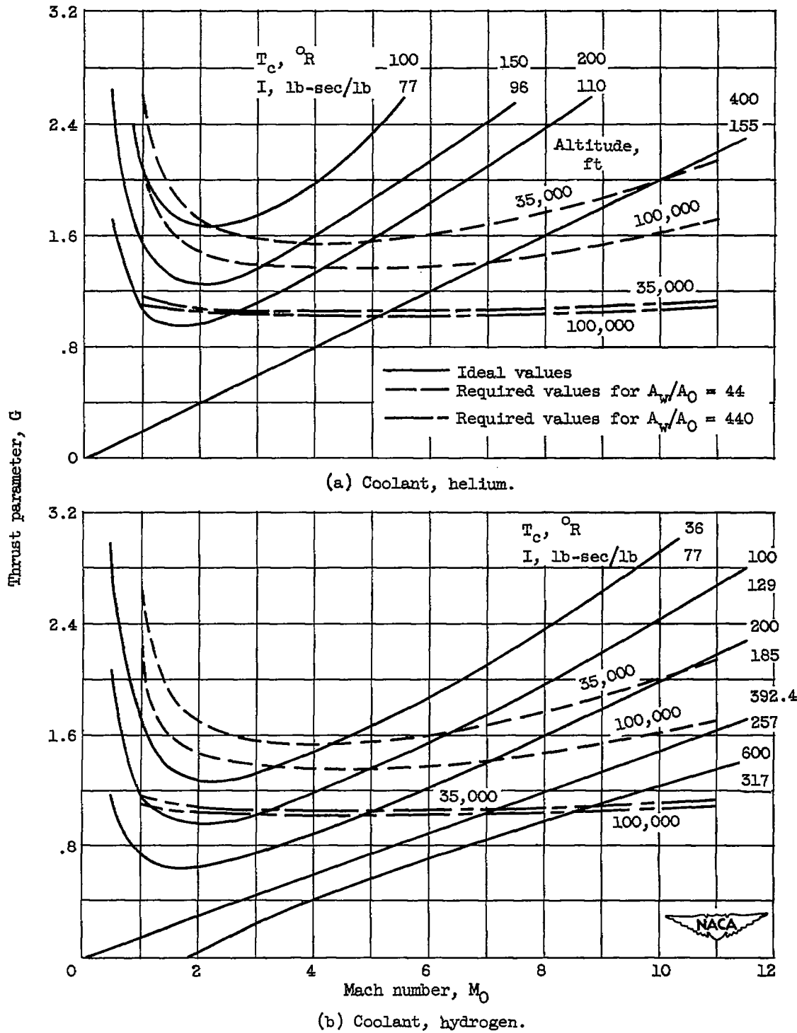
Figure 5. - Required and available values of thrust parameter G for propulsion of cone-cylinder body. Turbulent boundary layer; p_e/p_o = 0 ; T_w = T_c .
