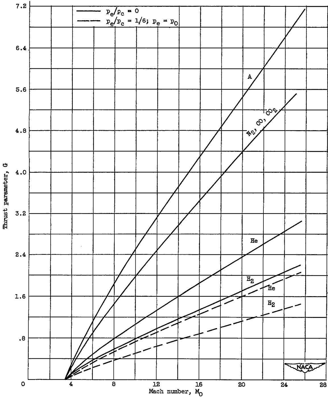
Figure 3. - Concluded. Ratio of generated thrust to friction drag as function of Mach number for cooled external surfaces. T_0 = 392.4^\circ R.
