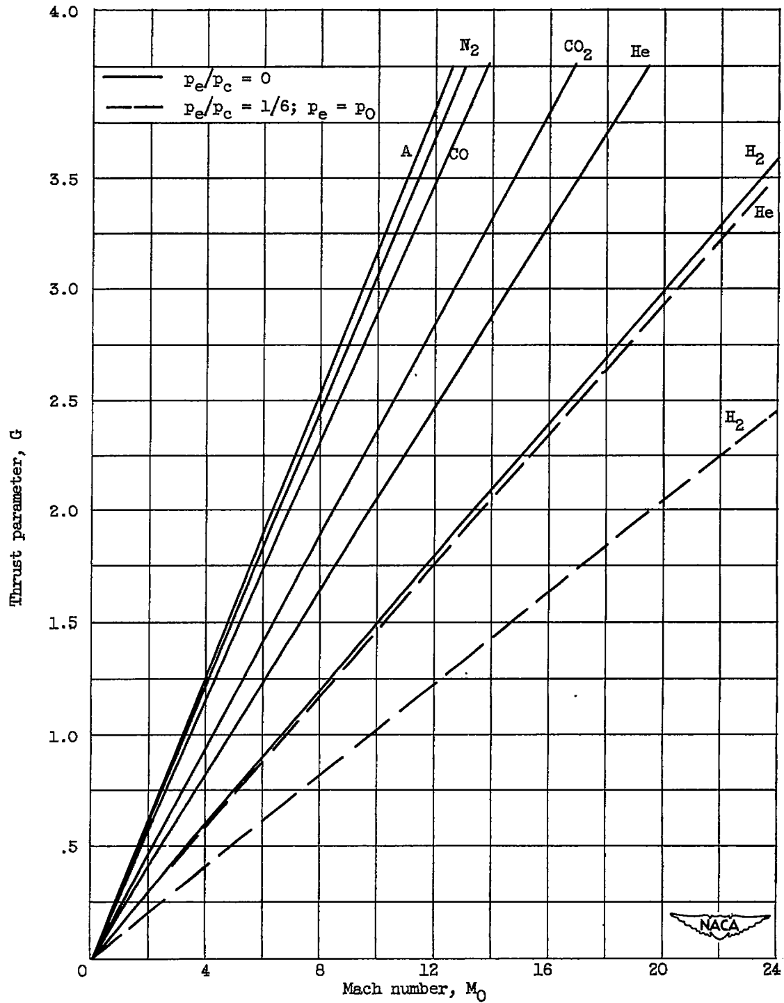
Figure 3. - Ratio of generated thrust to friction drag as function of Mach number for cooled external surfaces. T_0 = 392.4^\circ R .
