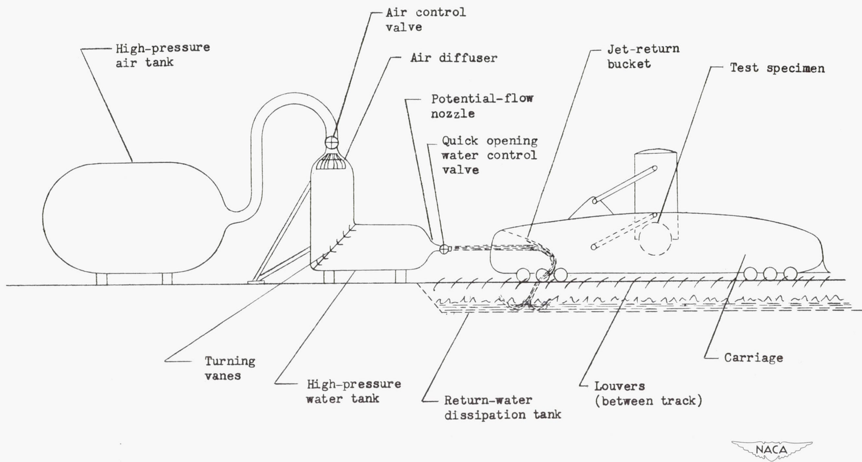
Figure 1.- Schematic drawing of hydraulic catapult system.
