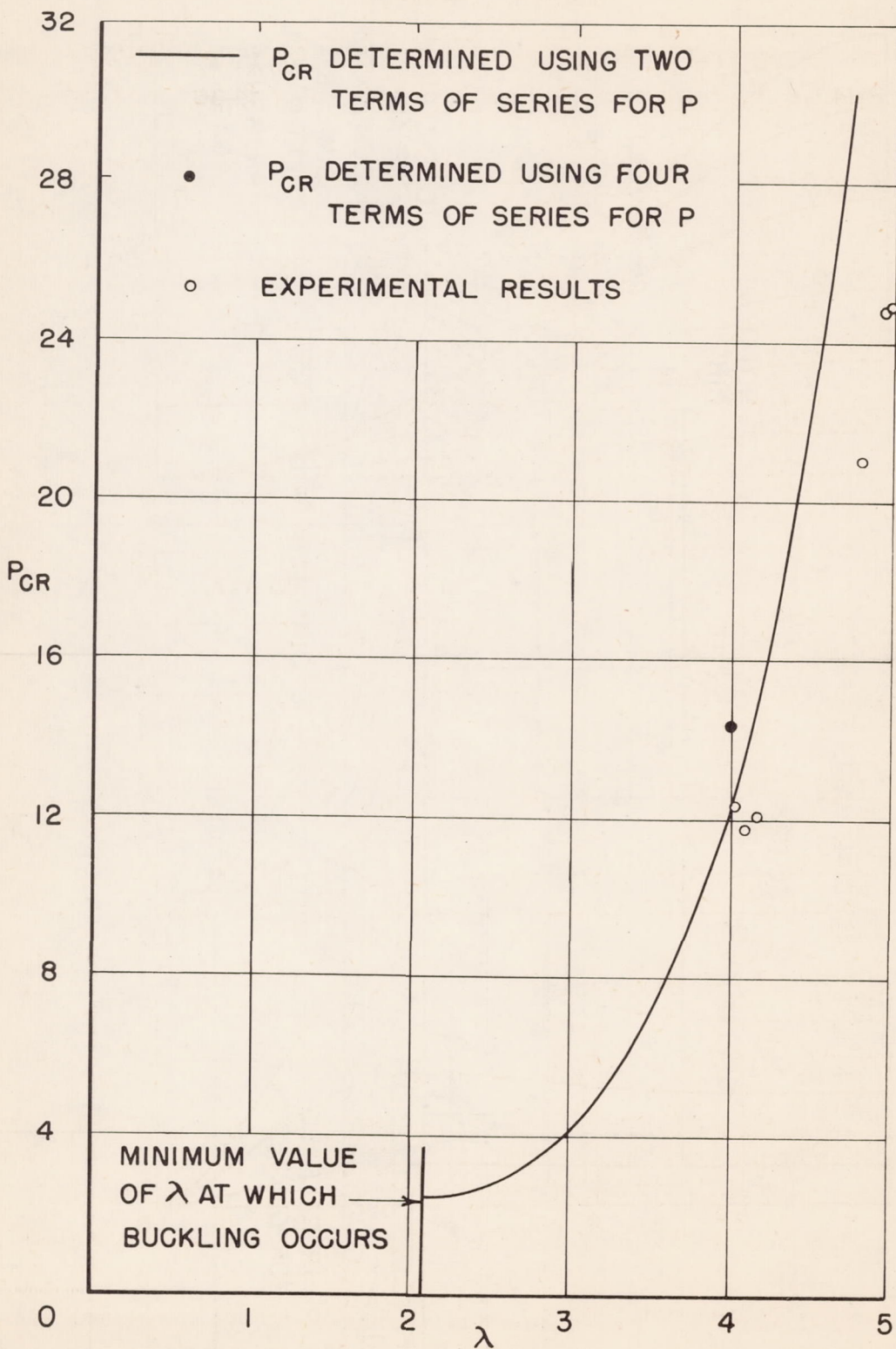
Figure 13.- Comparison of experimental buckling loads with theoretical values.
