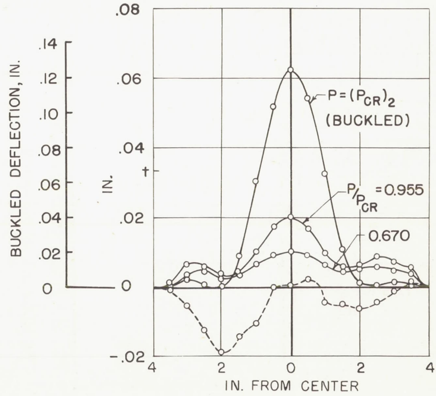
(f) Specimen 16; \lambda = 8.98 ; h = 0.410 inch; P_{cr} = 254.5 ; oil loading.
