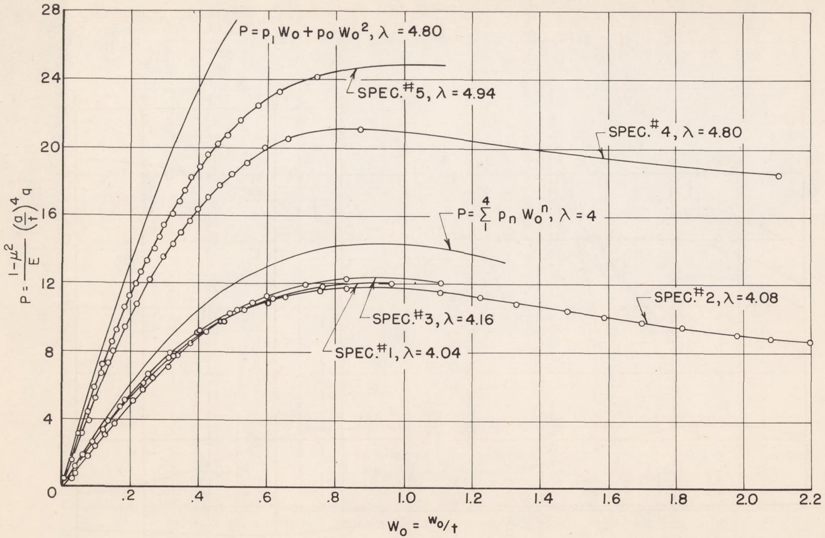
Figure 11.- Comparison of experimental pressure - center-deflection curves with theoretical results.
