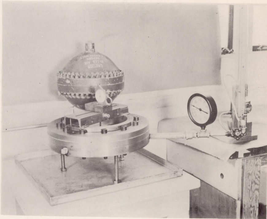
Figure 15.- View of testing fixture. L-84888
