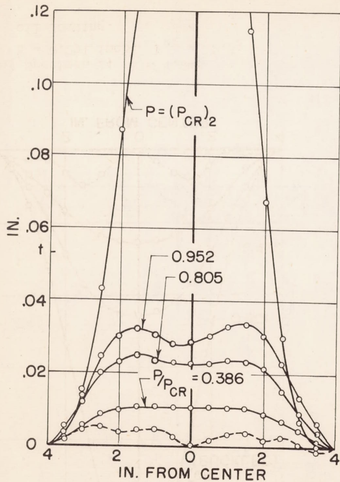
(c) Specimen 6; \lambda = 5.45 ; h = 0.240 inch; P_{cr} = 61.3 ; oil loading.
