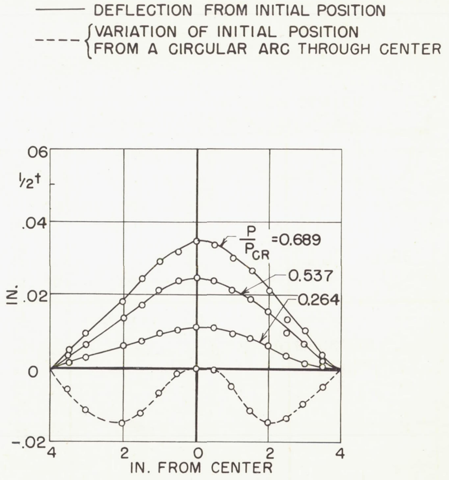
(b) Specimen 5; \lambda = 4.94 ; h = 0.376 inch; P_{cr} = 24.8 ; oil loading.
