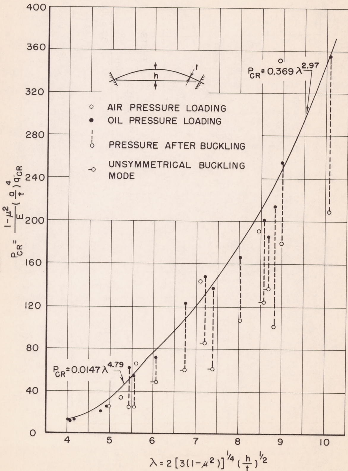
Figure 18.- Experimental results.
