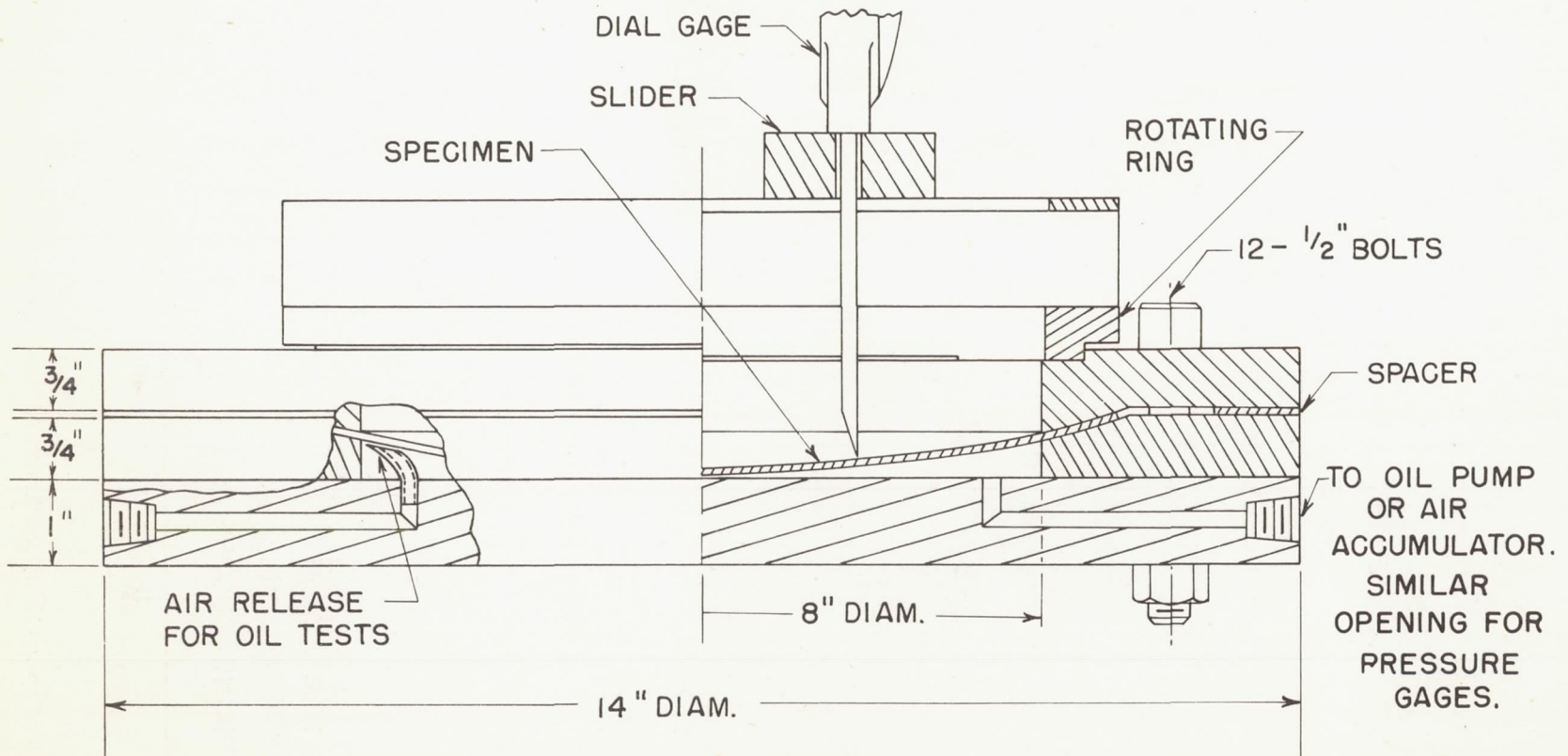
Figure 14.- Testing jig.
