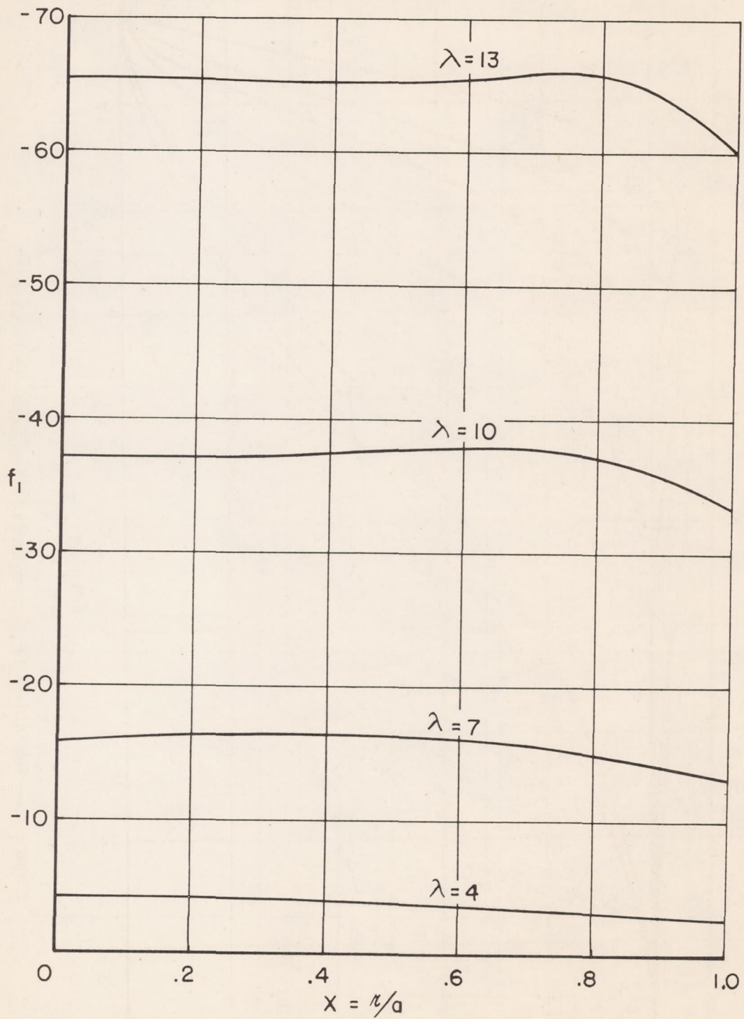
Figure 7.- Variation of linear membrane stress f_1 with \lambda .
