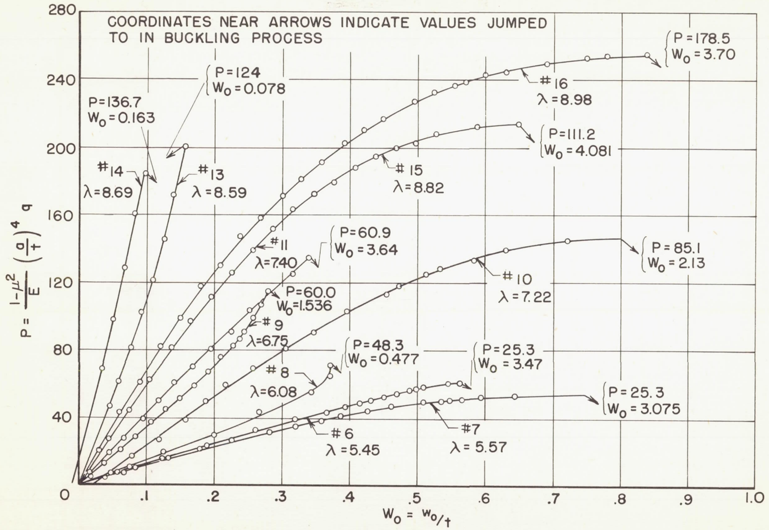
Figure 17.- Experimental pressure - center-deflection curves.
