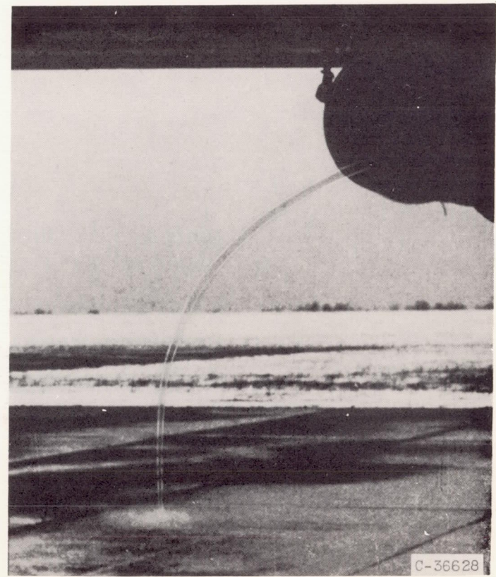
(b) Vortex 8 feet long formed at temperature of 37° F and dewpoint of 22° F (retouched).
