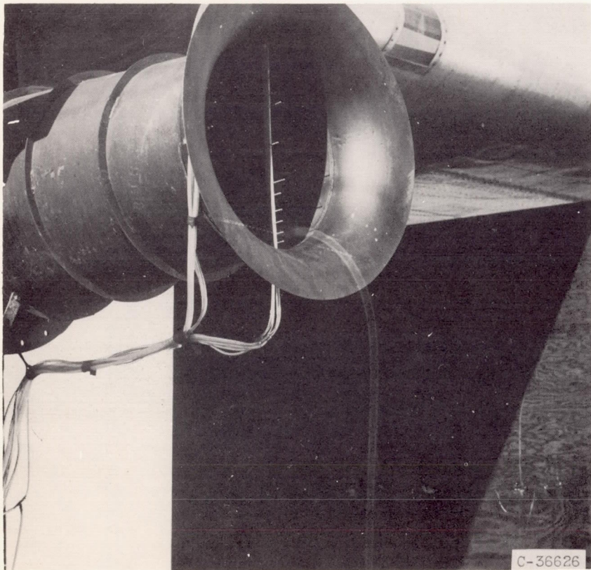
(a) Vortex 4.5 feet long formed at temperature of 76° F and dewpoint of 64° F.
