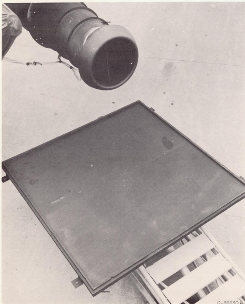
Figure 3. - Platform surface under engine inlet on which a shallow pool of water was contained for water-whirl studies.
