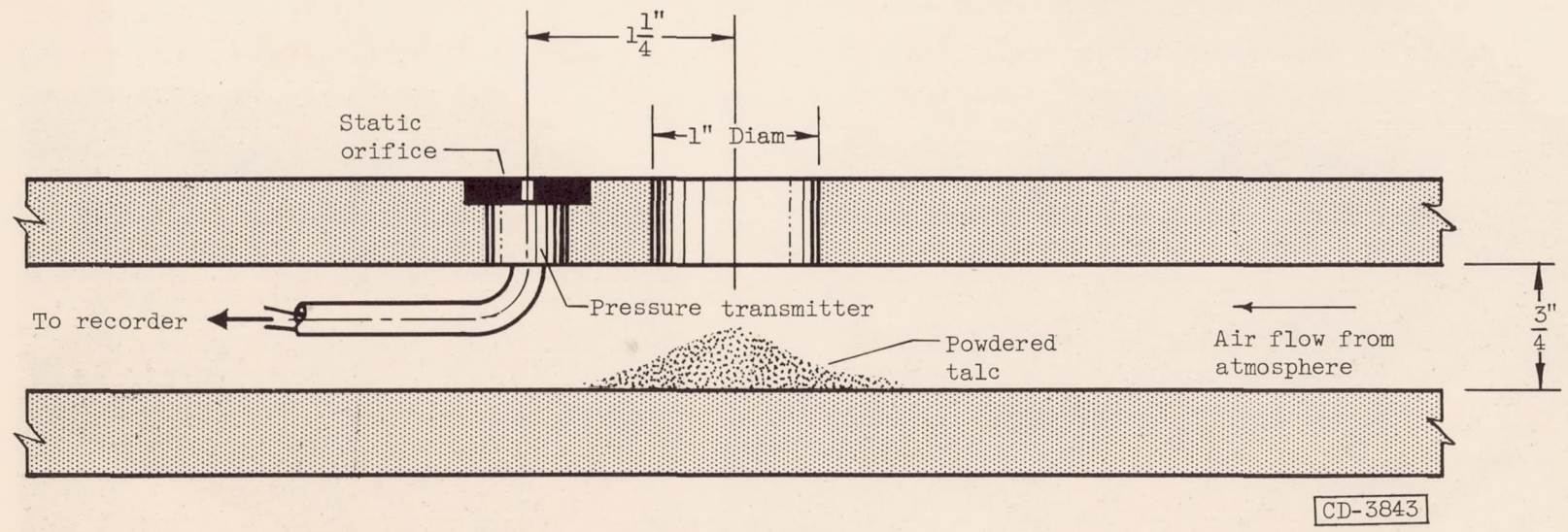
Figure 5. - Powder-release mechanism, showing schematically hole in platform surface and powder before being drawn through hole.
