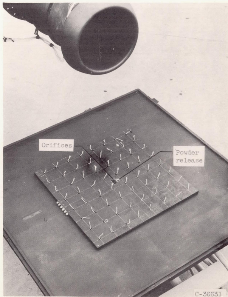
Figure 4. - Platform surface with tufts, pressure orifices, and powder release for study of pressure and velocity in vortices.
