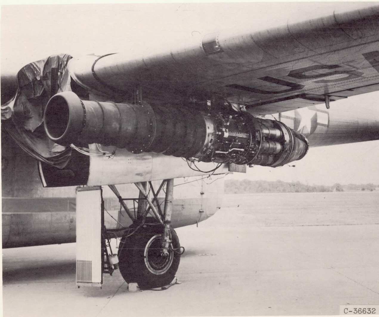
Figure 1. - Axial-flow jet engine mounted on Air Force cargo airplane for study of inlet vortices.
