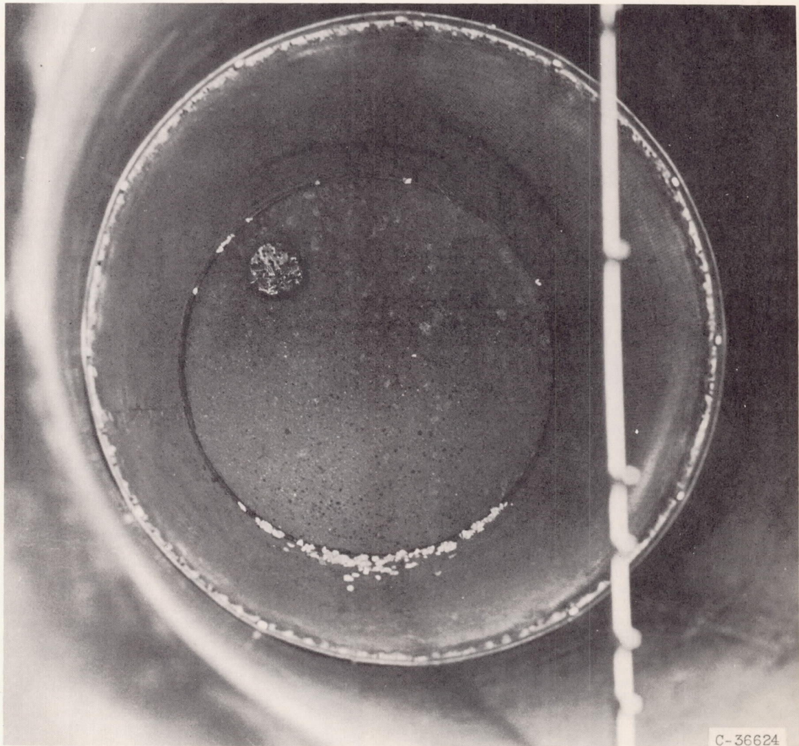
Figure 12. - Pebbles projected into engine inlet duct from platform surface by inlet vortex. (A screen prevented entrance of pebbles into engine.)
