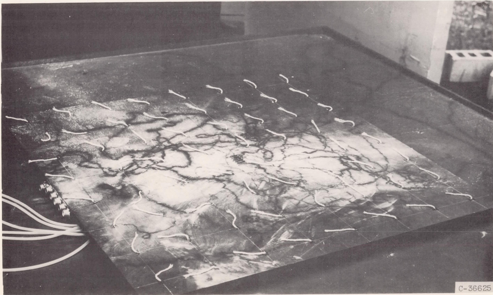
Figure 10. - Paths of vortex marked on platform surface by powdered talc in typical test run.
