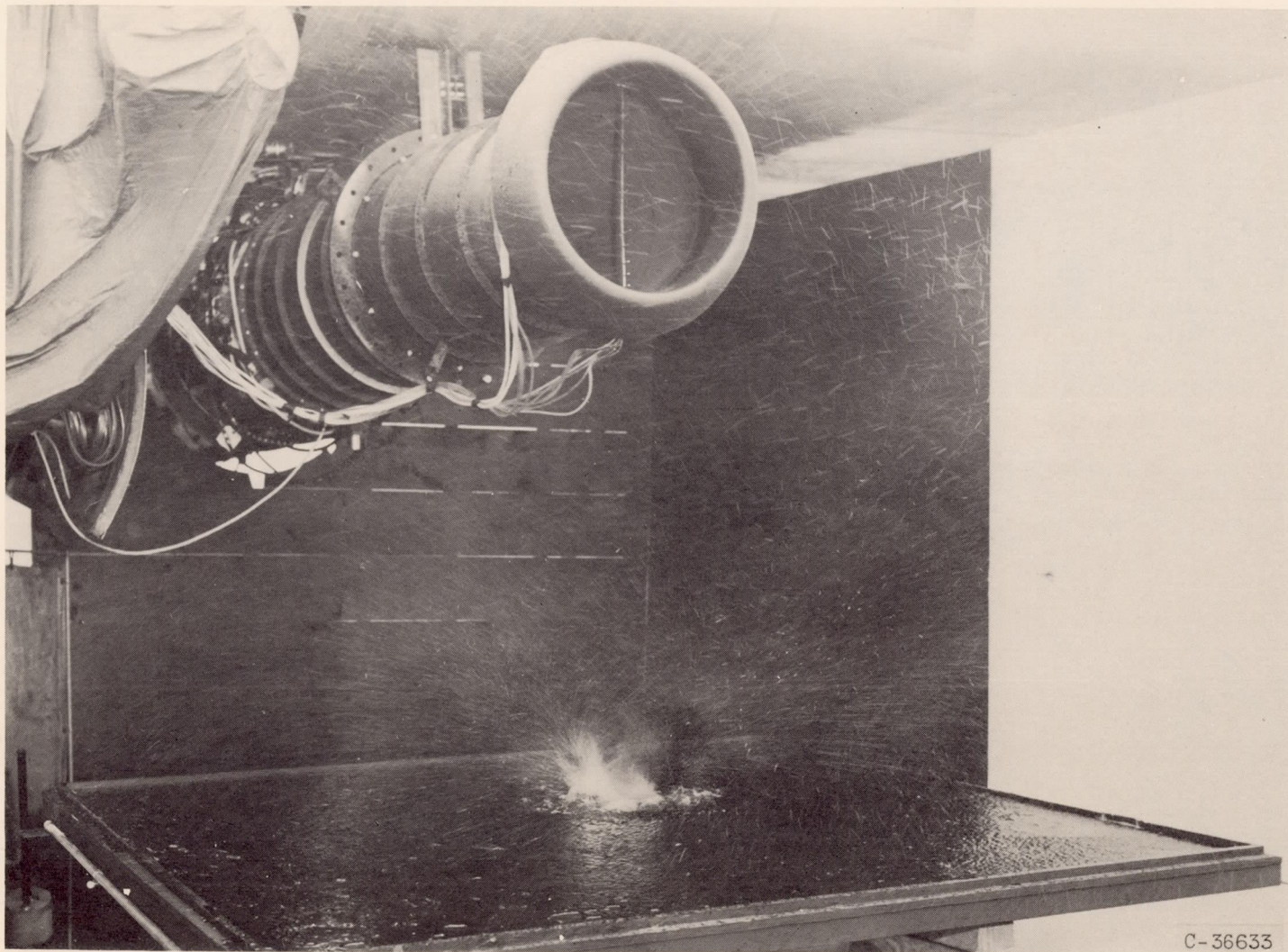
Figure 7. - Water whirl formed by vortex from engine inlet.
