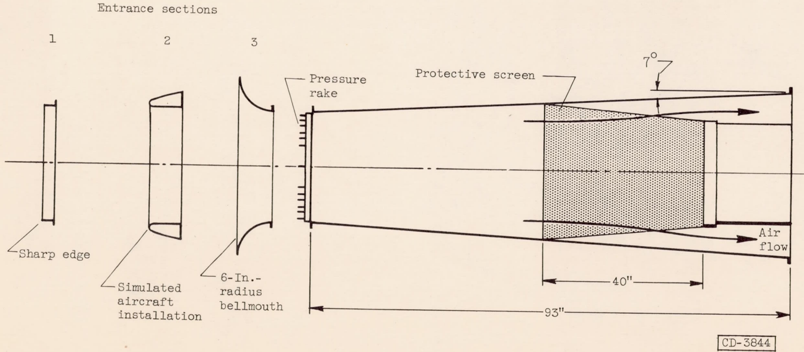
Figure 2. - Air inlet for jet engine.
