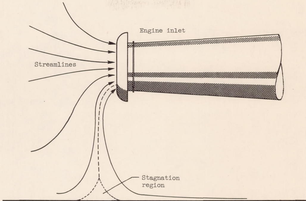
(a), Stagnation region under inlet, low wind velocity.
