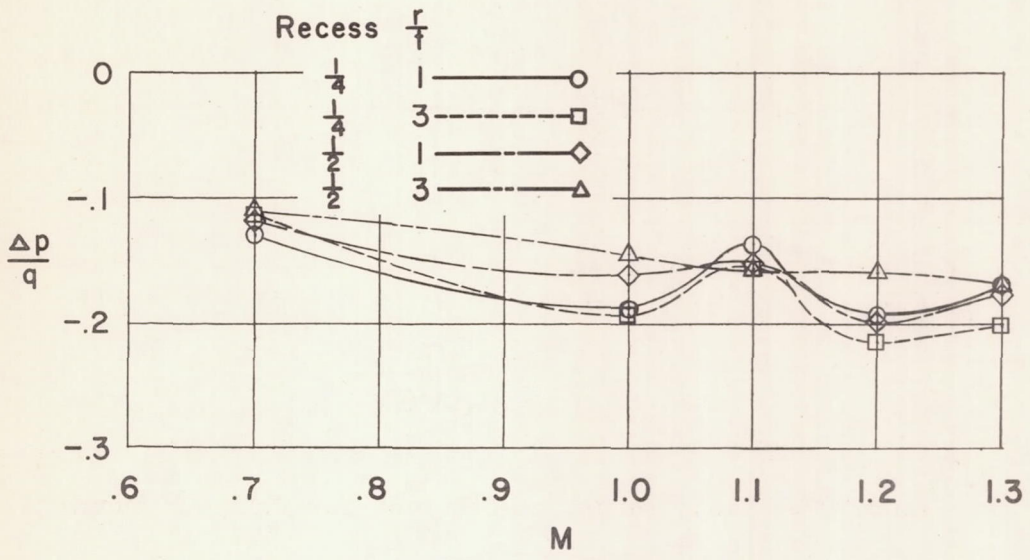
Figure 21.- Vent pressures.
