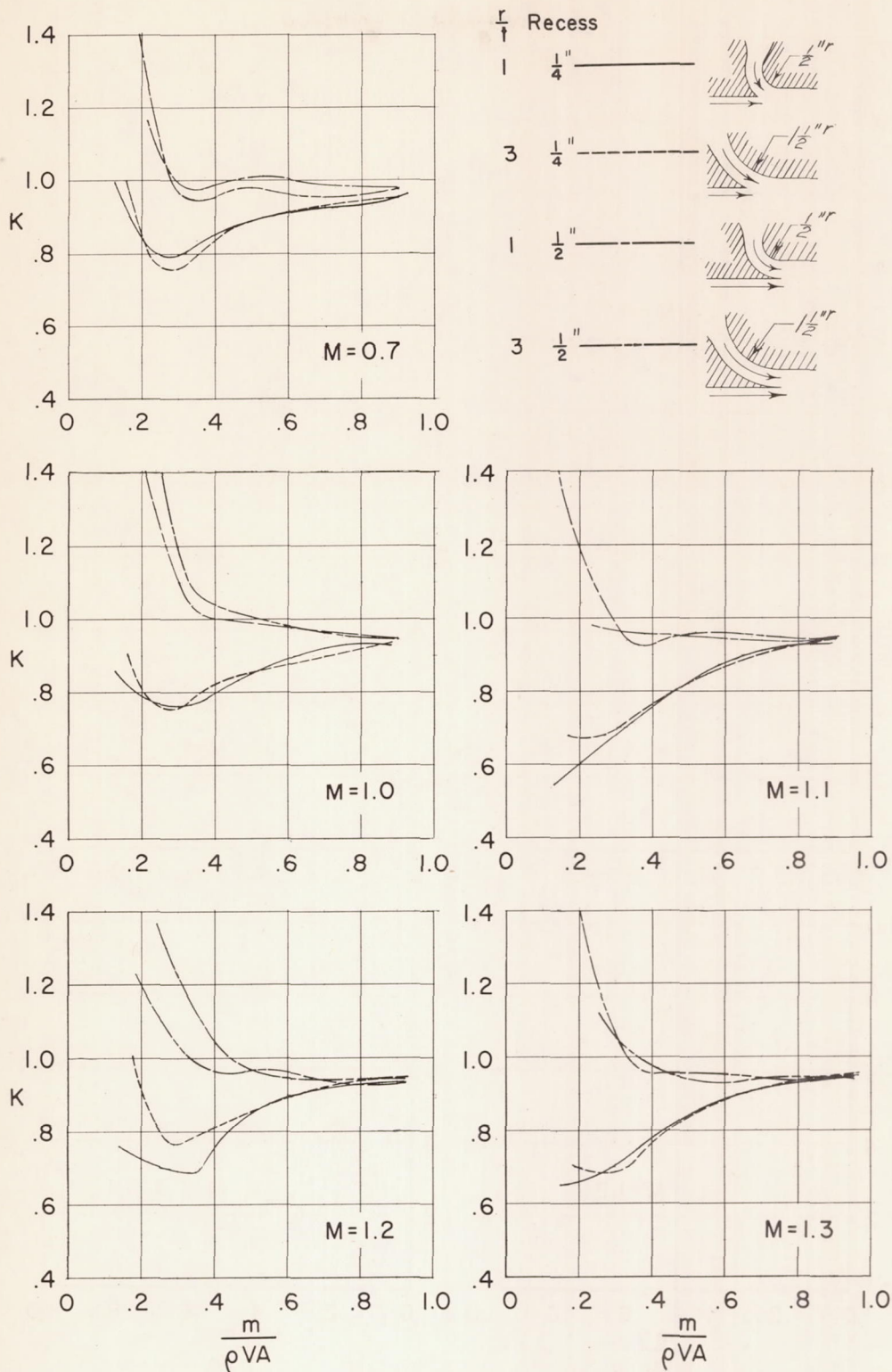
Figure 18.- Discharge coefficient as a function of discharge flow ratio for recessed outlets.
