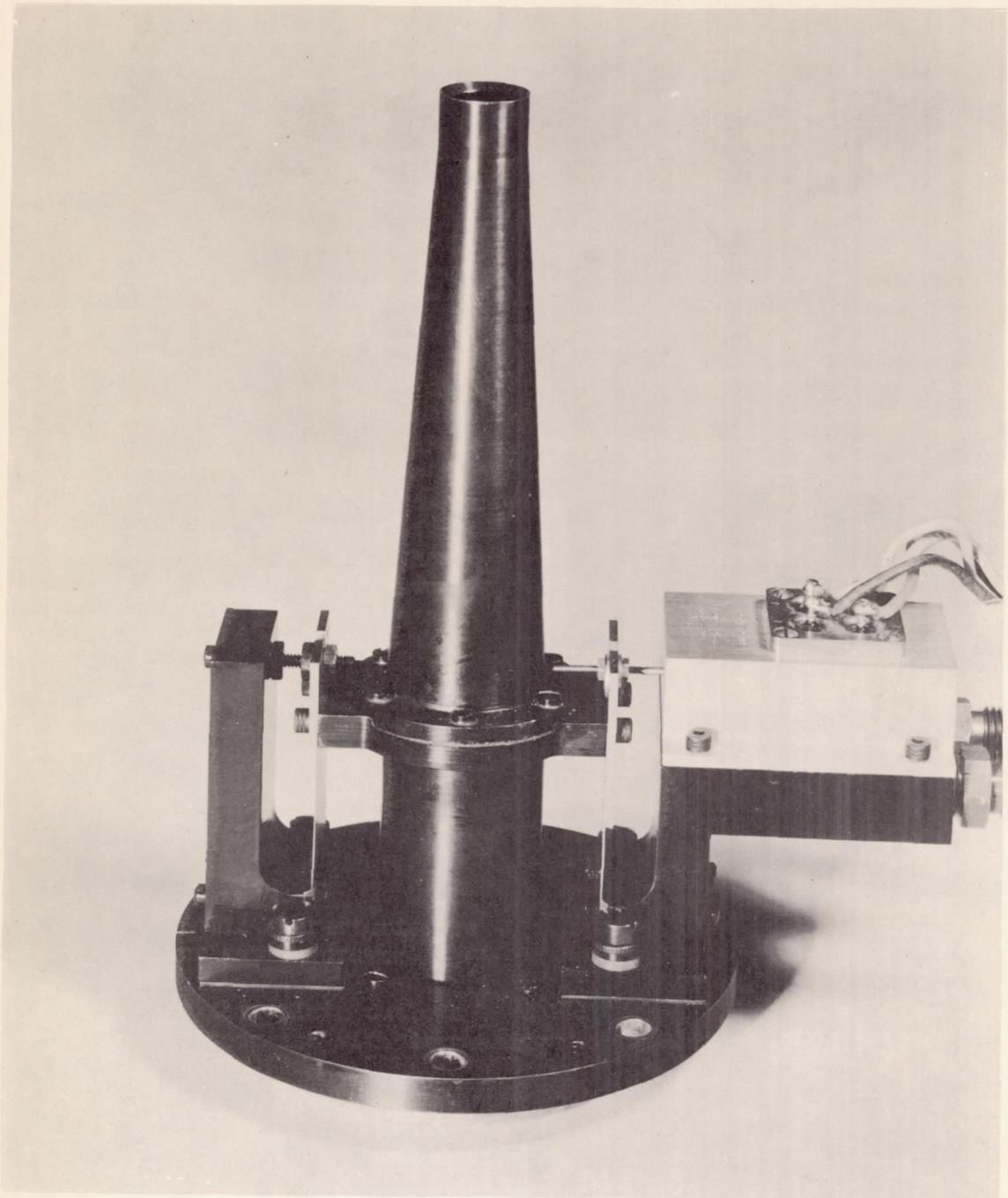
Figure 4.- Balance and approach duct used for force measurements. L-82974
