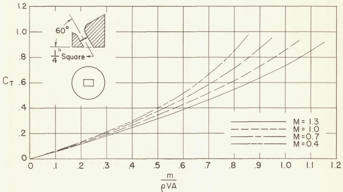
Figure 24.- Thrust coefficients for a square 60^\circ inclined ducted outlet.
