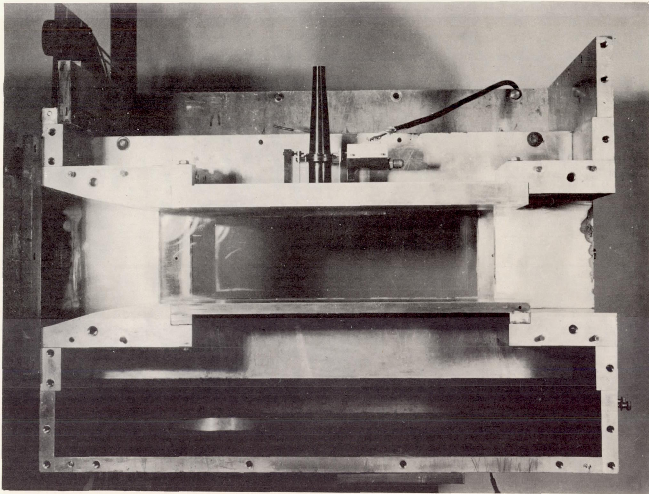
Figure 1.- The 4\frac{1}{2} -inch by 6\frac{1}{4} -inch transonic tunnel with force balance L-82975 in position.
