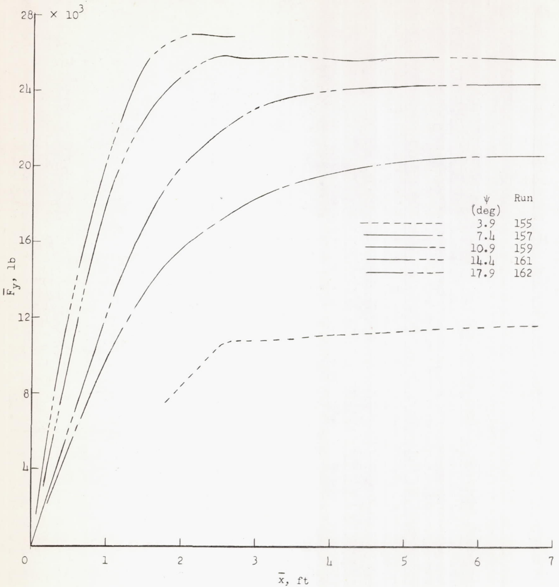
(e) Test series E: \bar{F}_z = 45,200 pounds; \bar{p} \approx 230 pounds per square inch; \bar{\delta}_0 \approx 3.0 inches.
