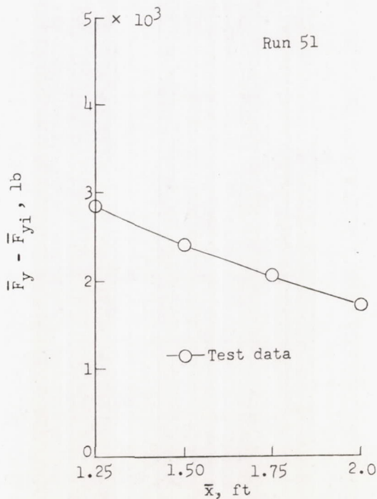
Yawed-rolling method.
