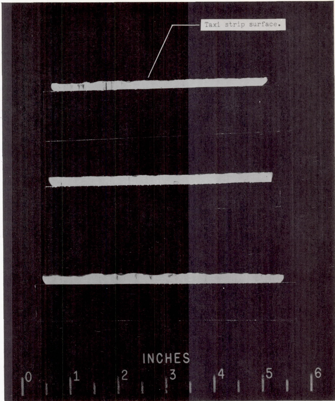
Figure 13.- Representative samples of concrete-taxi-strip surface roughness.
